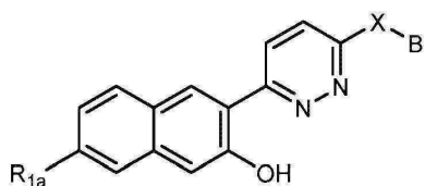
(Ia12)
