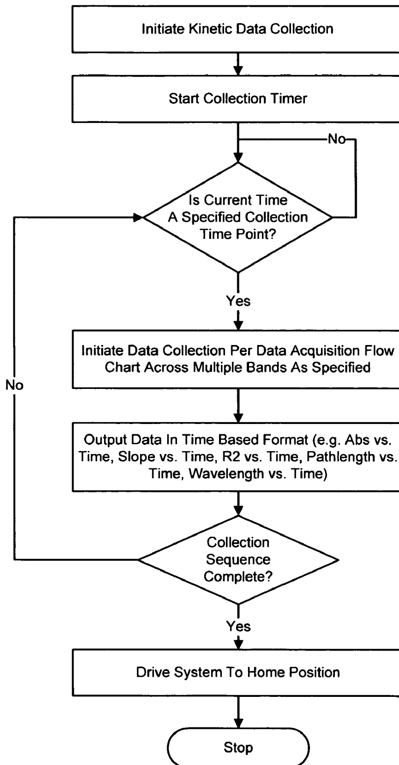
FIG 3 Variable Pathlength Device Software: Kinetic Acquisition
