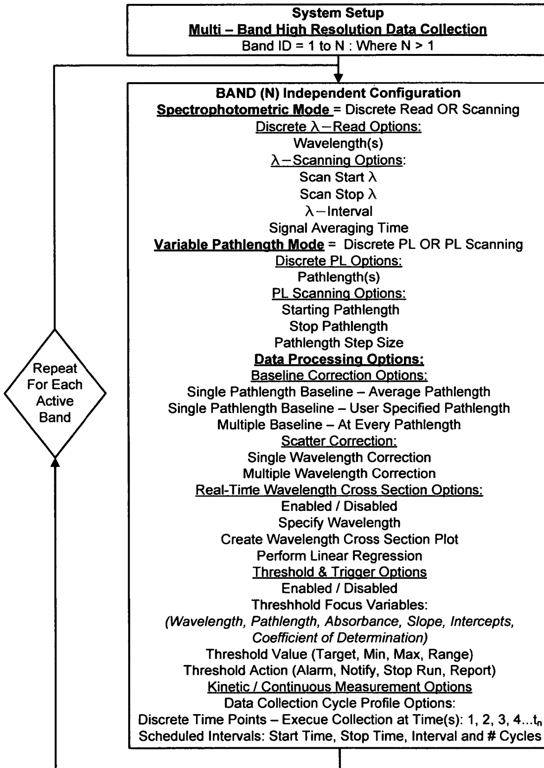
FIG 1 Variable Pathlength Device Software: Setup
