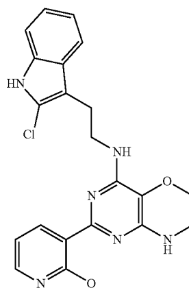
3-(4-((2-(2-chloro-1H-indol-3-yl)ethyl)amino)-7,8-dihydro-6H-pyrimido[5,4-b][1,4]oxazin-2-yl)pyridin-2-ol
