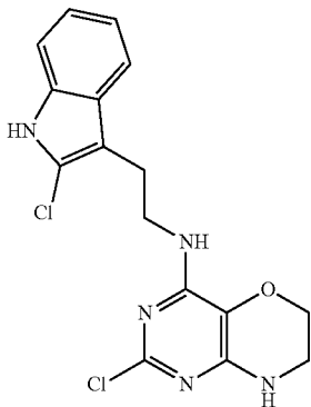
40.3 2-chloro-N-[2-(2-chloro-1H-indol-3-yl)ethyl]-7,8-dihydro-6H-pyrimido[5,4-b][1,4]oxazin-4-amine
