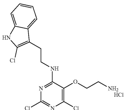
40.2 5-(2-aminoethoxy)-2,6-dichloro-N-[2-(2-chloro-1H-indol-3-yl)ethyl]pyrimidin-4-amine; hydrochloride
