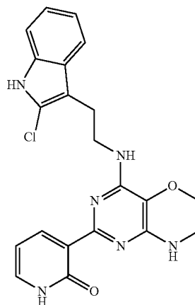
Example 40 3-(4-((2-(2-chloro-1H-indol-3-yl)ethyl)amino)-7,8-dihydro-6H-pyrimido[5,4-b][1,4]oxazin-2-yl)pyridin-2(1H)-one
