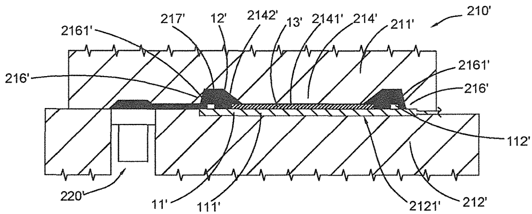
FIG.36B
