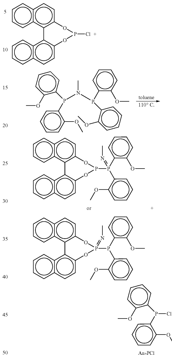
Scheme 1: in situ preparation of ligand composition T'
