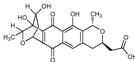
and Derivative 2 (VIII),
