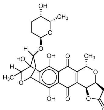
granaticin B (II),
