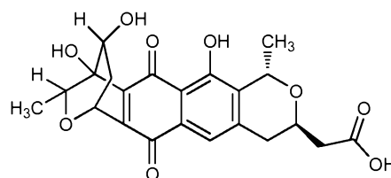
and Derivative 2 (VIII),
