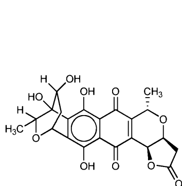
granaticin A (I),
