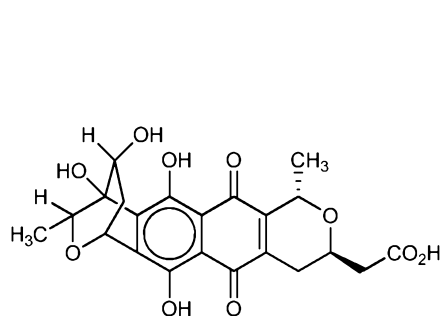
dihydrogranaticin A (III),
