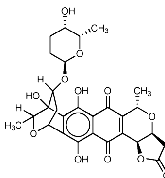
granaticin B (II),
