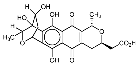
dihydrogranaticin A (III),
