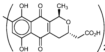
and actinorhodin ( VI ),
