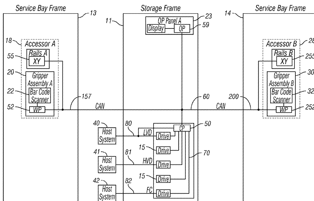
FIG. 3 (Prior Art)
