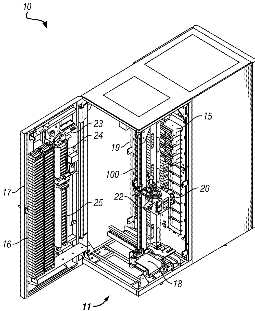
FIG. 2 (Prior Art)
