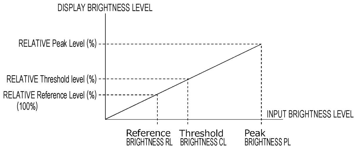
DISPLAY BRIGHTNESS CHARACTERISTIC OF MASTER MONITOR
