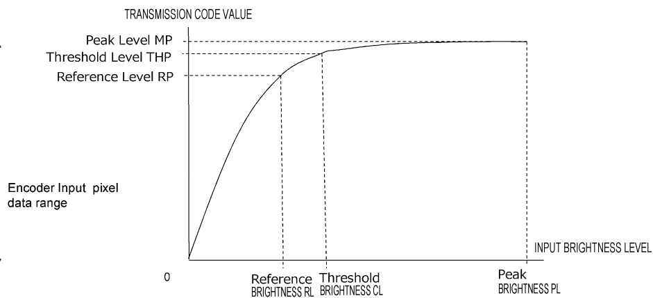
OPTO-ELECTRICAL TRANSFER FUNCTION (OETF)
