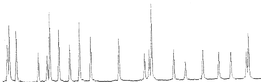
6-FAM-ddCTP 250 pm
