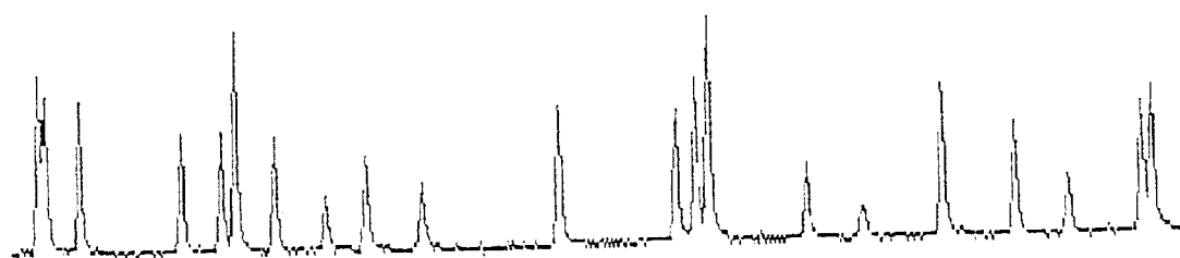
6-FAM-EO-ddCTP 50 pm
