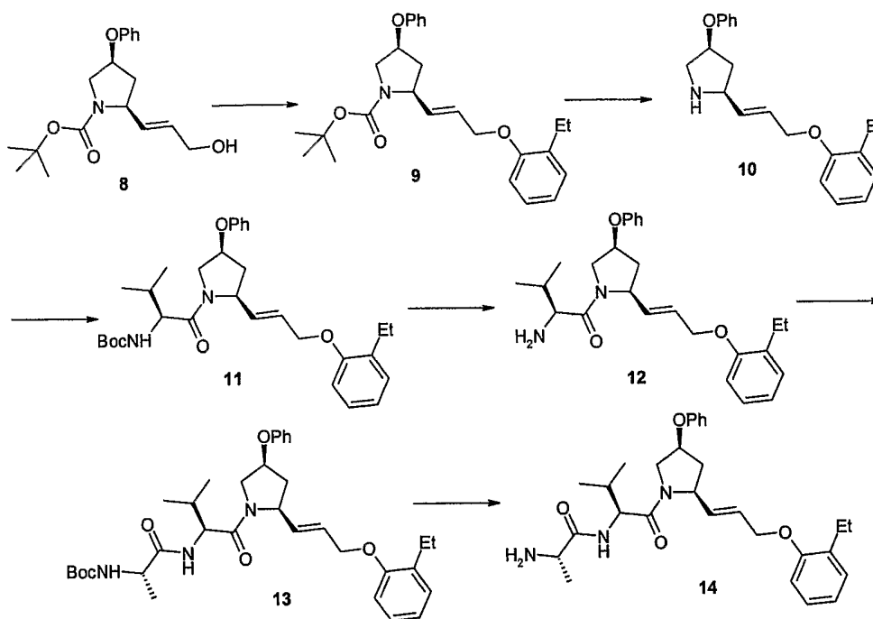
Scheme II
