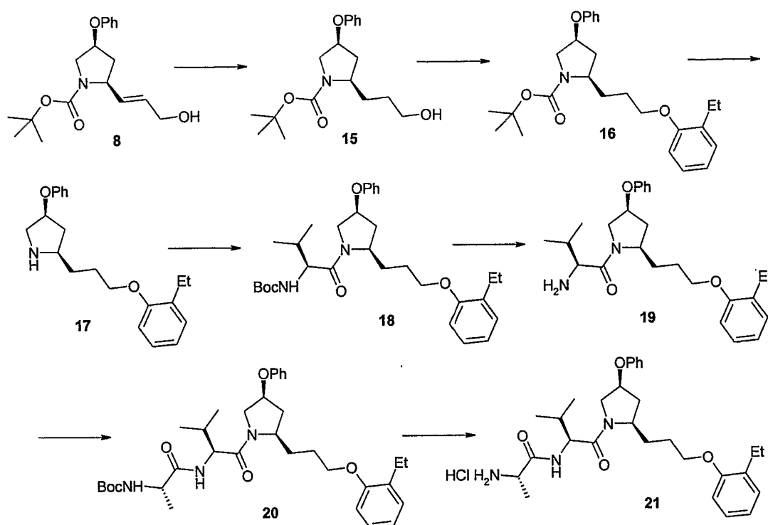
Scheme III
