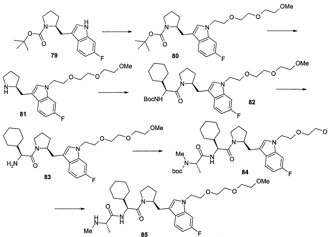
Scheme VIII
