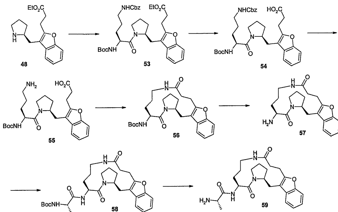
Scheme V(b)
