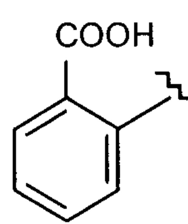
Formula (VIIIc)
