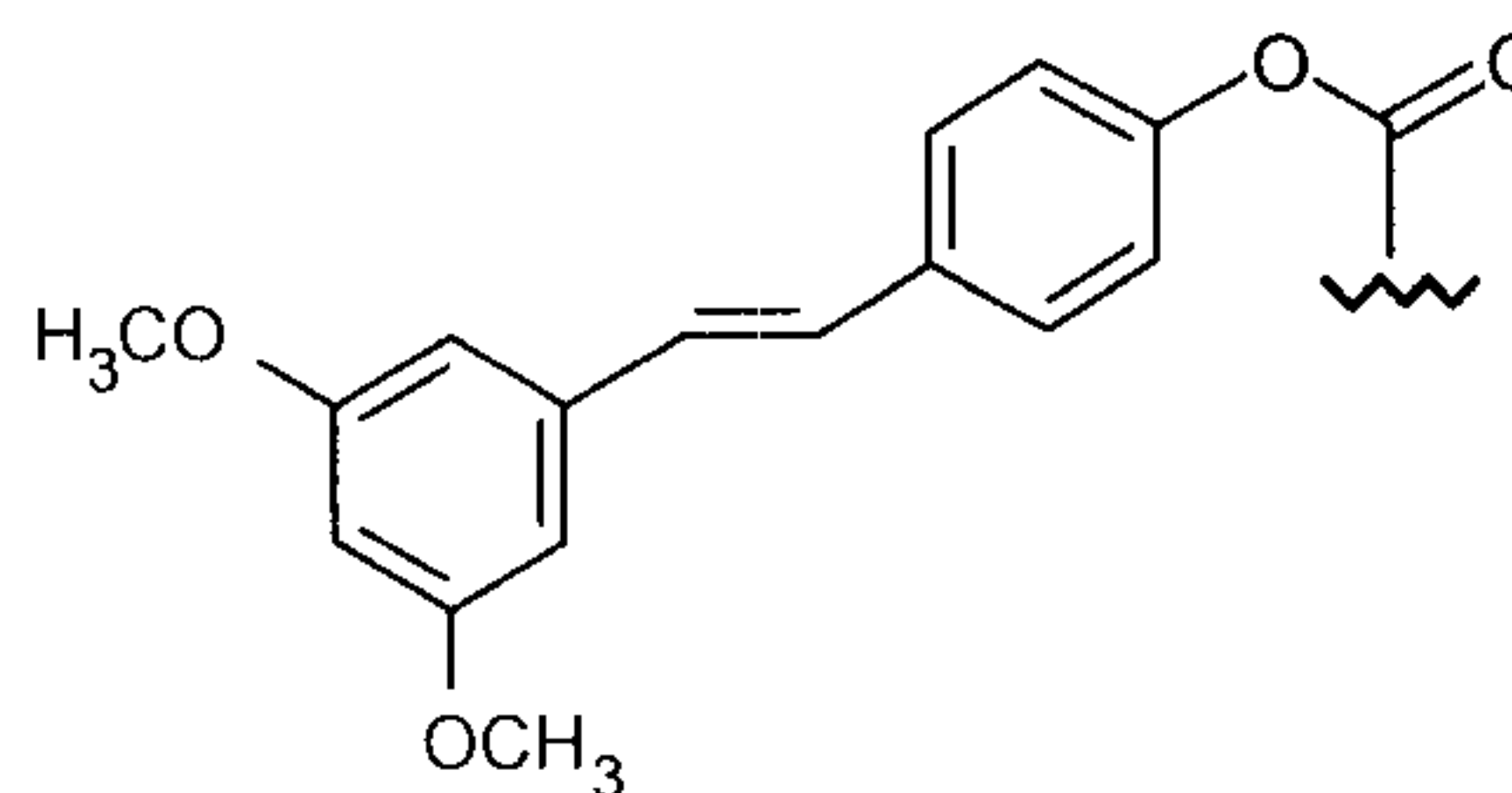
Formula (IXb)
