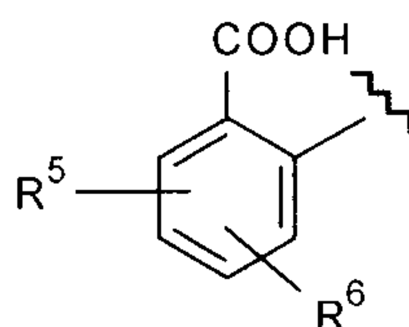
Formula (VIII)
