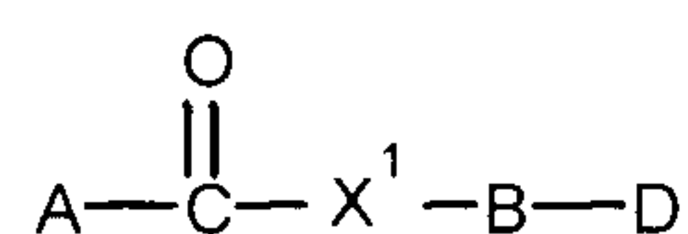
Formula (I)
