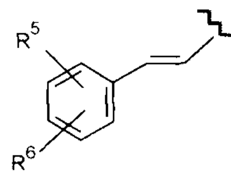
Formula (VII)
