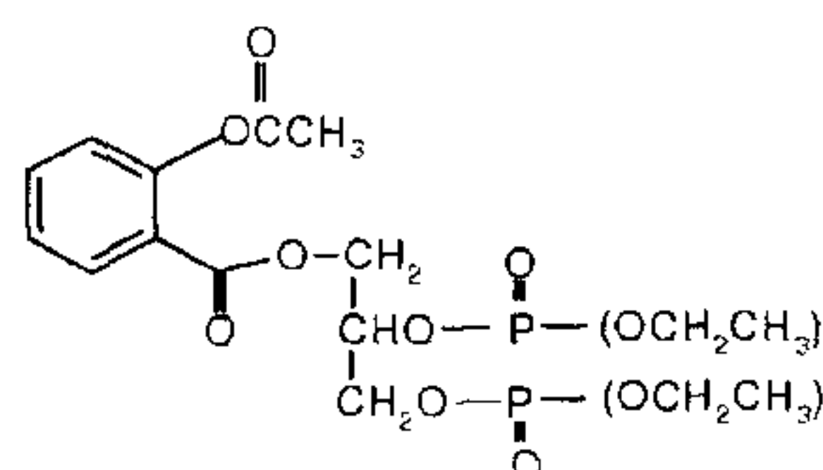
Glycerophospho-aspirin II
