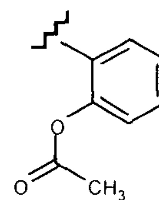
Formula (VI).
