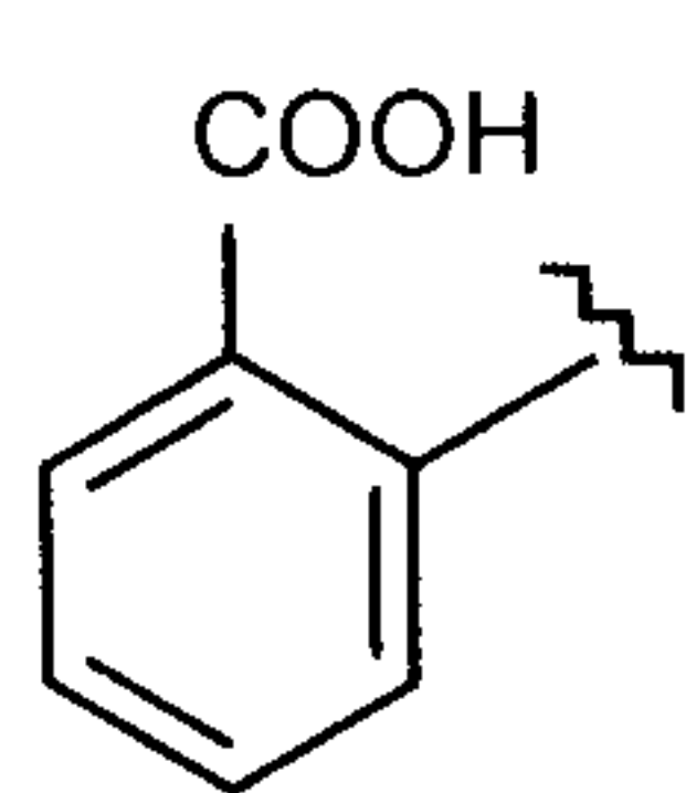
Formula (VIIIa)
