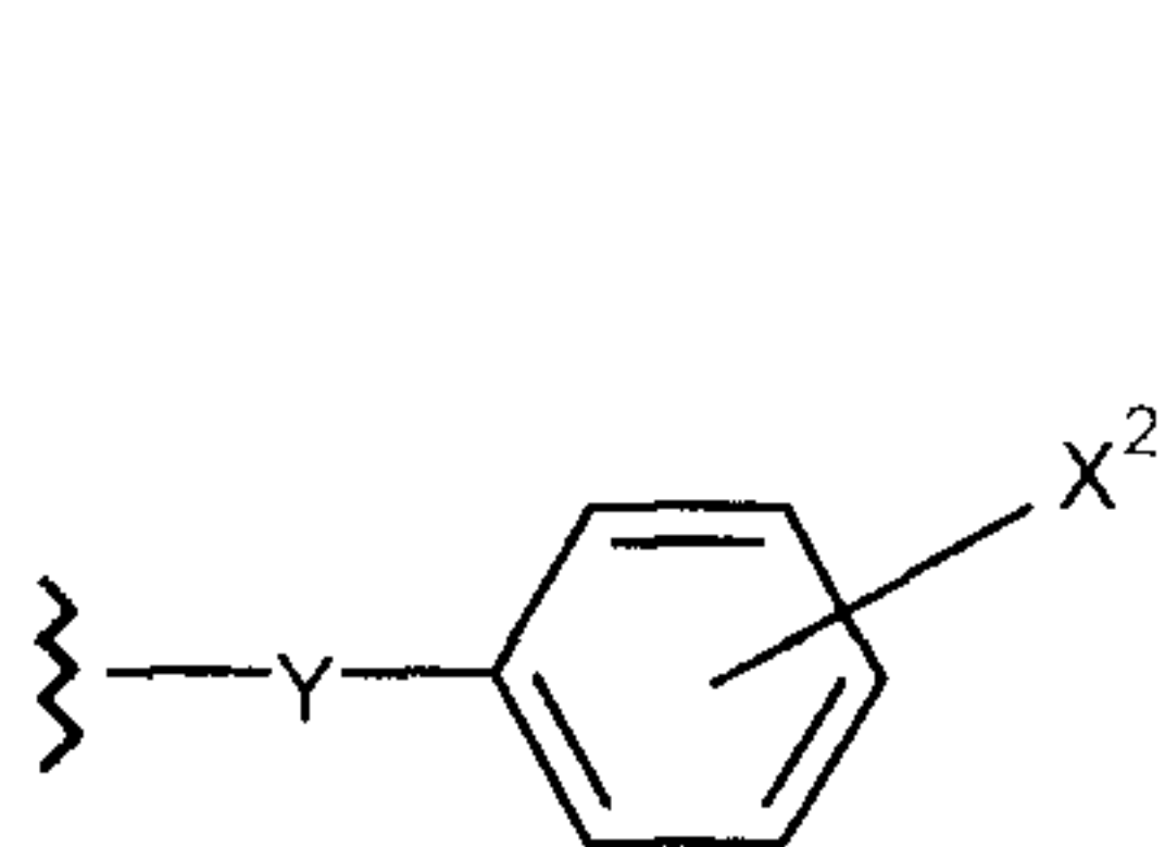
Formula (II)
