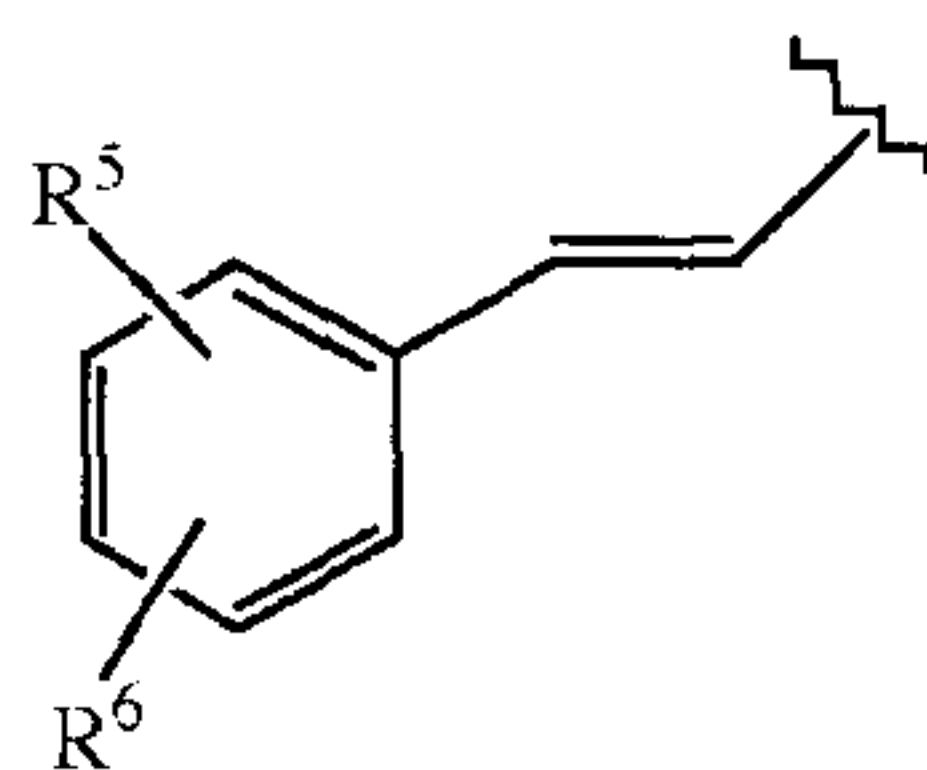
Formula (VII)
