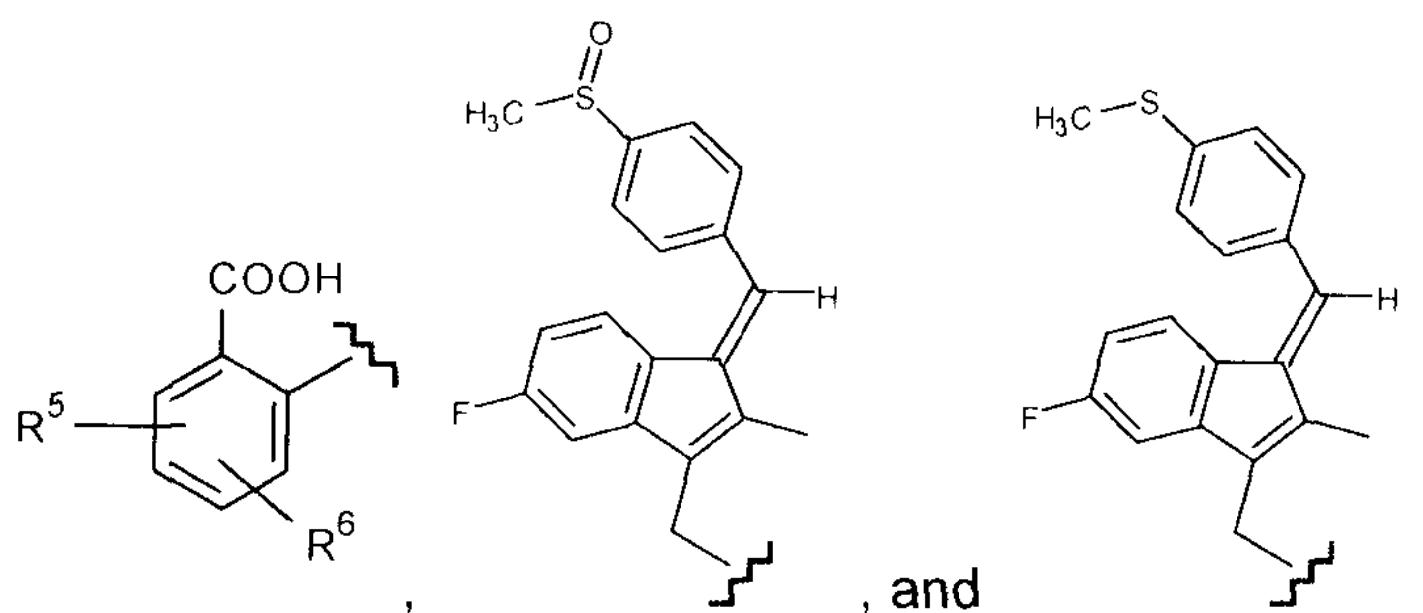
Formula (VIII)
