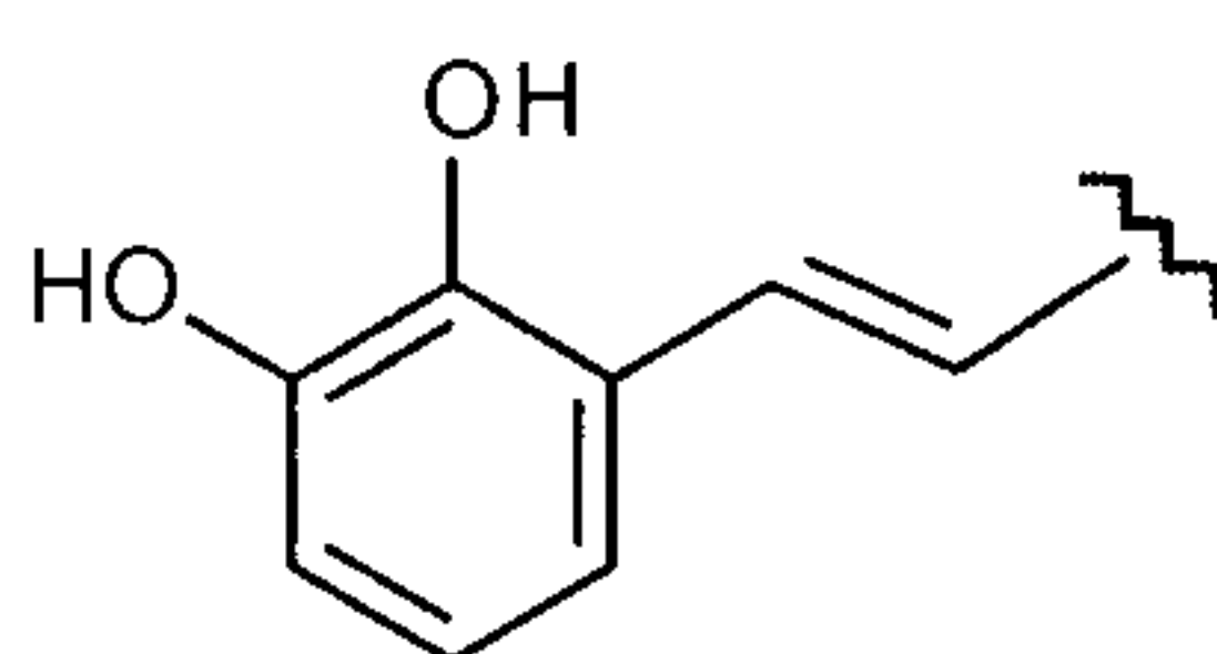
Formula (VIIc)
