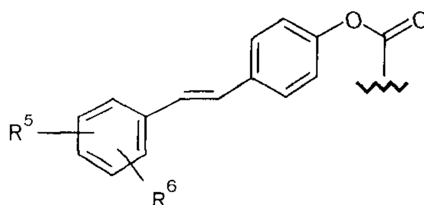
Formula (IX)
