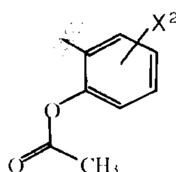
Formula (V)
