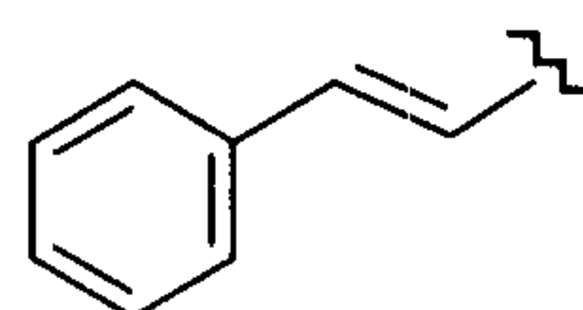
Formula (VIIId)
