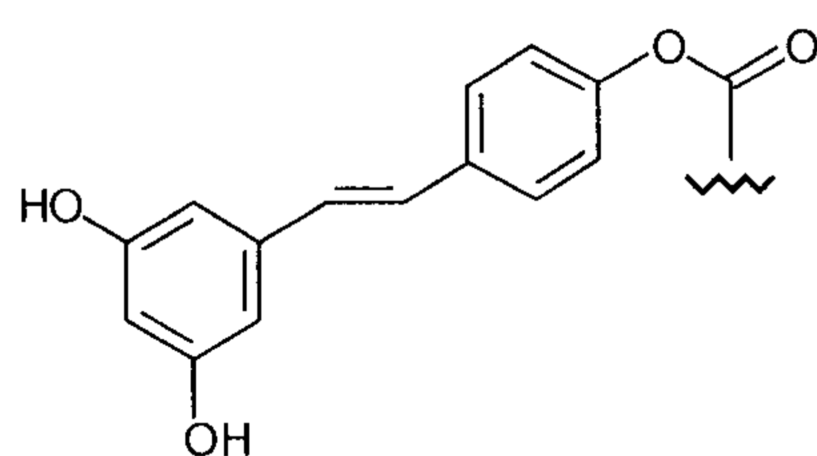
Formula (IXa)
