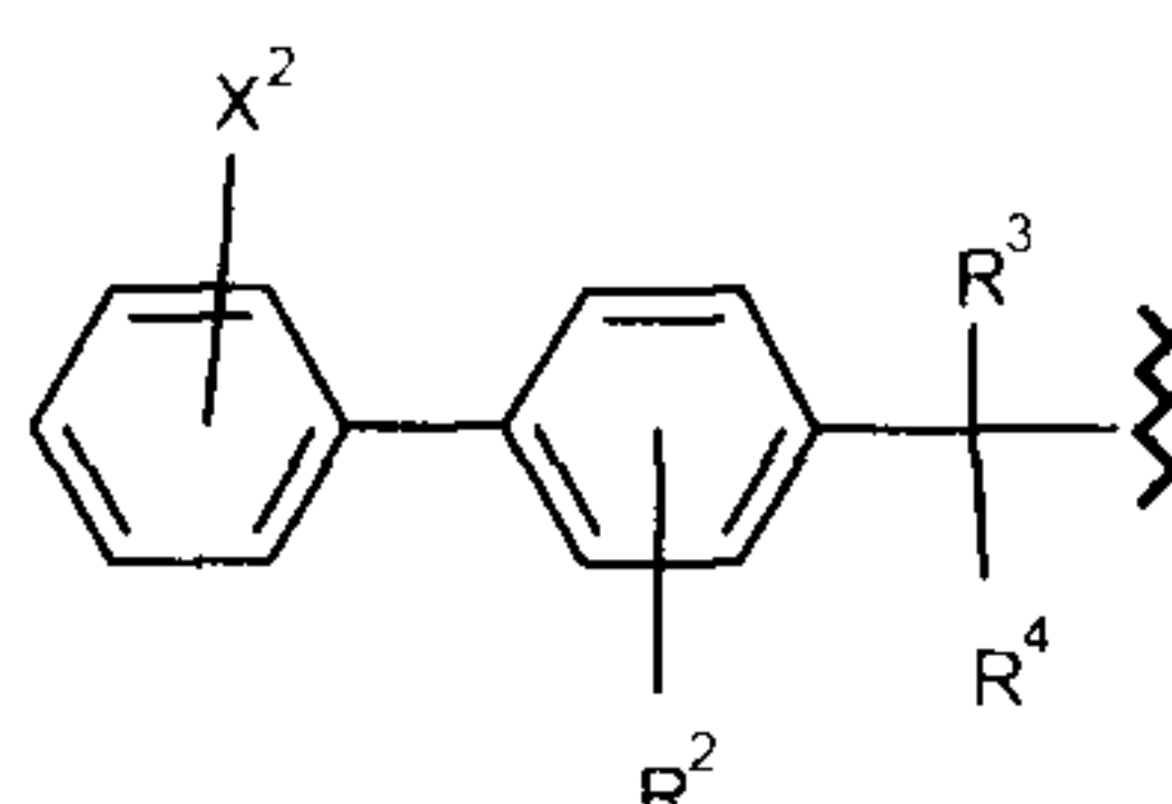
Formula (III)
