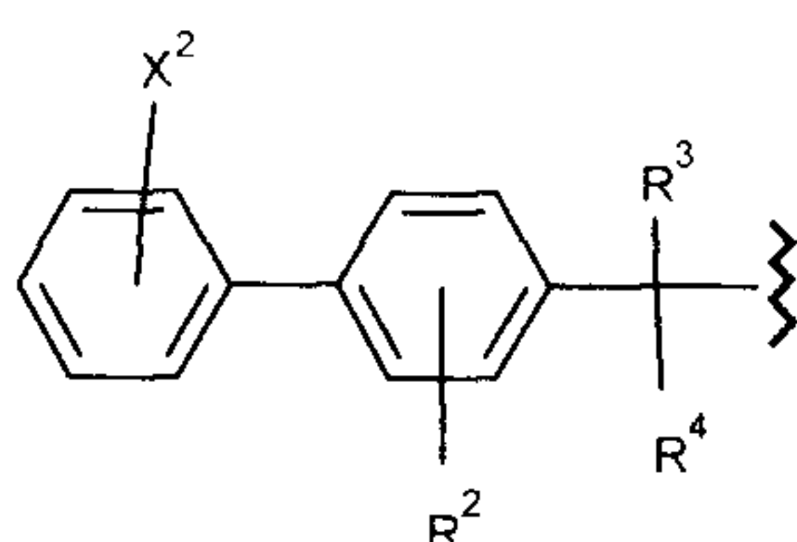
Formula (III)
