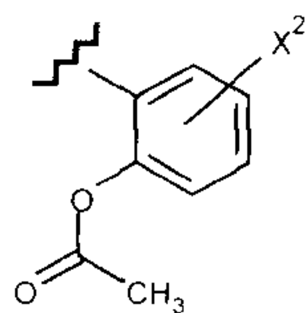
Formula (V)
