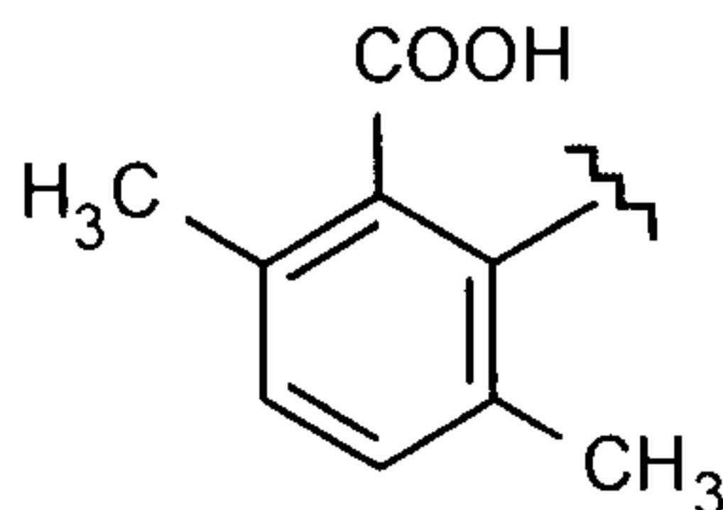
Formula (VIIIb)
