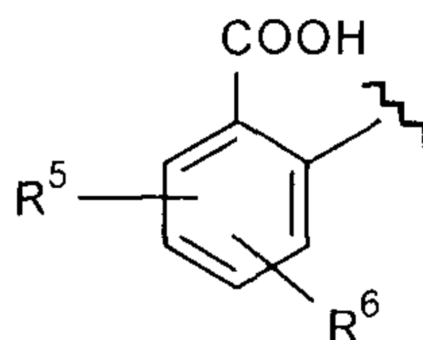
Formula (VIII)
