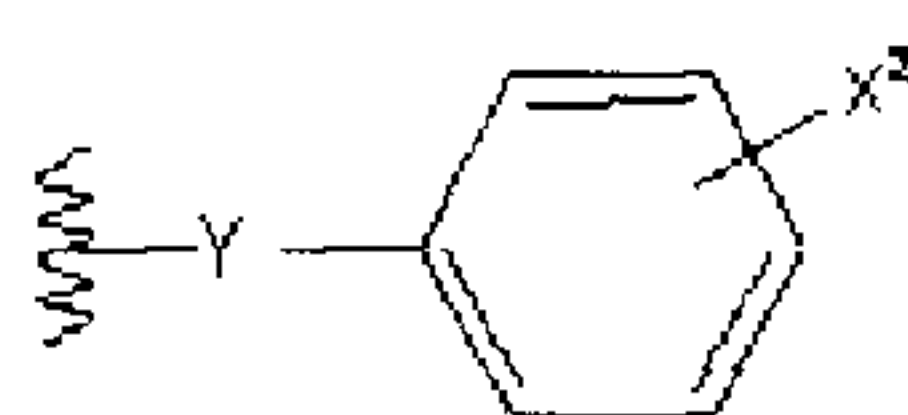
Formula (II)
