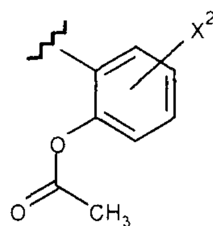
Formula (V)
