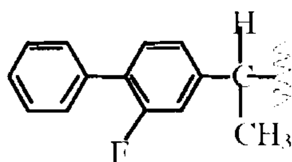
Formula (IV).
