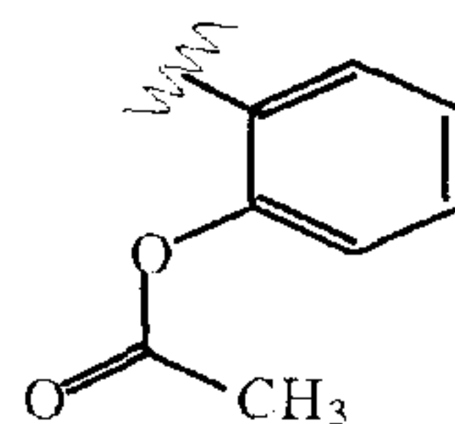
Formula (VI).
