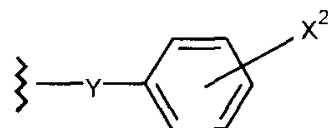
Formula (II)
