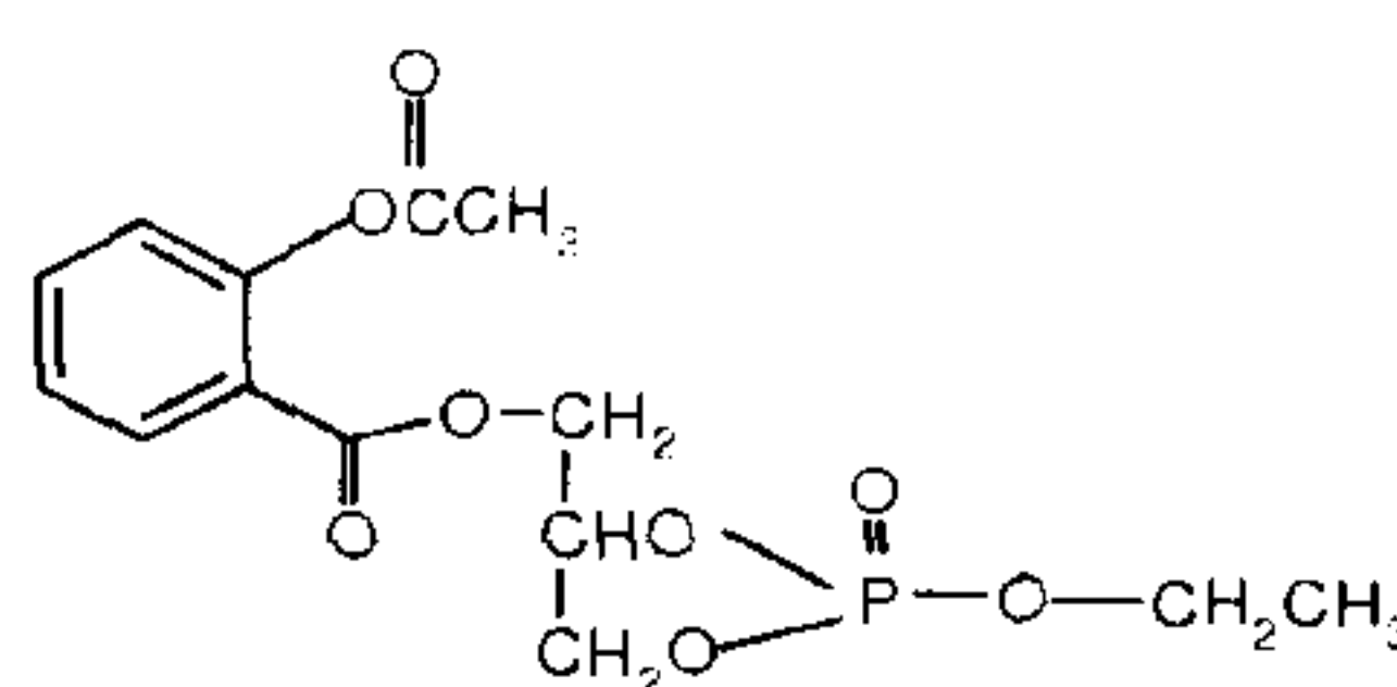
Glycerophospho-aspirin I
