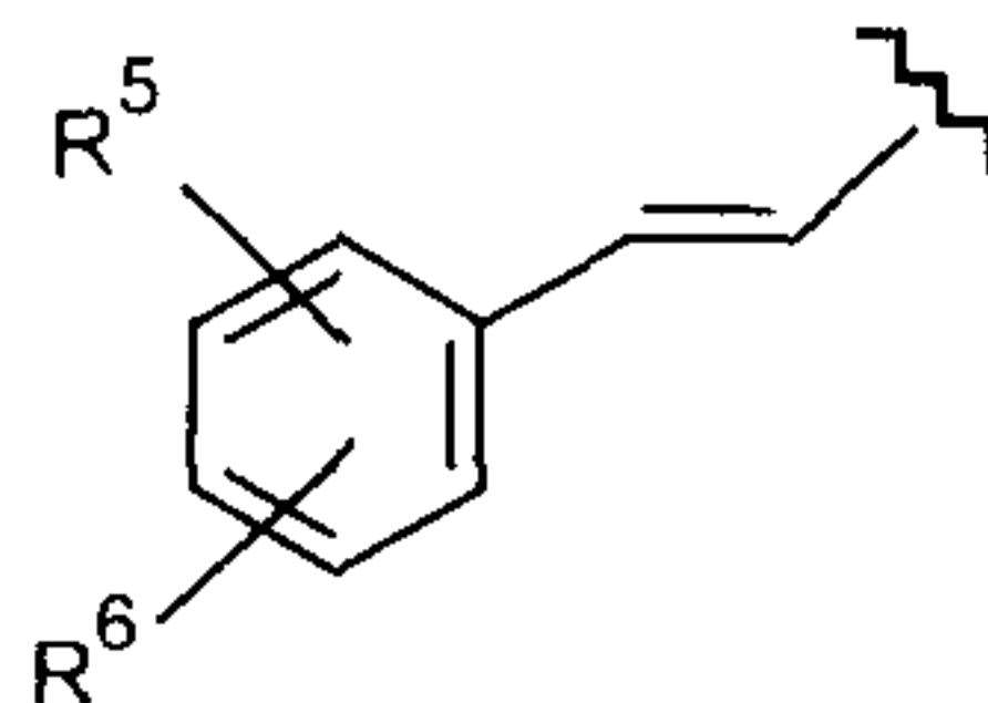
Formula (VII)
