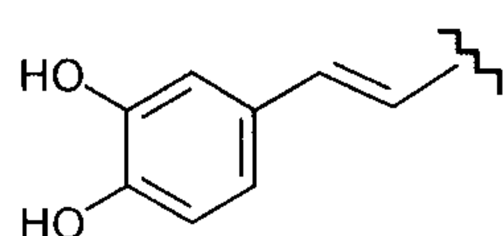
Formula (VIIa)
