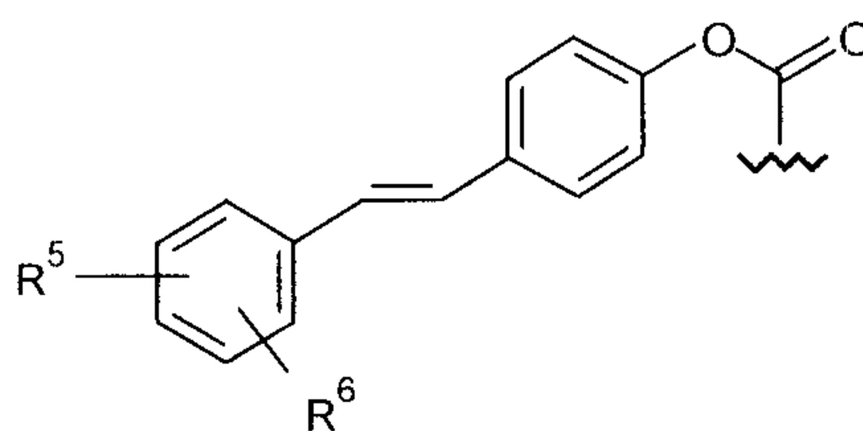
Formula (IX)
