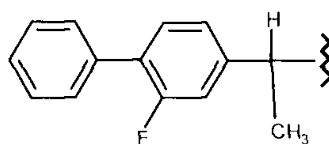
Formula (IV).
