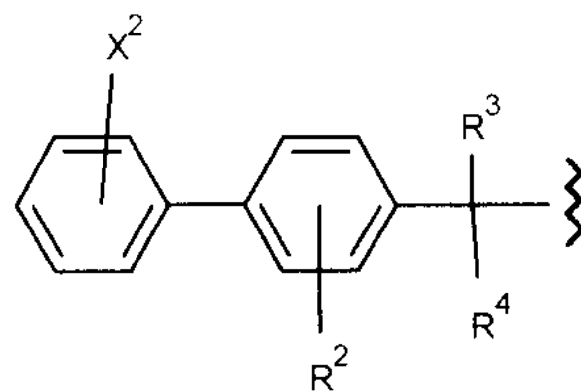
Formula (III)
