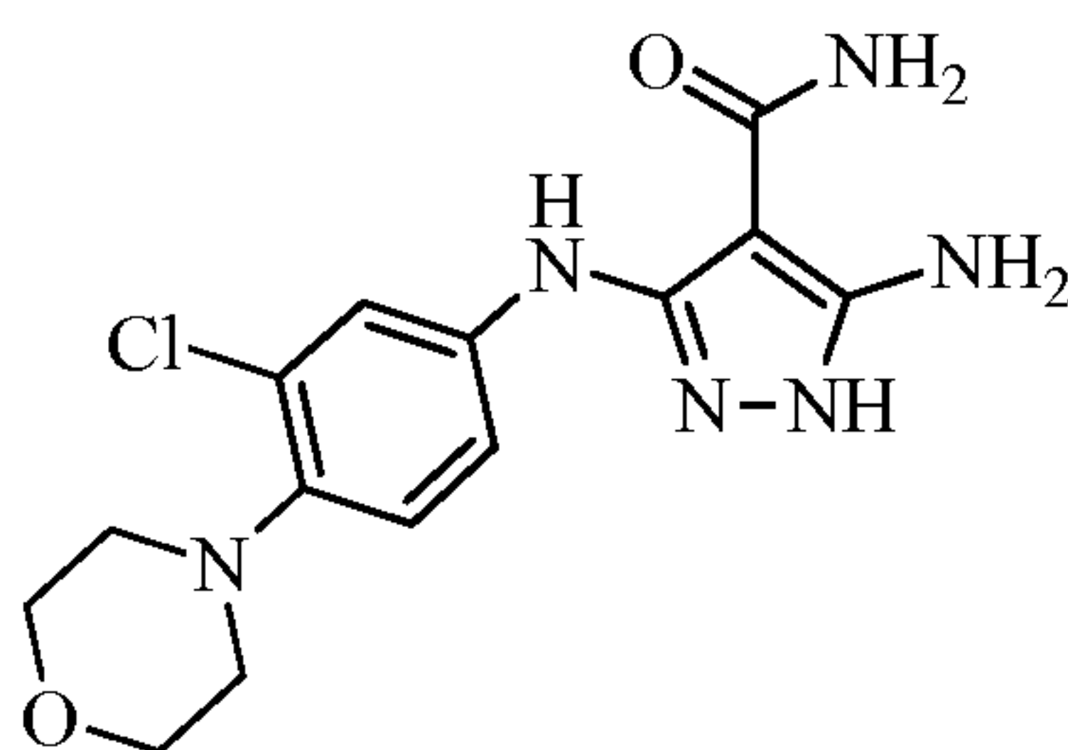
5-amino-3-((3-chloro-4-morpholinophenyl)amino)-1H-pyrazole-4-carboxamide
