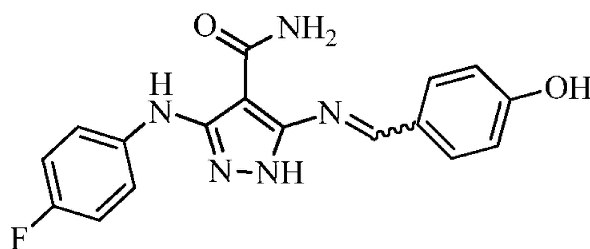
3-((4-fluorophenyl)amino)-5-((4-hydroxybenzylidene)amino)-1 H -pyrazole-4-carboxamide
