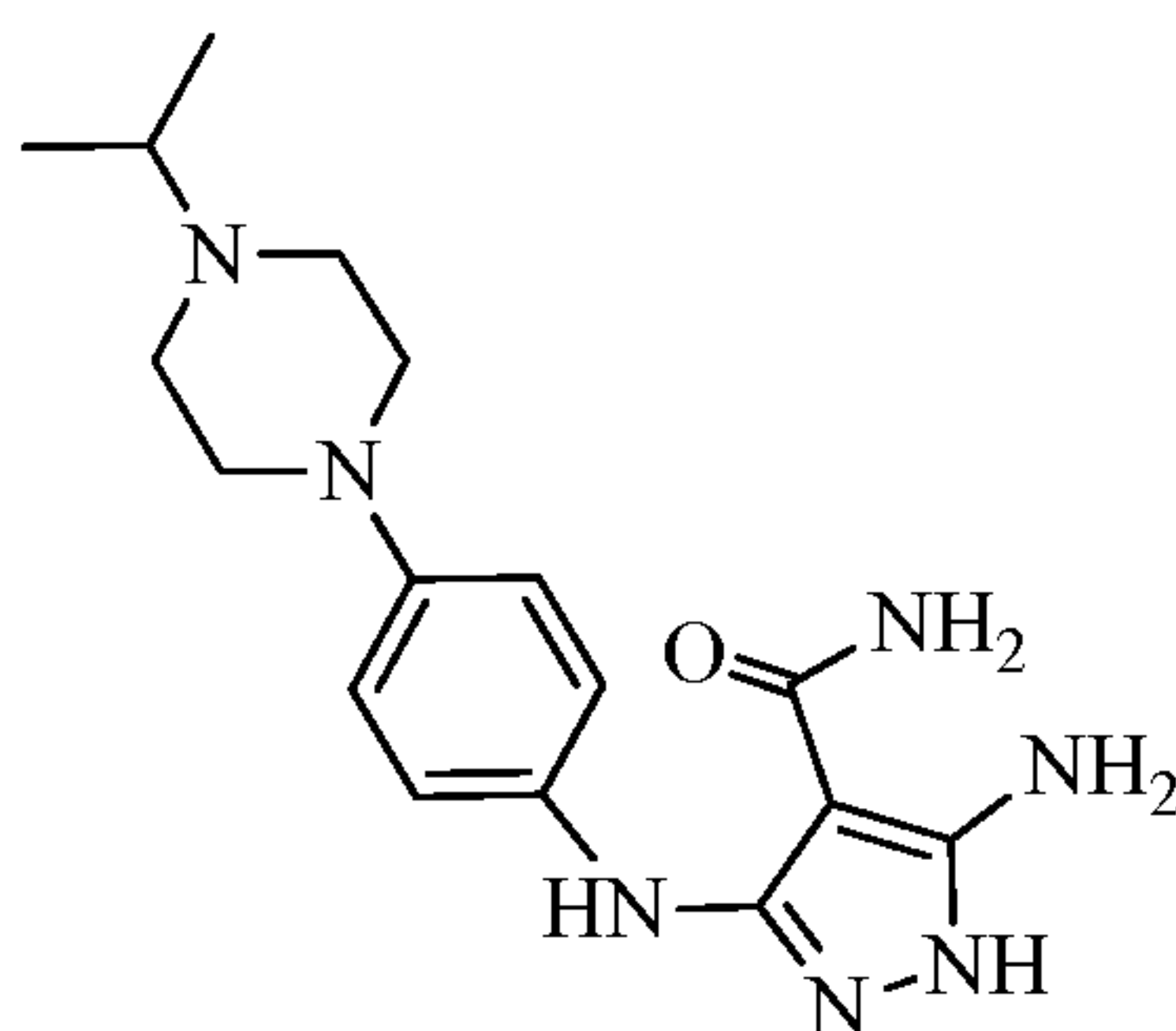
5-amino-3-((4-(4-isopropylpiperazin-1-yl)phenyl)amino)-1 H -pyrazole-4-carboxamide
