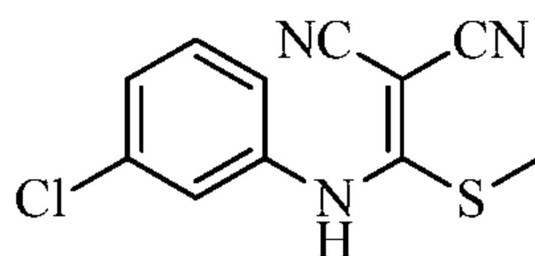
2-(((3-chlorophenyl)amino)(methylthio)methylene)malononitrile
