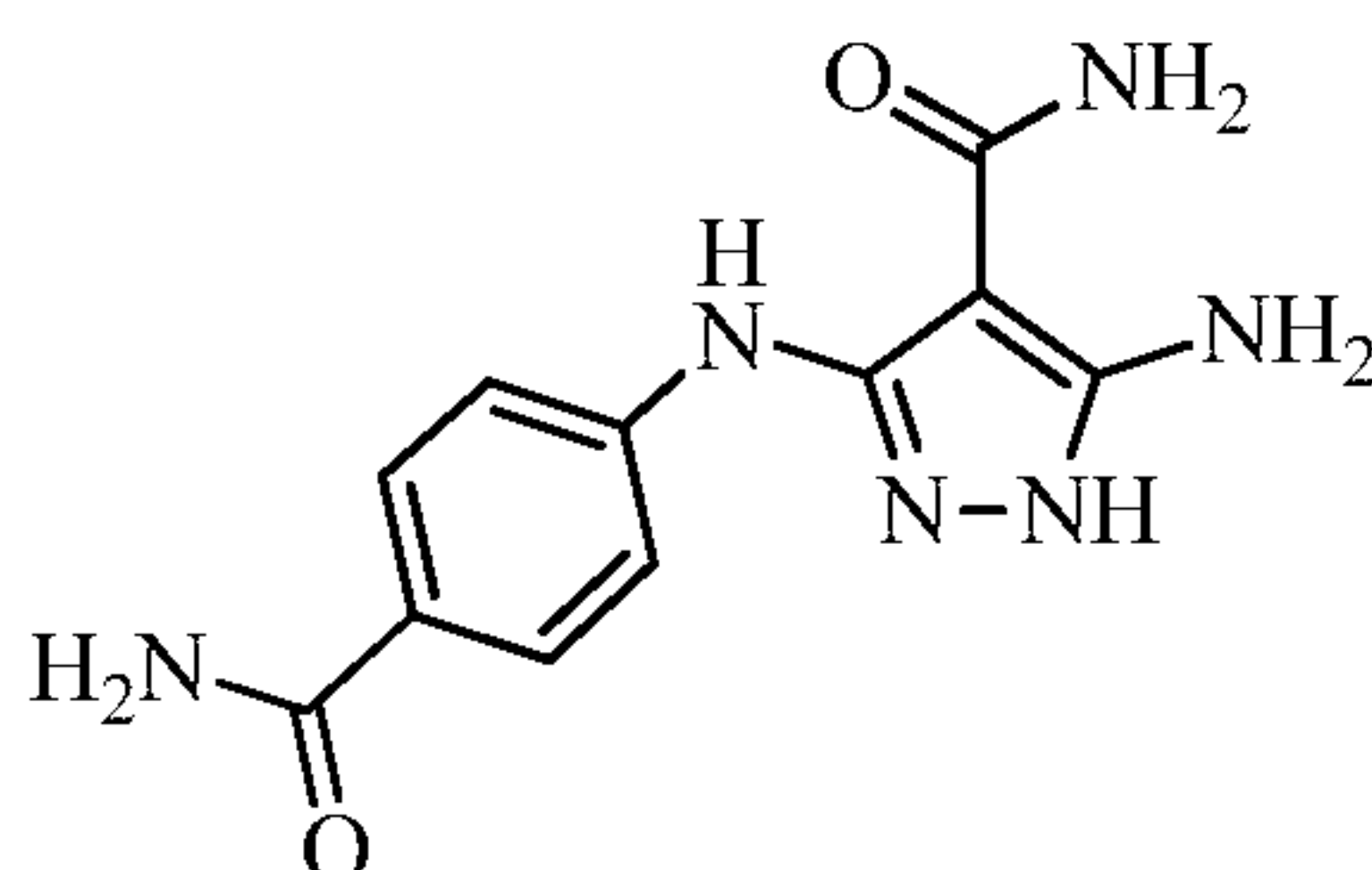
5-amino-3-((4-carbamoylphenyl)amino)-1 H -pyrazole-4-carboxamide
