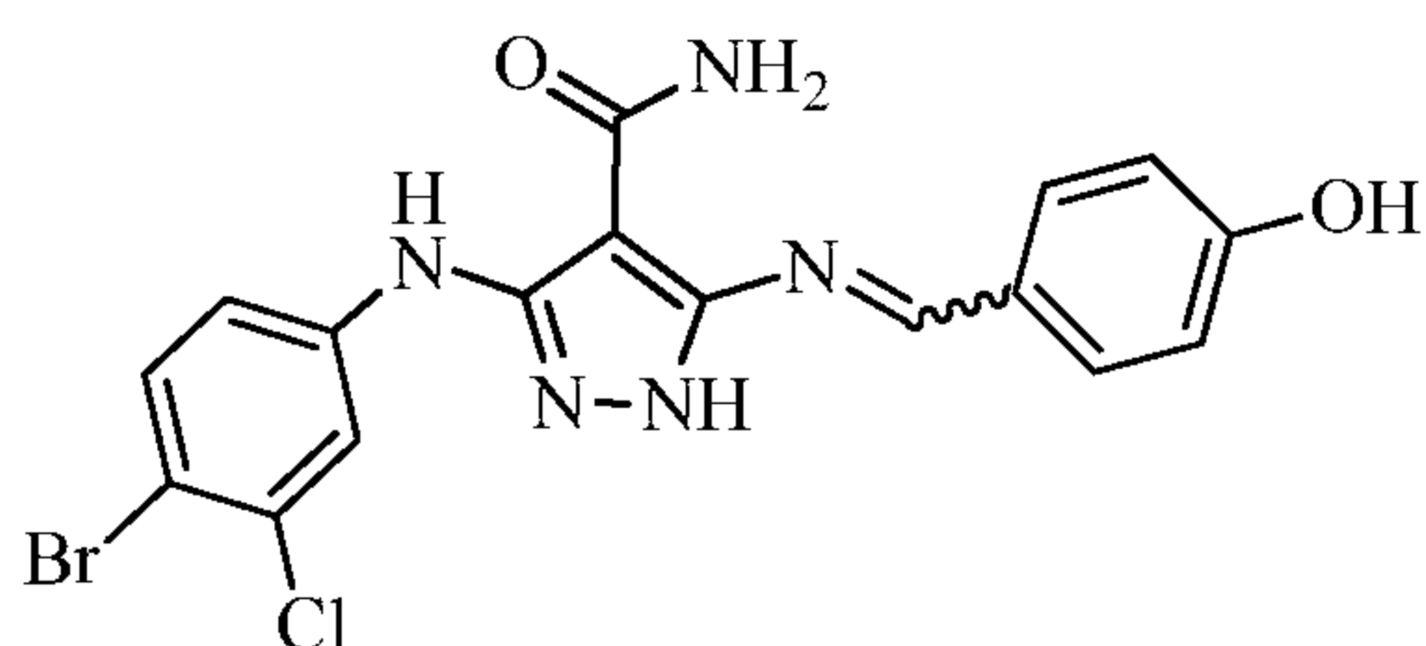
3-((4-bromo-3-chlorophenyl)amino)-5-((4-hydroxybenzylidene)amino)-1 H -pyrazole-4-carboxamide
