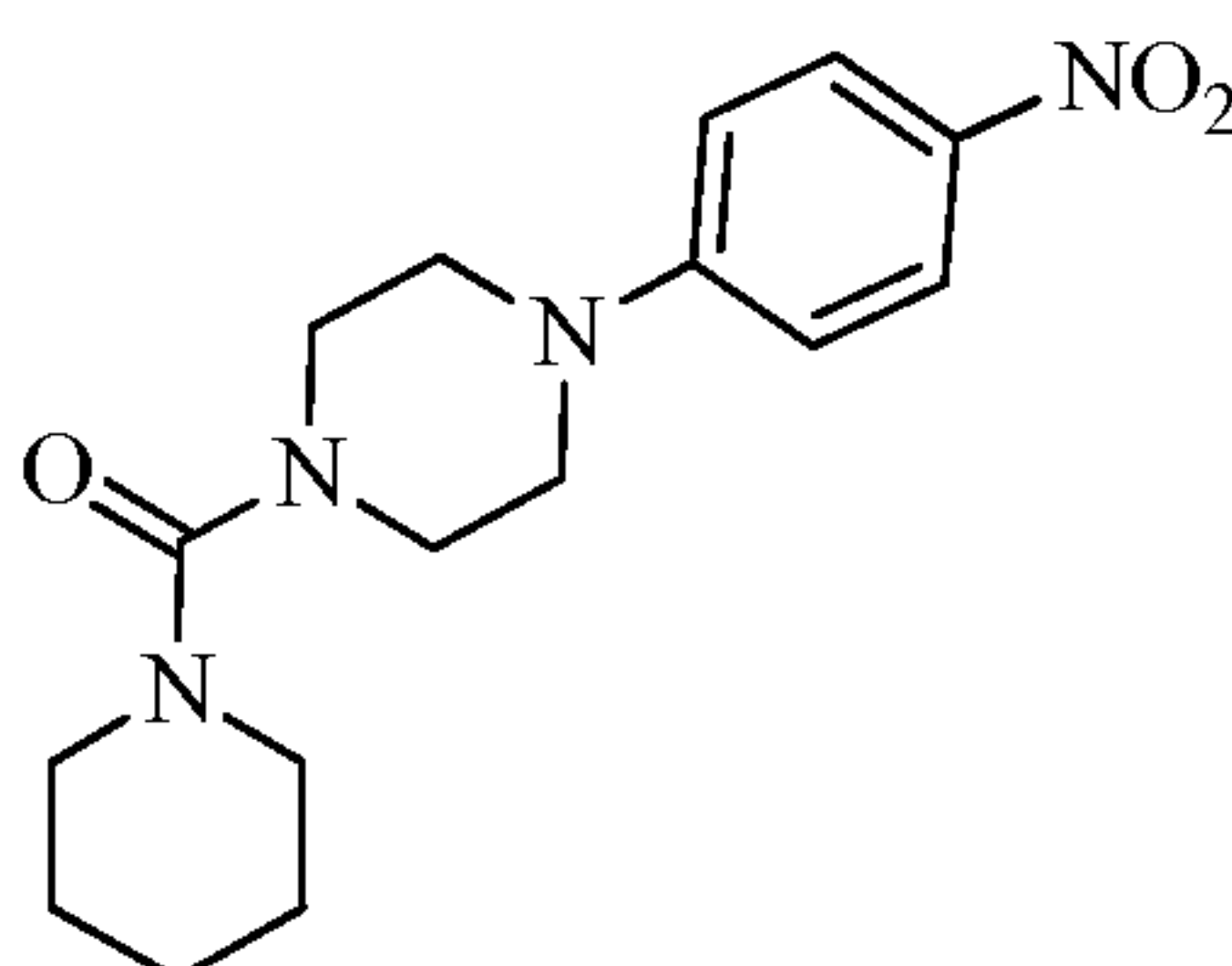
(4-(4-nitrophenyl)piperazin-1-yl)(piperidin-1-yl)methanone
