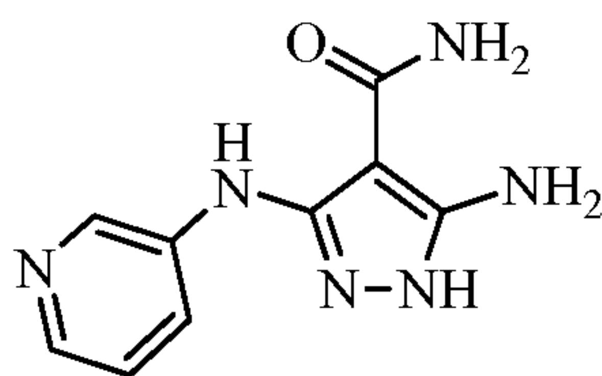
5-amino-3-(pyridin-3-ylamino)-1 H -pyrazole-4-carboxamide
