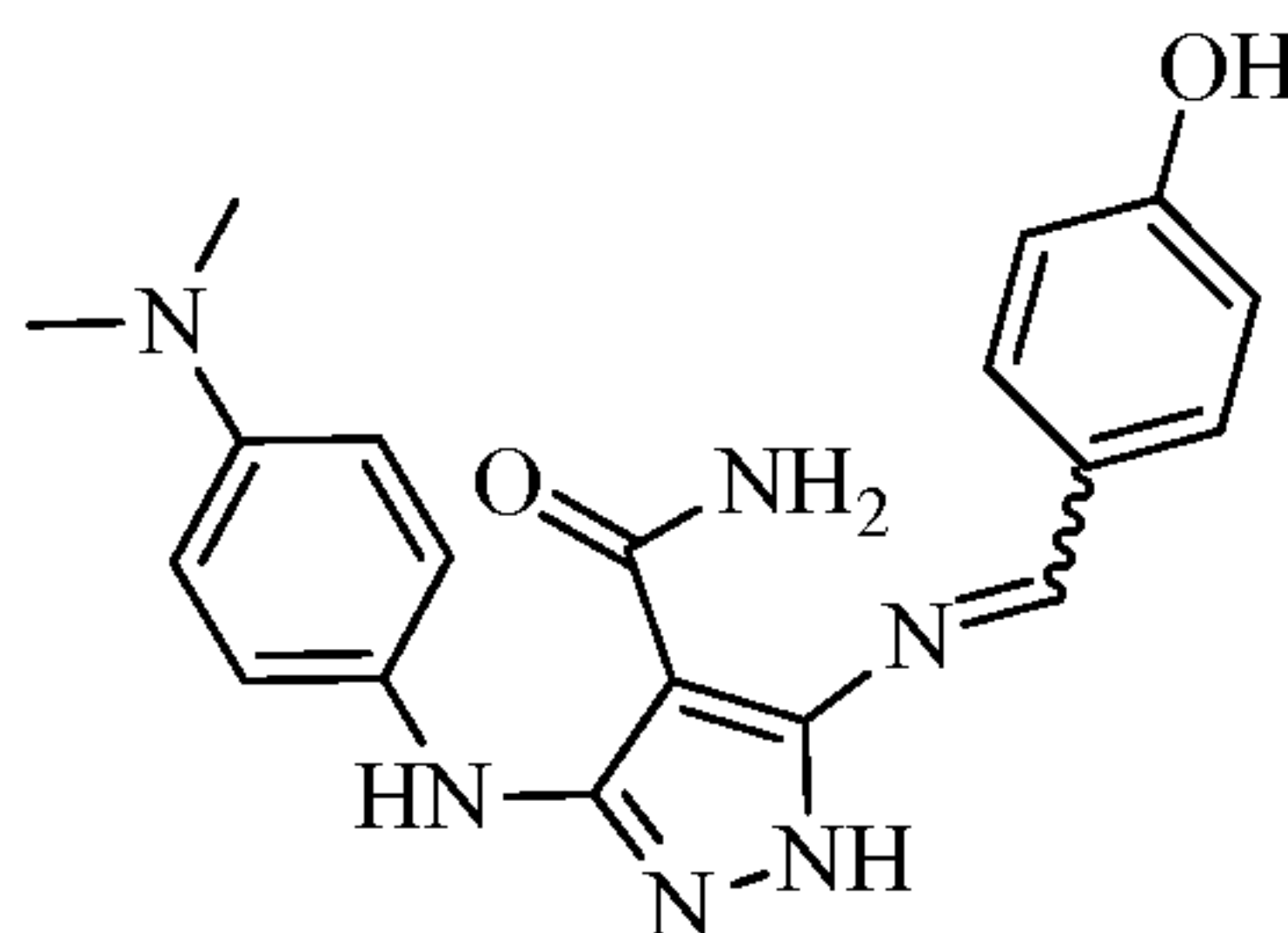
3-((4-(dimethylamino)phenyl)amino)-5-((4-hydroxybenzylidene)amino)-1 H -pyrazole-4-carboxamide
