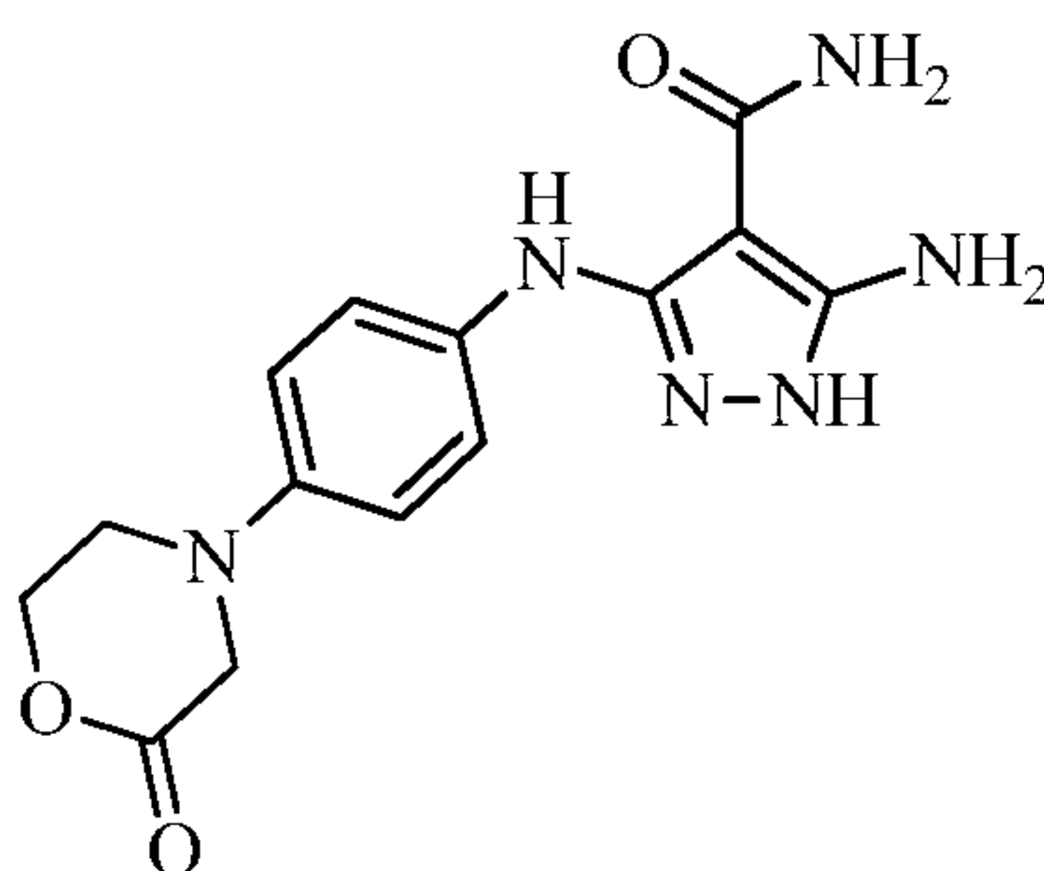
5-amino-3-((4-(2-oxomorpholino)phenyl)amino)-1H-pyrazole-4-carboxamide
