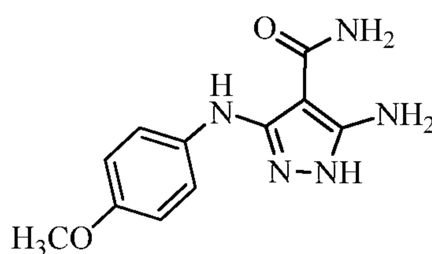
5-amino-3-((4-methoxyphenyl)amino)-1H-pyrazole-4-carboxamide
