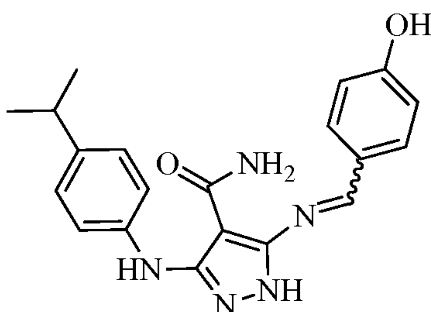
5-((4-hydroxybenzylidene)amino)-3-((4-isopropylphenyl)amino)-1 H -pyrazole-4-carboxamide
