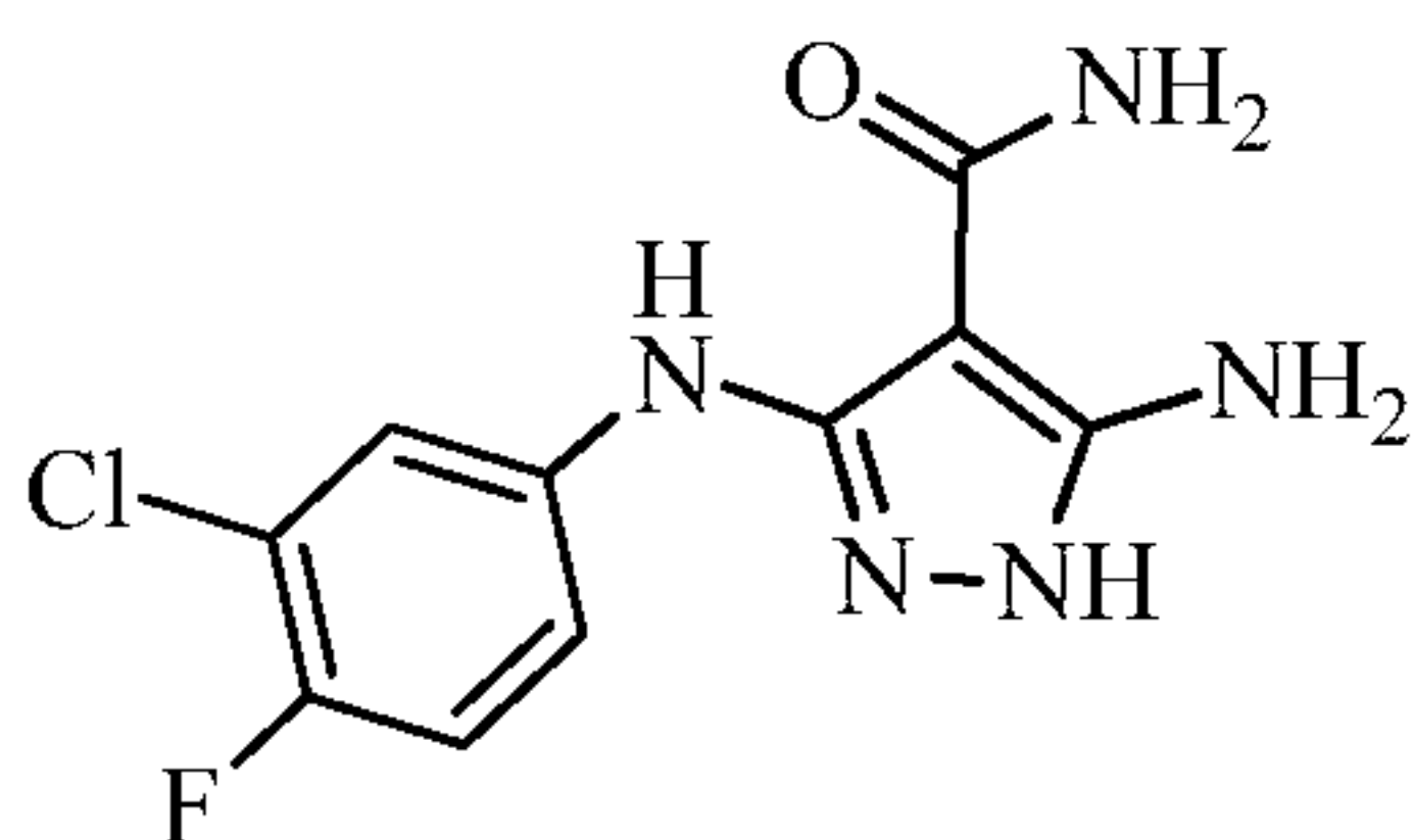
3-((3-chloro-4-fluorophenyl)amino)-5-((4-hydroxybenzylidene)amino)-1 H -pyrazole-4-carboxamide
