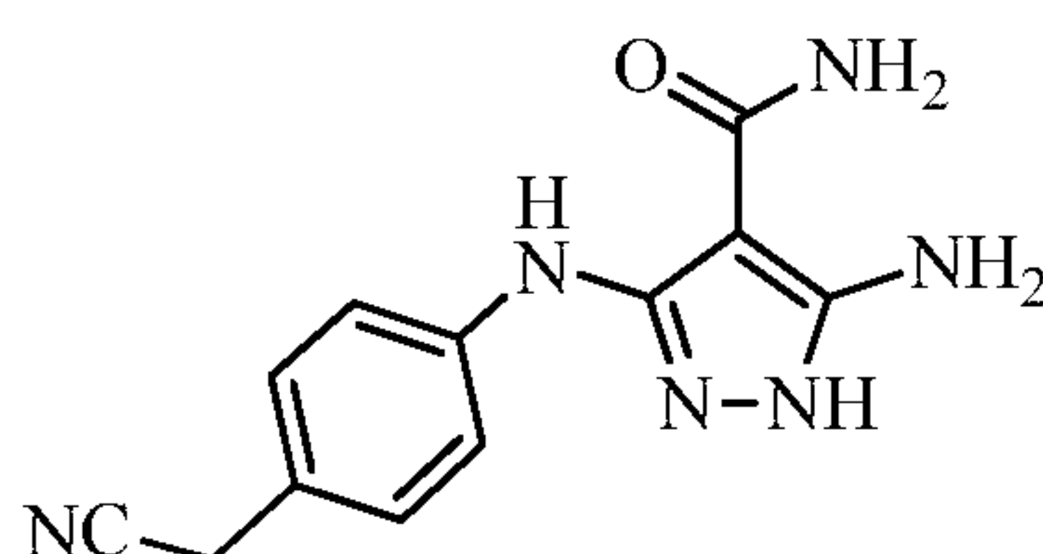
5-amino-3-((4-(cyanomethyl)phenyl)amino)-1 H -pyrazole-4-carboxamide
