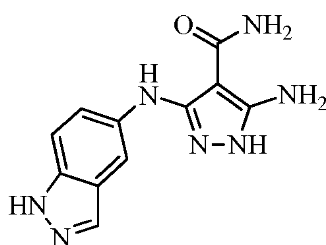
3-((1H-indazol-5-yl)amino)-5-amino-1H-pyrazole-4-carboxamide
