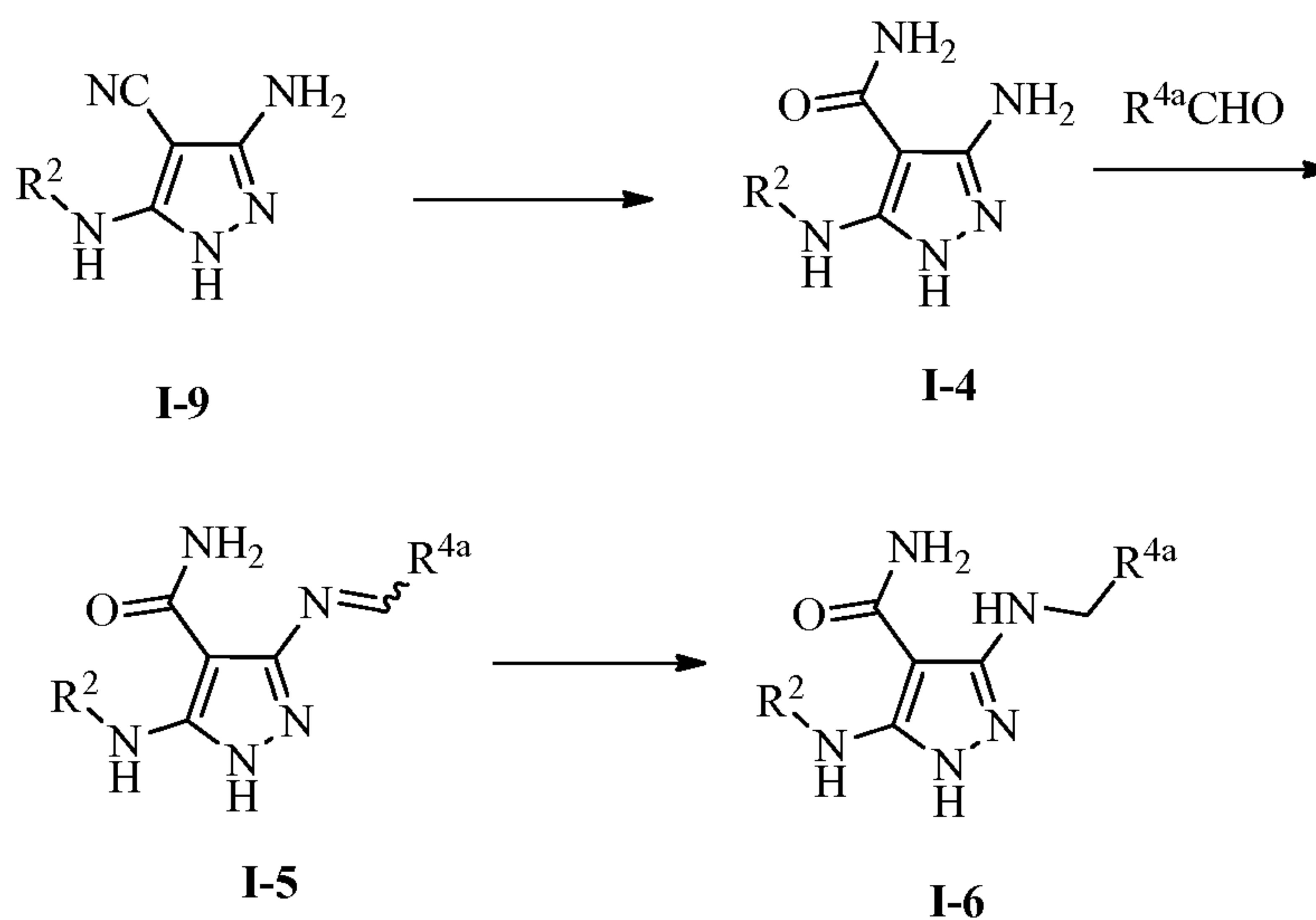
Scheme III
