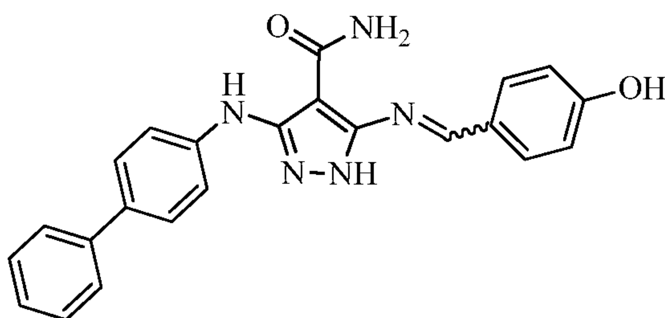
3-([1,1'-biphenyl]-4-ylamino)-5-((4-hydroxybenzylidene)amino)-1 H -pyrazole-4-carboxamide
