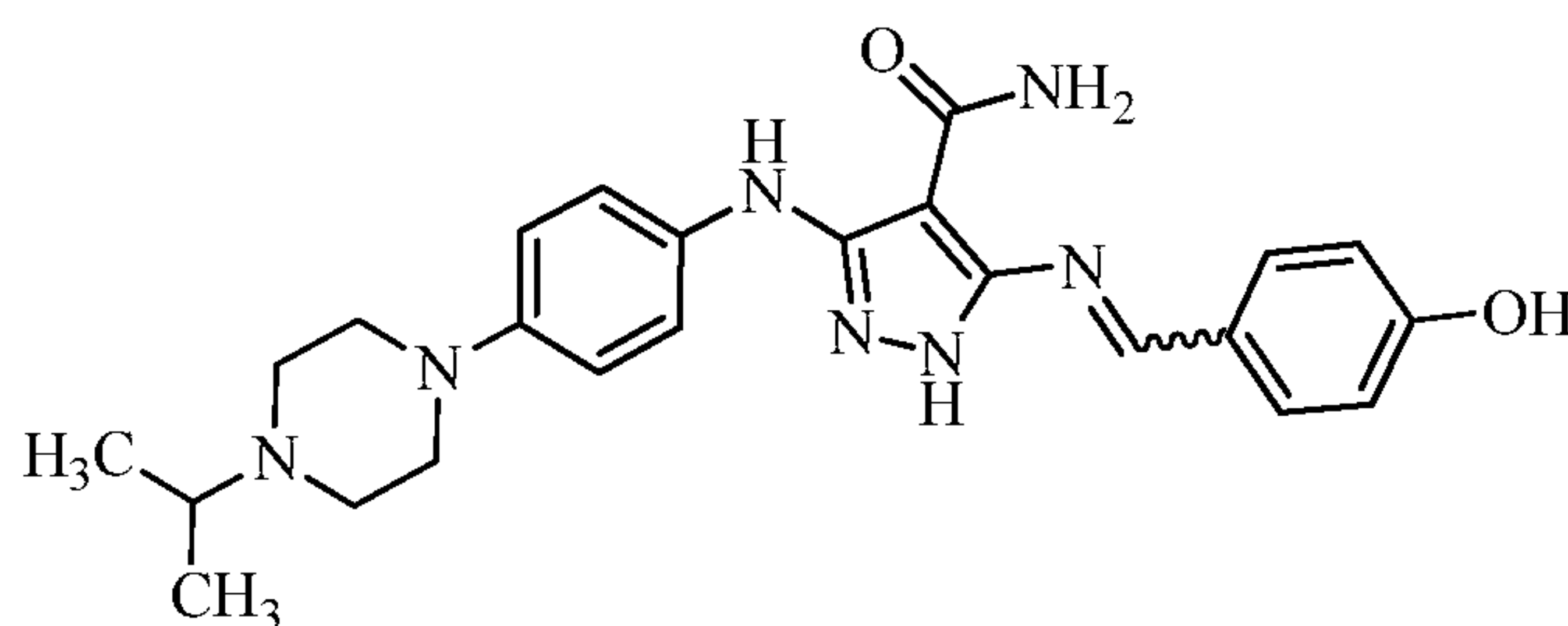
5-((4-hydroxybenzyl)amino)-3-((4-(4-isopropylpiperazin-1-yl)phenyl)amino)-1 H -pyrazole-4-carboxamide
