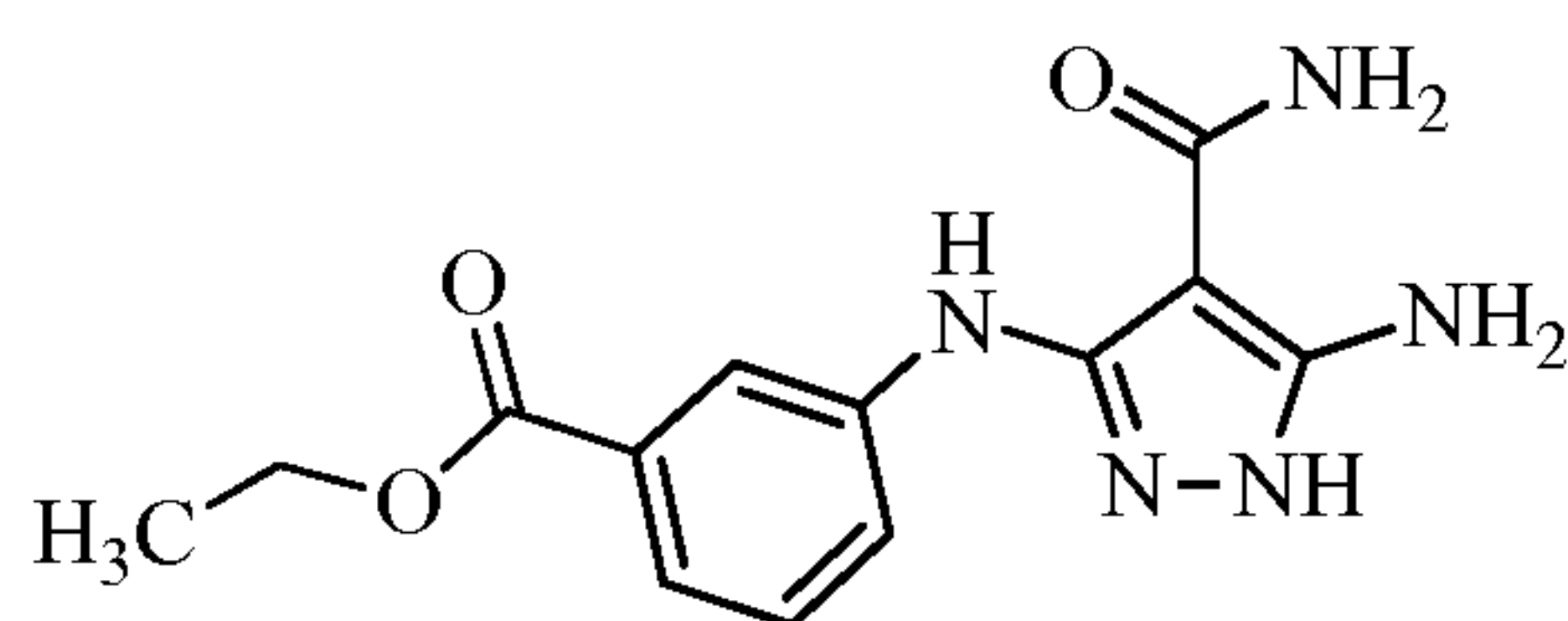
ethyl 3-((5-amino-4-carbamoyl-1H-pyrazol-3-yl)amino)benzoate
