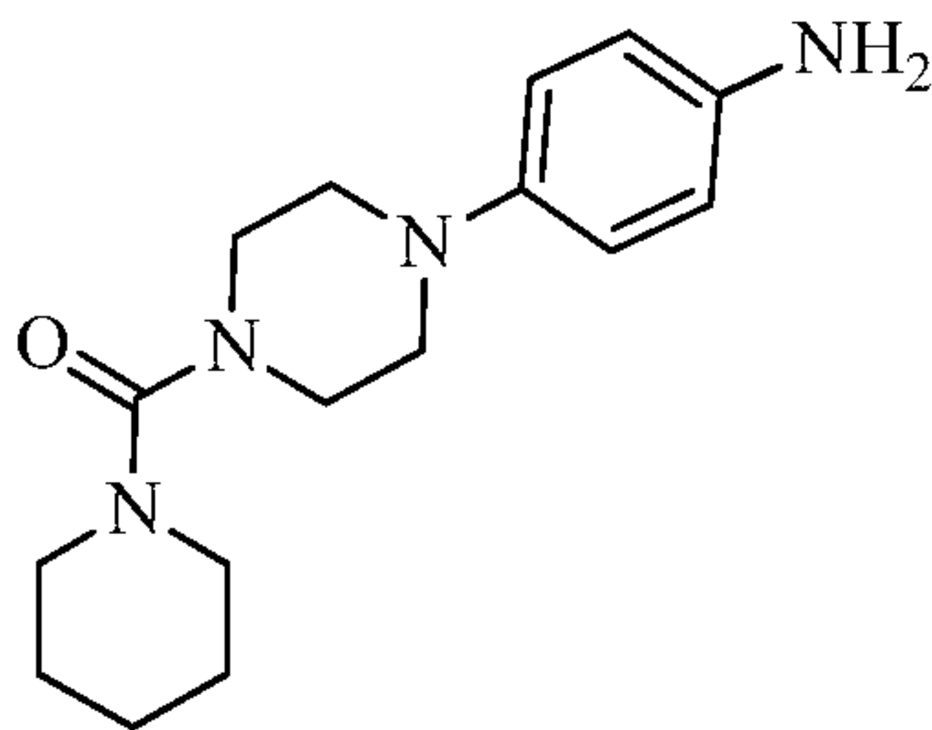
(4-(4-aminophenyl)piperazin-1-yl)(piperidin-1-yl)methanone
