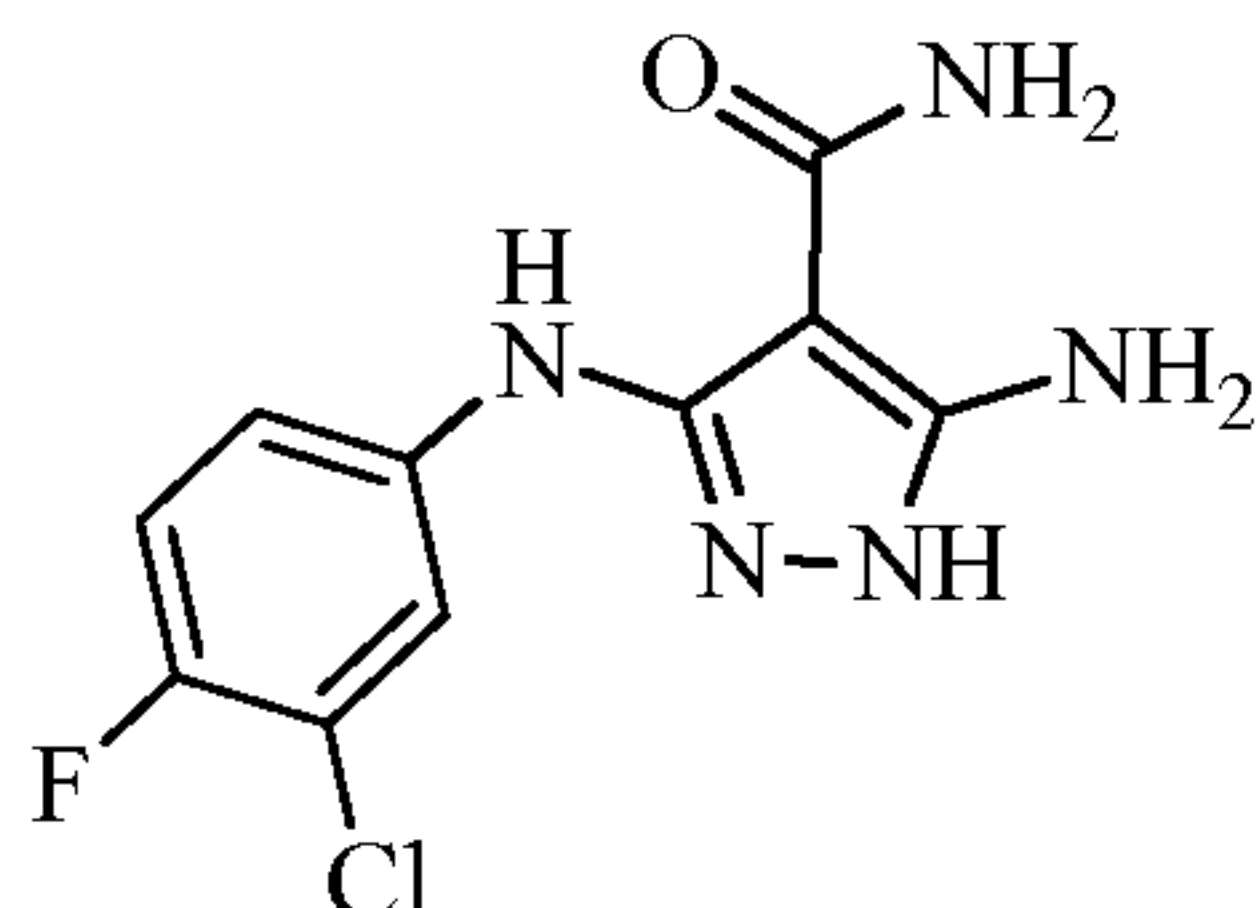
5-amino-3-((3-chloro-4-fluorophenyl)amino)-1H-pyrazole-4-carboxamide
