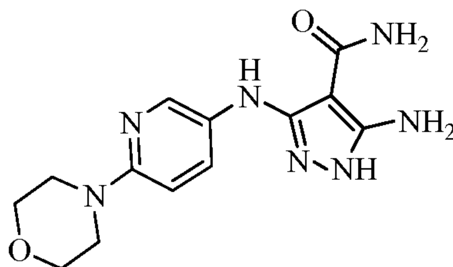
5-amino-3-((6-morpholinopyridin-3-yl)amino)-1H-pyrazole-4-carboxamide
