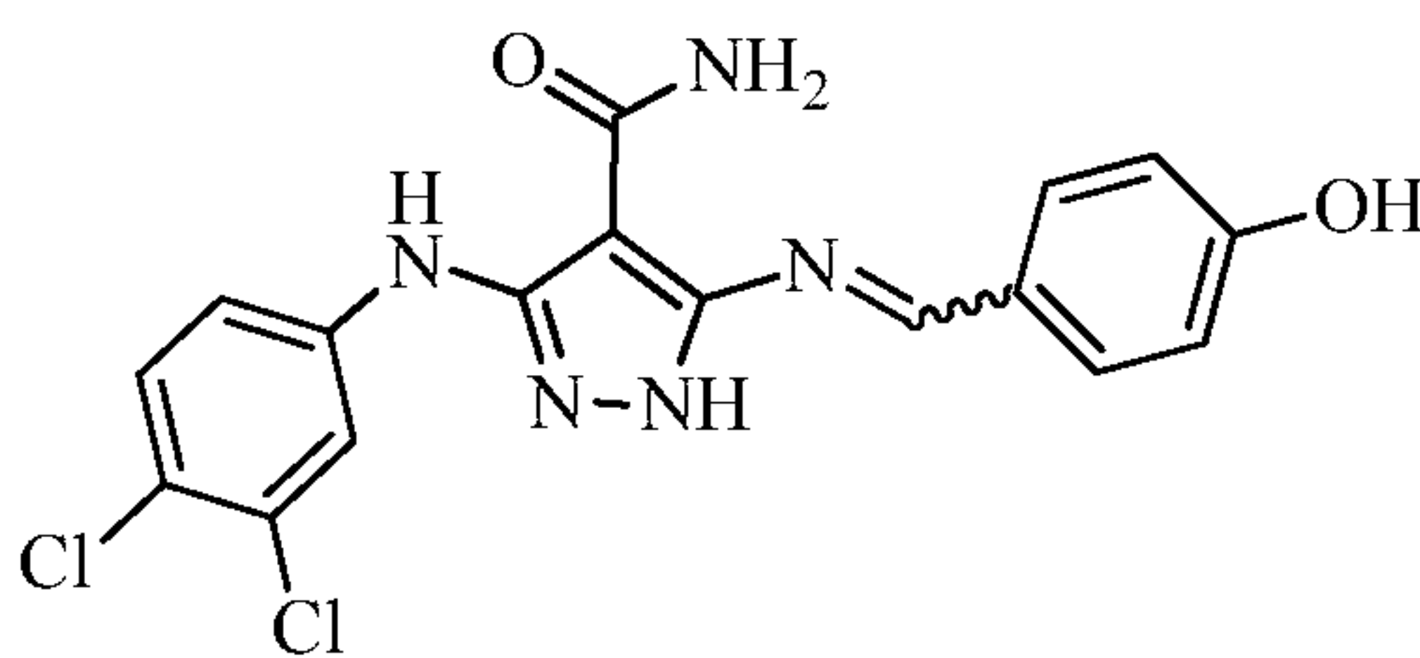
3-((3,4-dichlorophenyl)amino)-5-((4-hydroxybenzylidene)amino)-1 H -pyrazole-4-carboxamide
