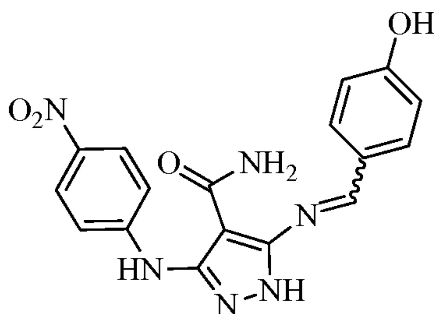
5-((4-hydroxybenzylidene)amino)-3-((4-nitrophenyl)amino)-1 H -pyrazole-4-carboxamide
