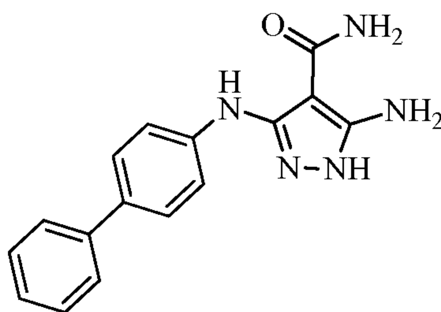
3-([1,1'-biphenyl]-4-ylamino)-5-amino-1 H -pyrazole-4-carboxamide
