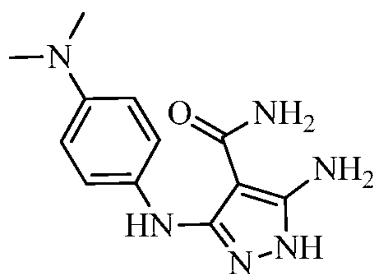
5-amino-3-((4-(dimethylamino)phenyl)amino)-1 H -pyrazole-4-carboxamide
