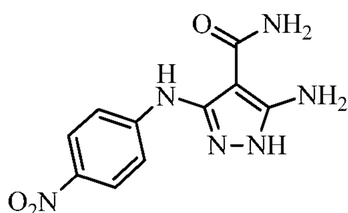
5-amino-3-((4-nitrophenyl)amino)-1H-pyrazole-4-carboxamide
