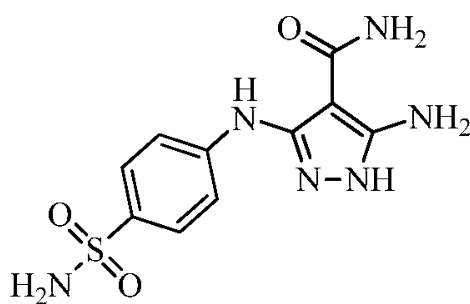
5-amino-3-((4-sulfamoylphenyl)amino)-1H-pyrazole-4-carboxamide
