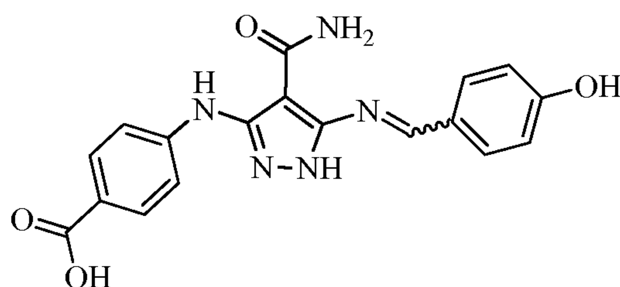
4-((4-carbamoyl-5-((4-hydroxybenzylidene)amino)-1 H -pyrazol-3-yl)amino)benzoic acid
