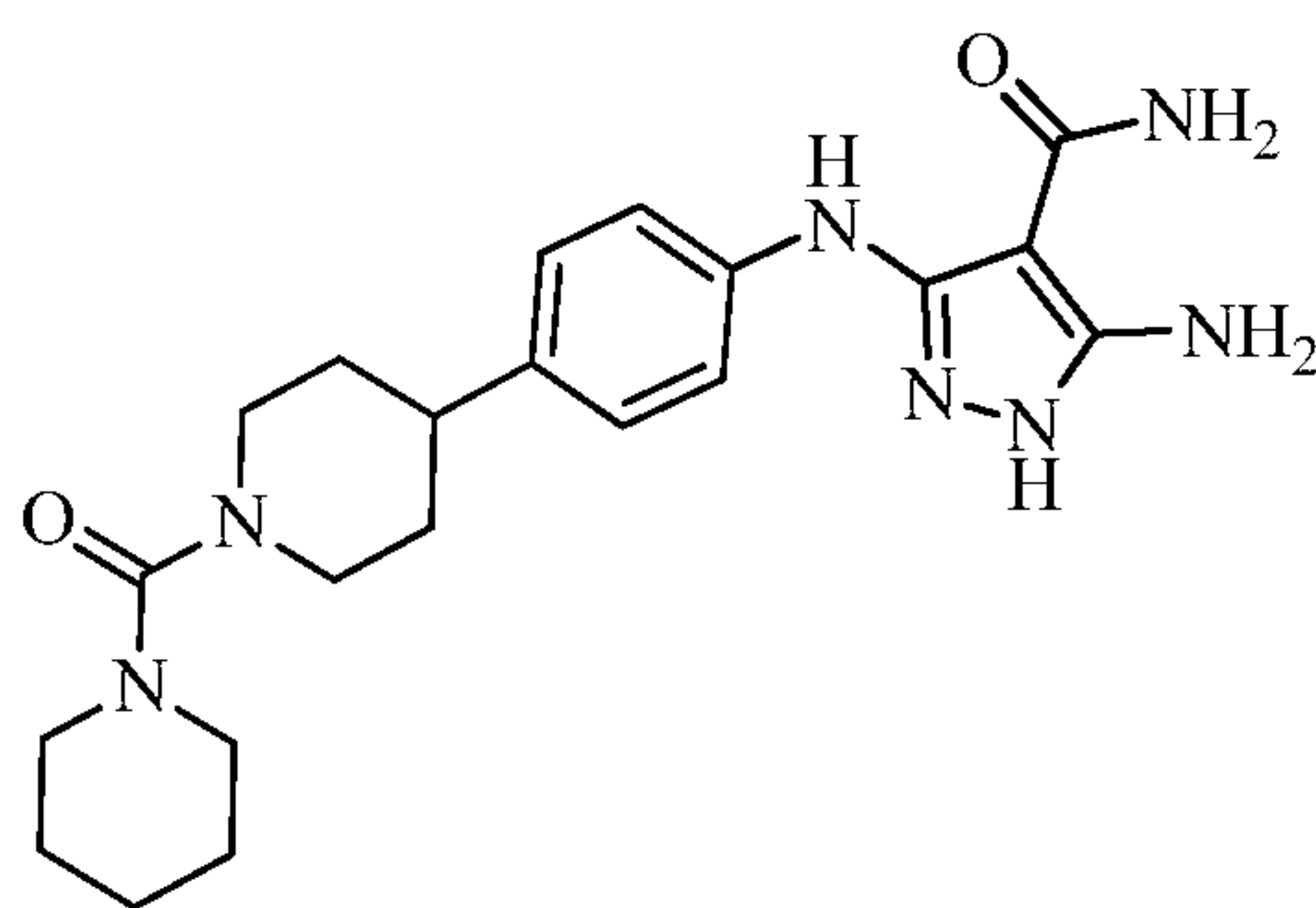
5-amino-3-((4-(1-(piperidine-1-carbonyl)piperidin-4-yl)phenyl)amino)-1 H -pyrazole-4-carboxamide
