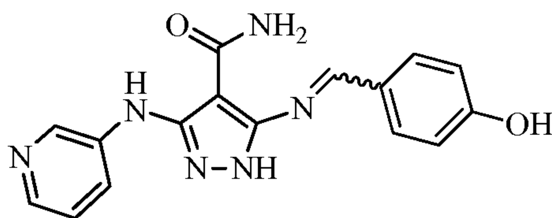
5-((4-hydroxybenzylidene)amino)-3-(pyridin-3-ylamino)-1 H -pyrazole-4-carboxamide
