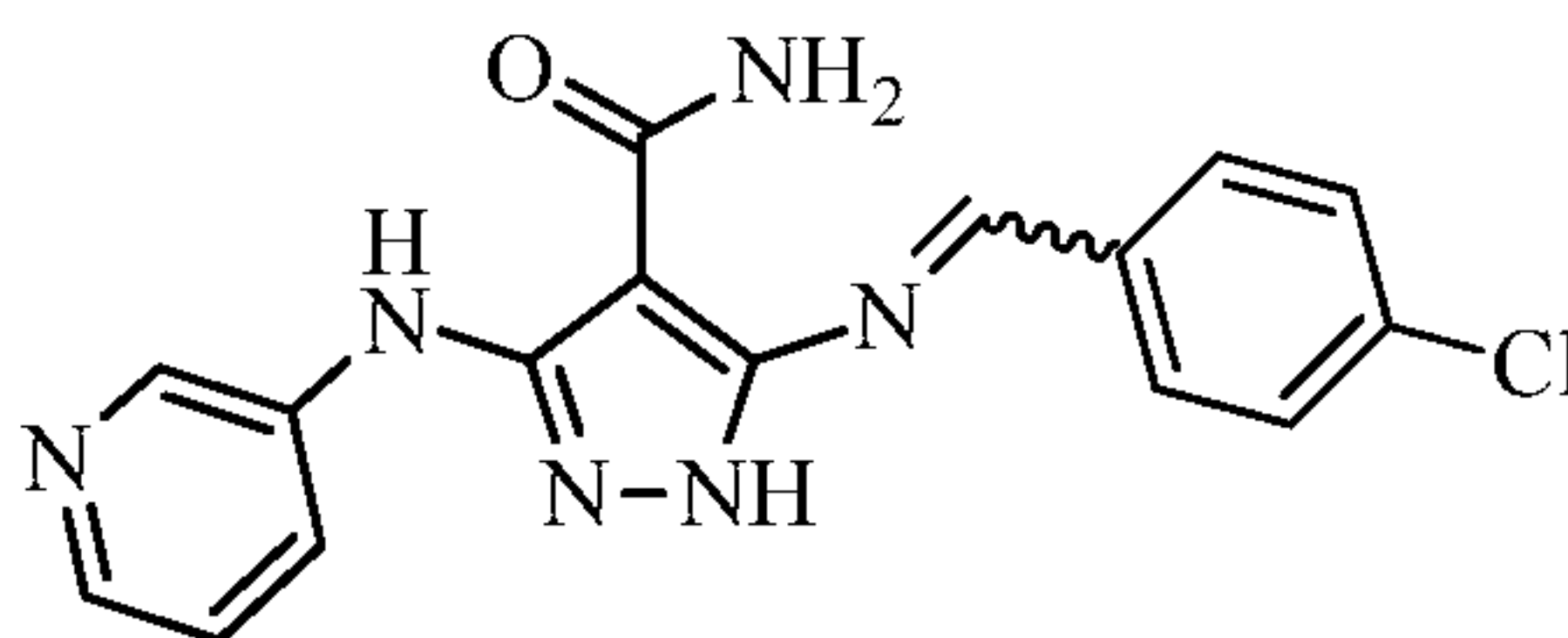
5-((4-chlorobenzylidene)amino)-3-(pyridin-3-ylamino)-1 H -pyrazole-4-carboxamide
