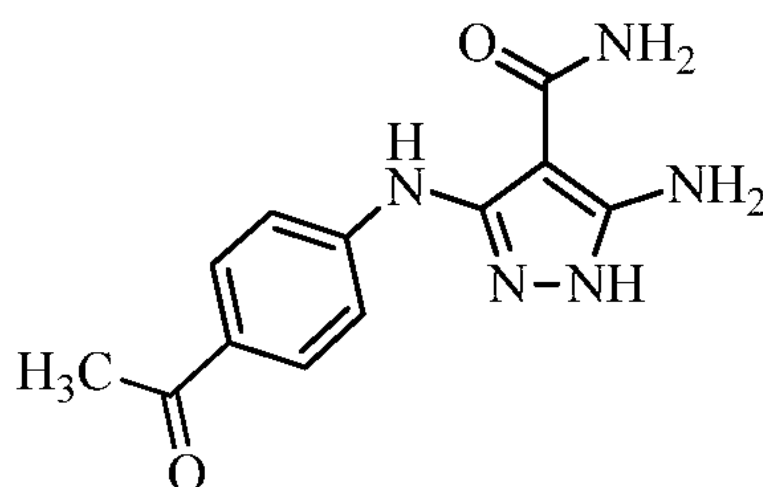
3-((4-acetylphenyl)amino)-5-amino-1 H -pyrazole-4-carboxamide
