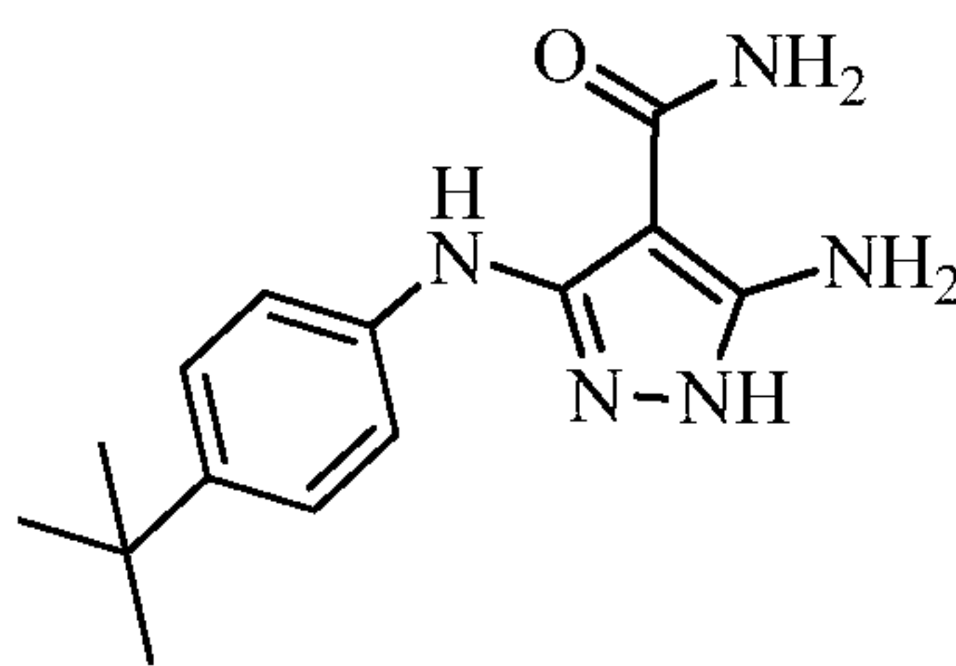
5-amino-3-((4-( tert -butyl)phenyl)amino)-1 H -pyrazole-4-carboxamide
