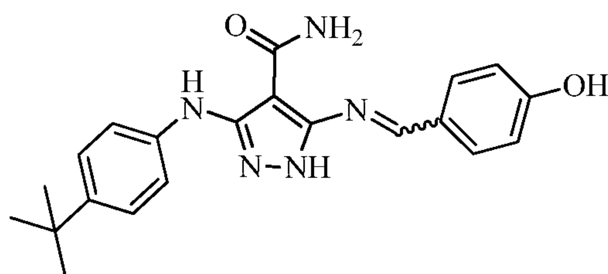
3-((4-( tert -butyl)phenyl)amino)-5-((4-hydroxybenzylidene)amino)-1 H -pyrazole-4-carboxamide
