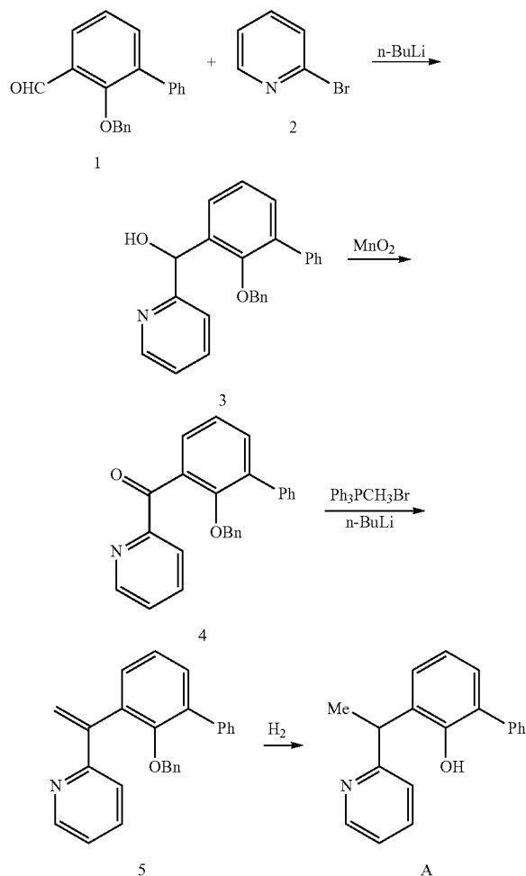
(2-(Benzyloxy)biphenyl-3-yl)(pyridin-2-yl)methanol (3)
