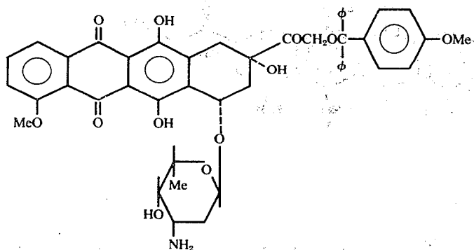
14-O-p-anisylmethyladriamycin XV
