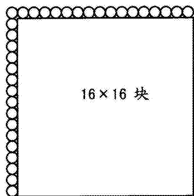
(a) Intra_16×16
