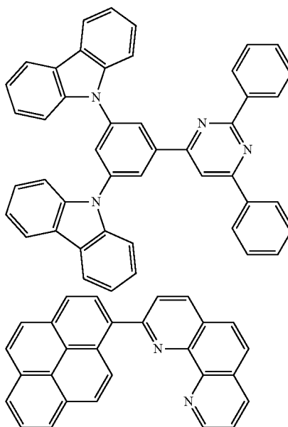
[Chemical Formula 11]
