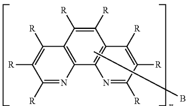
[Chemical Formula 33]
