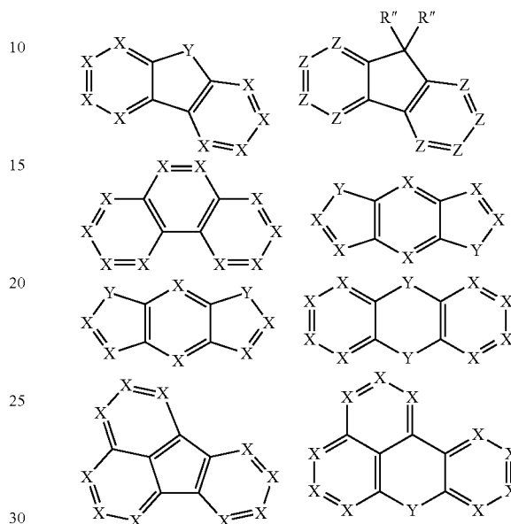
[Chemical Formula 10]
