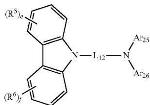
[Chemical Formula 62]
