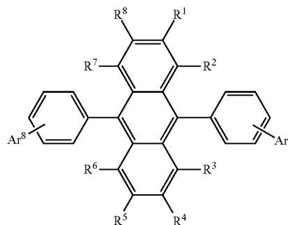
[Chemical Formula 53]
