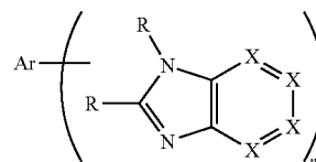
[Chemical Formula 20]
