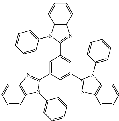
[Chemical Formula 21]
