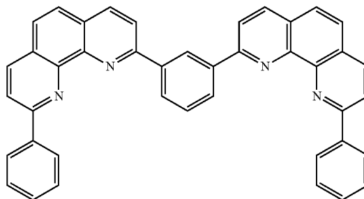
[Chemical Formula 35]
