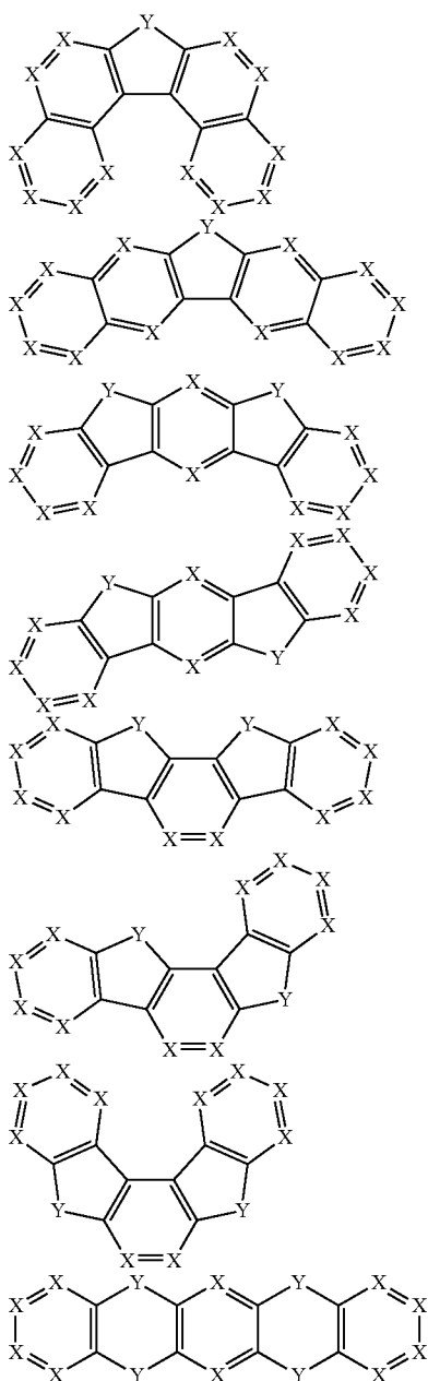
[Chemical Formula 18]
