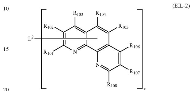
[Chemical Formula 40]
