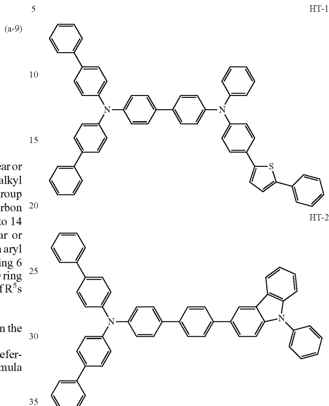
[Chemical Formula 65]
