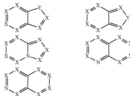
[Chemical Formula 7]
