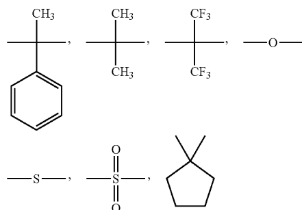
[Chemical Formula 42]
