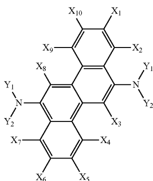
[Chemical Formula 45]
