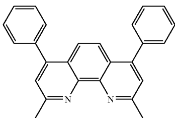
[Chemical Formula 32]
