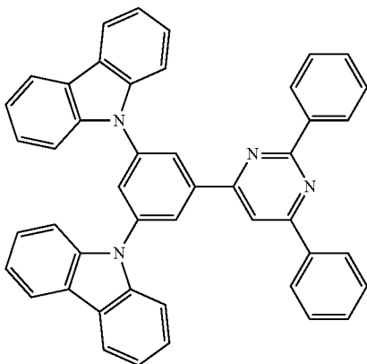
[Chemical Formula 1]
