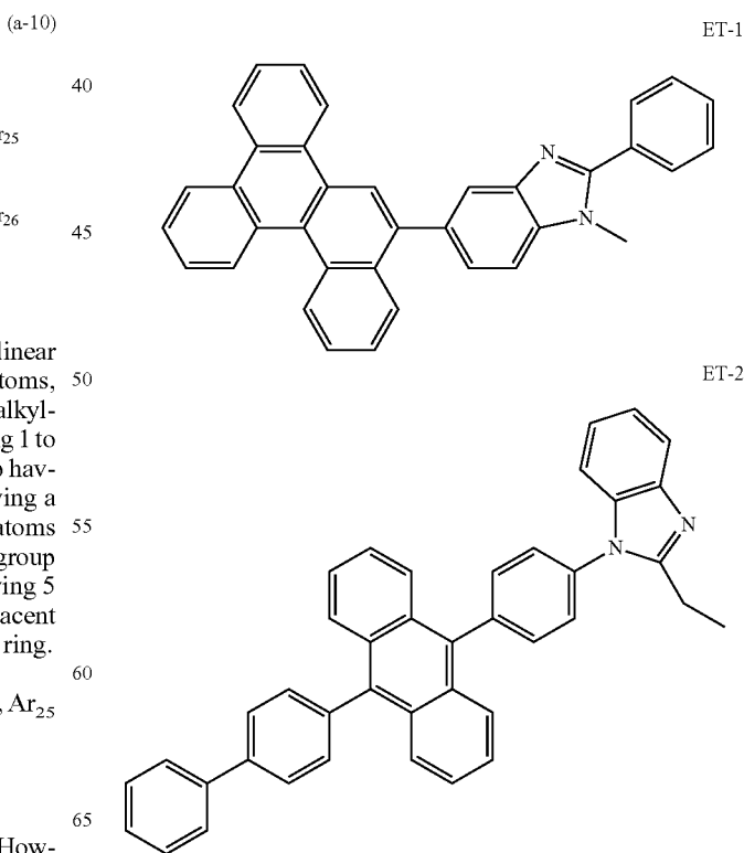
[Chemical Formula 65]
