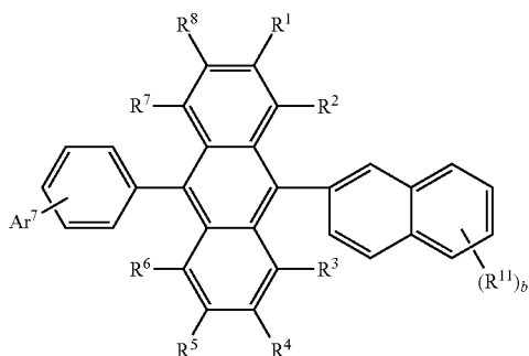
[Chemical Formula 52]
