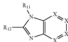
[Chemical Formula 23]
