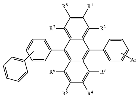
[Chemical Formula 55]
