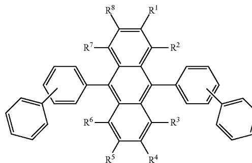
[Chemical Formula 54]
