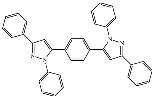
[Chemical Formula 5]
