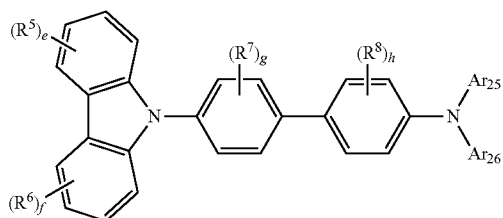
[Chemical Formula 63]
