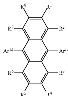
[Chemical Formula 47]
