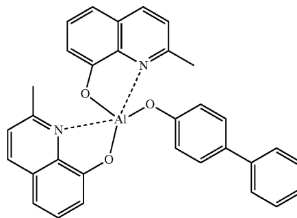
[Chemical Formula 2]
