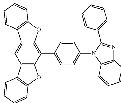
[Chemical Formula 19]
