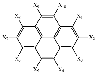
[Chemical Formula 46]
