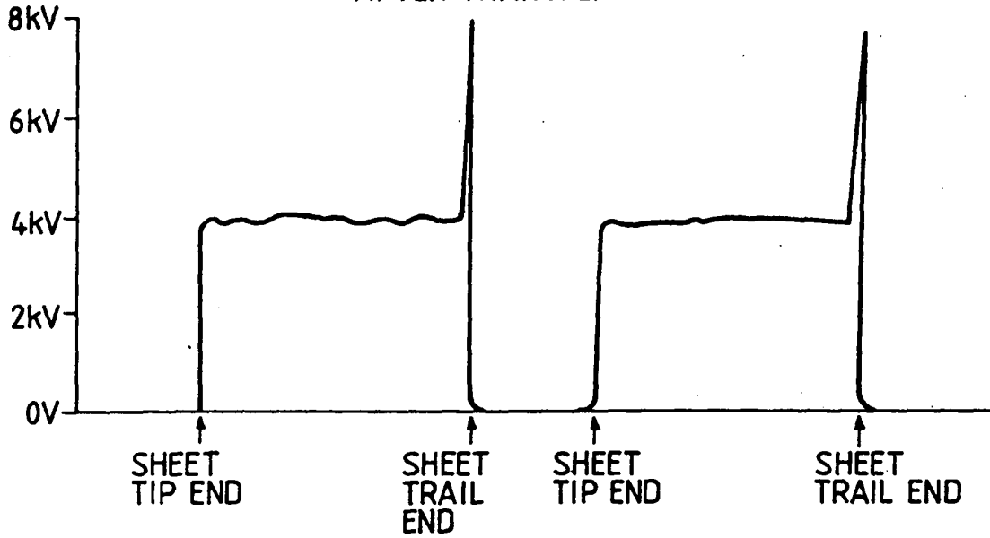
FIG. 2 SHEET POTENTIAL AFTER TRANSFER
