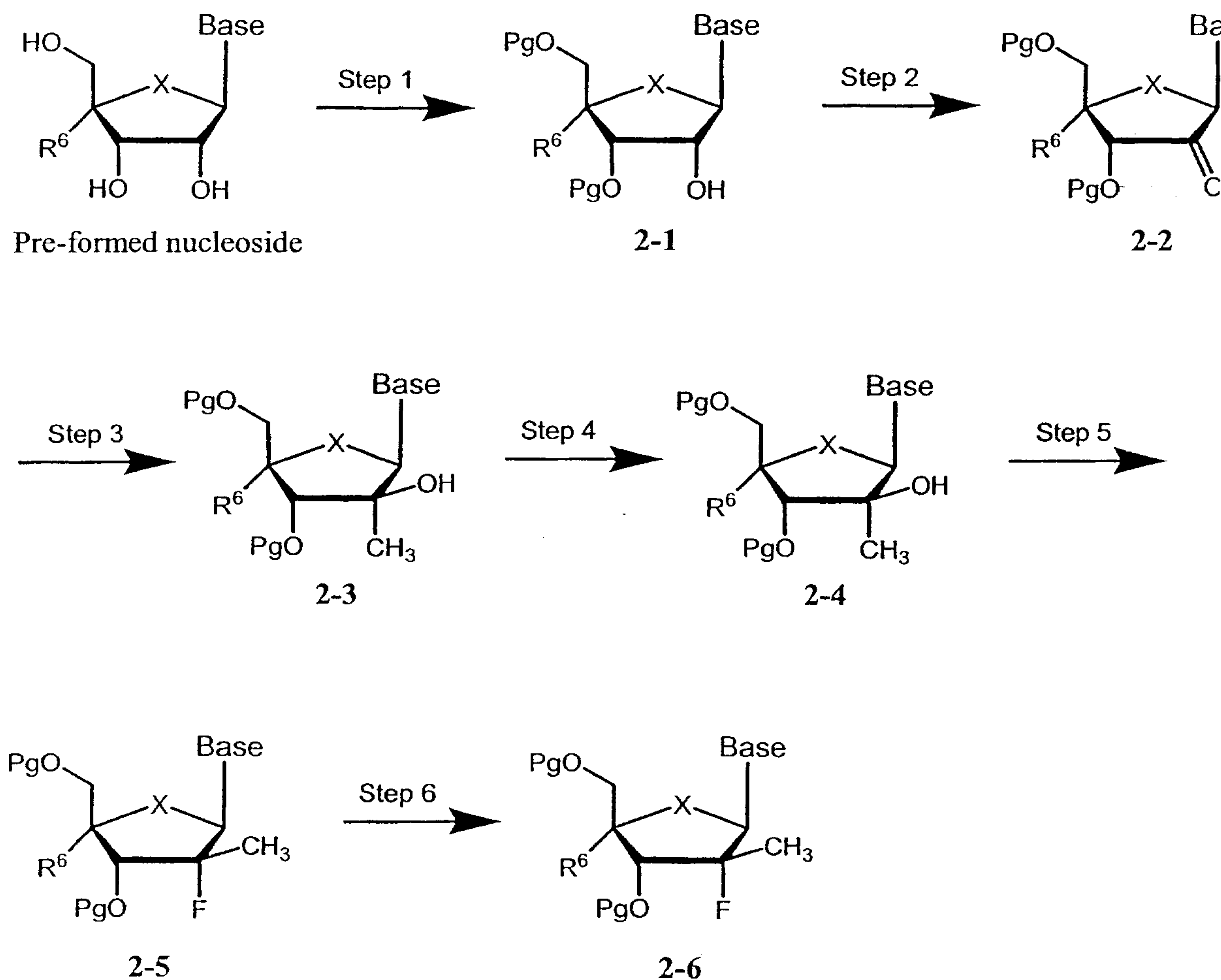
Scheme 2
