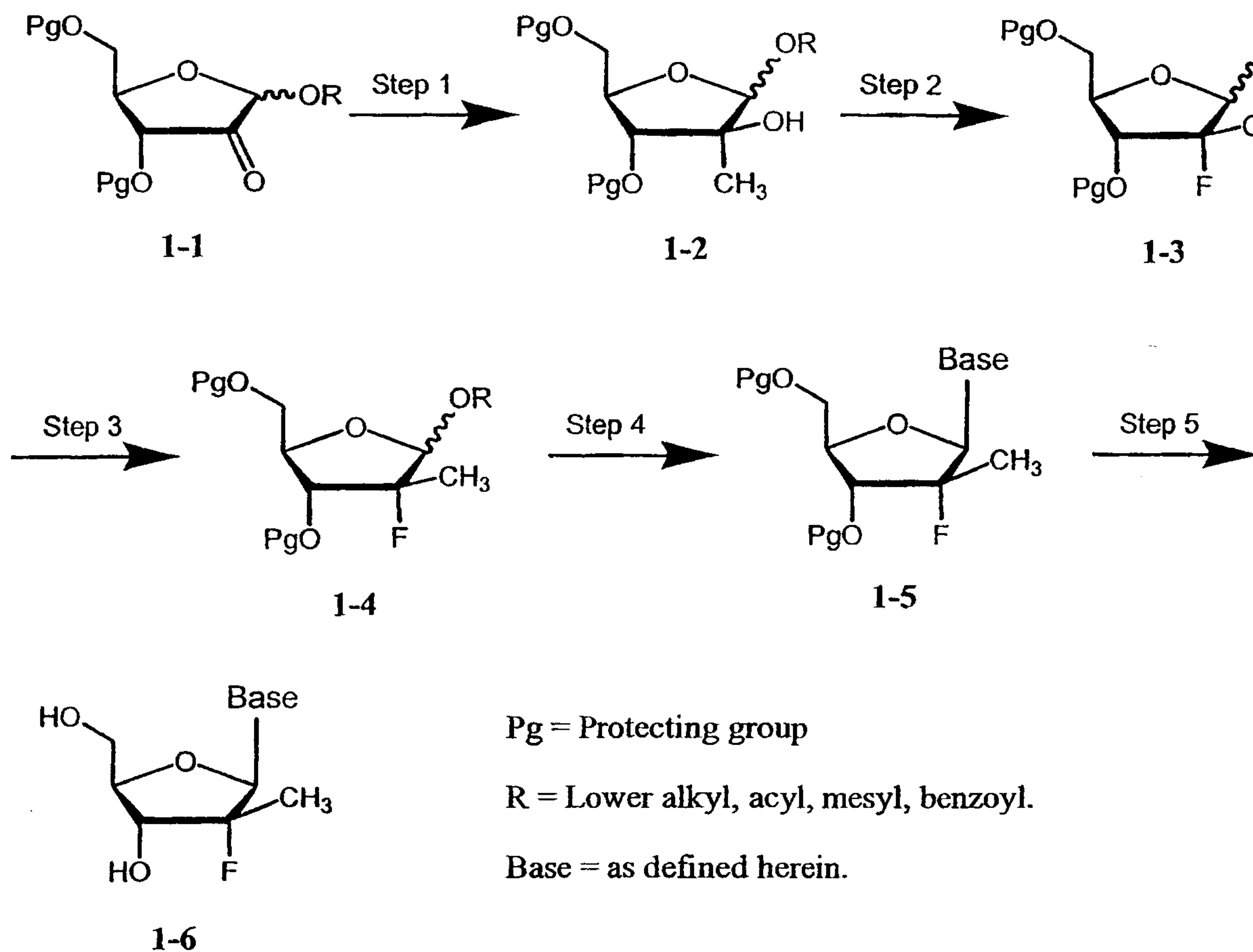
Scheme 1
