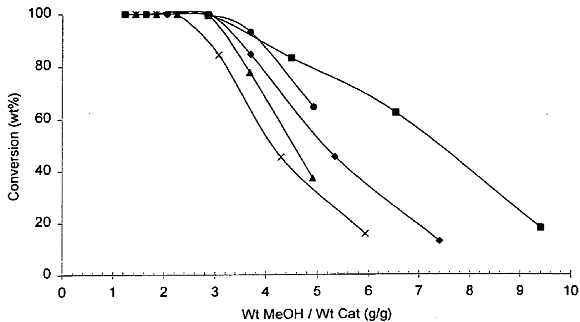
Methanol conversion of NH 3 -treated (at 210°C) SAPO-34 : effect of ageing
