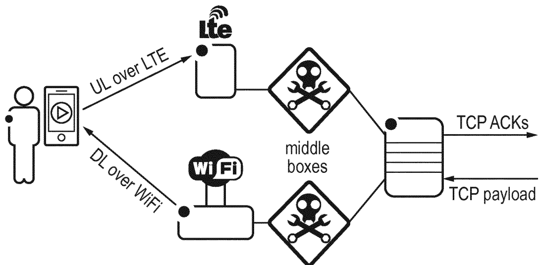
Illustration of asymmetric routing and middle-box interference
