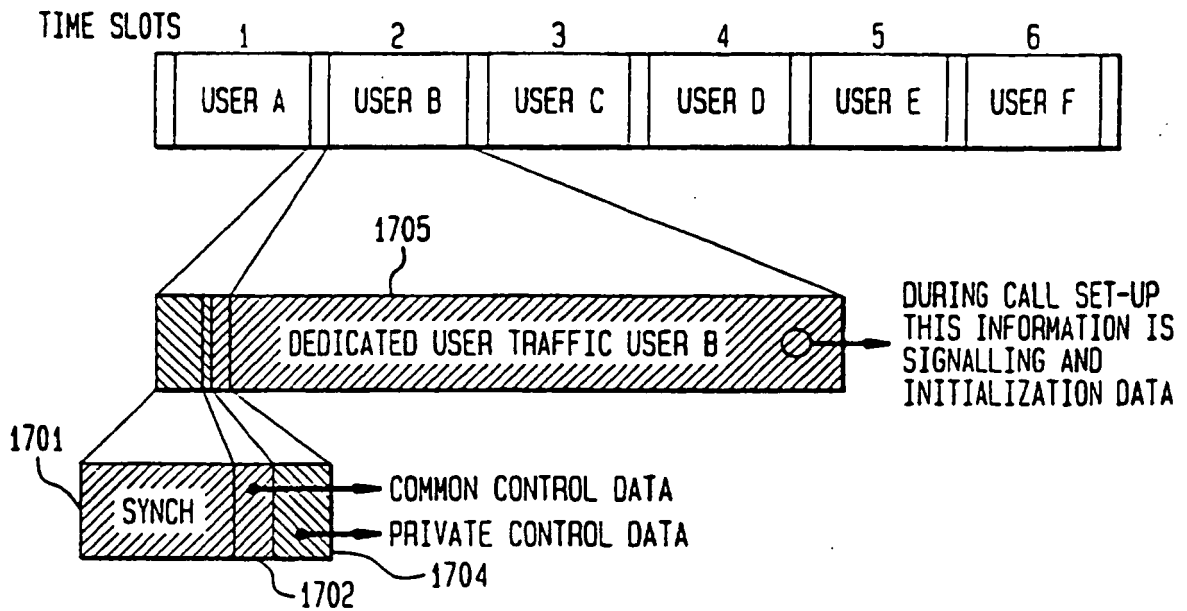
FIG. 17 SYNCH AND CONTROL CHANNEL STRUCTURE
