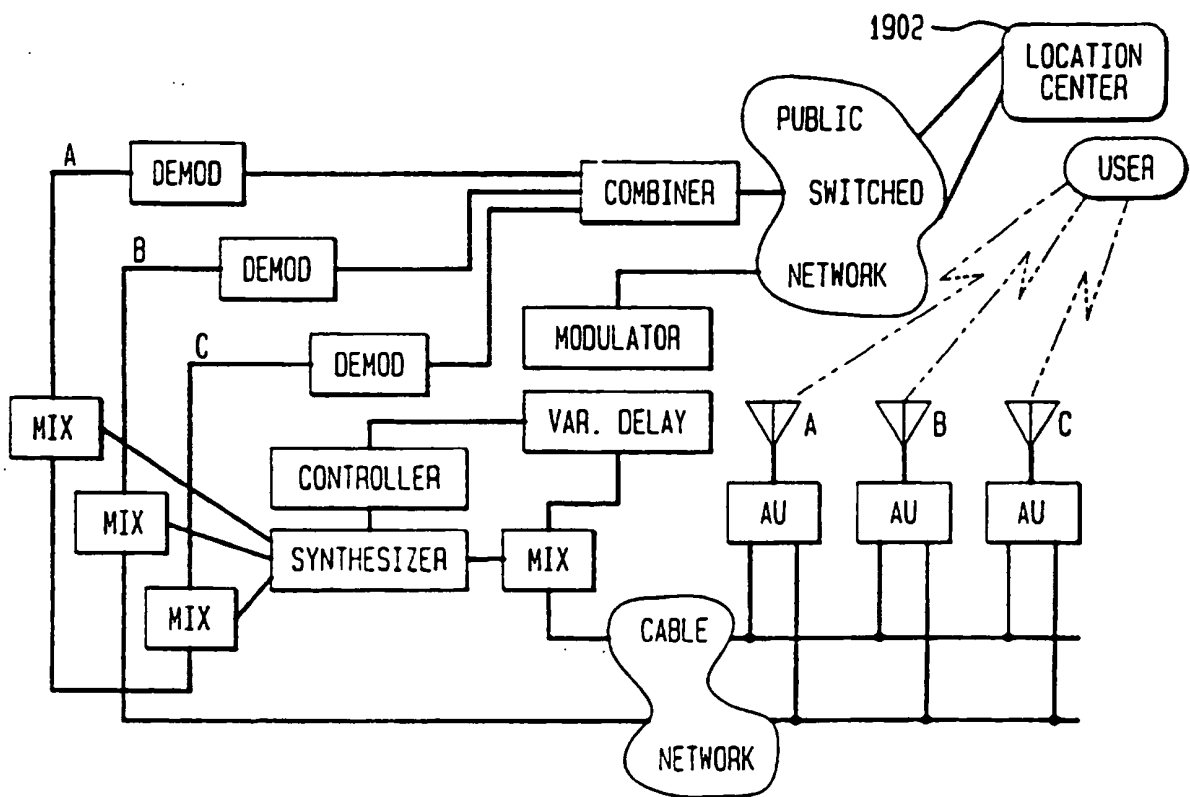
FIG. 19 LOCATION CENTER EXTERNAL TO COMMUNICATION SYSTEM
