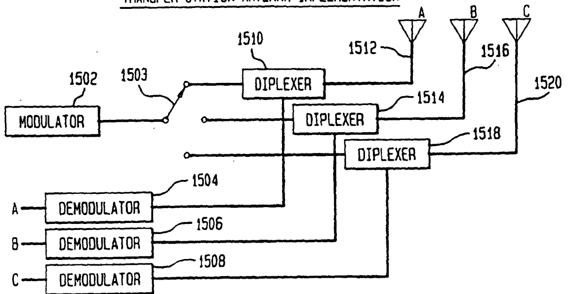
FIG. 15 TRANSFER STATION ANTENNA IMPLEMENTATION
