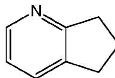
6,7-dihydro-5 H -cyclopenta [ b ]pyridinyl
