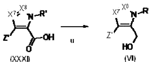
Scheme 8.3
