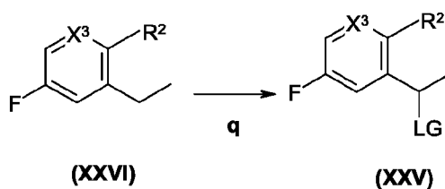
Scheme 6.1
