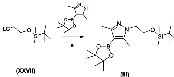
Scheme 7.1
