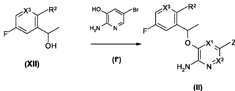
Scheme 2.3
