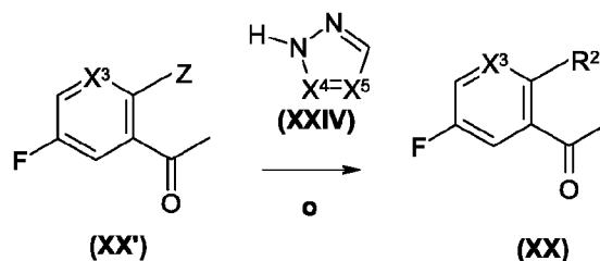
Scheme 5.2
