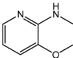
3,4-dihydro-2 H -pyrido [3,2- b ][1,4]oxazinyl
