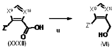
Scheme 8.4
