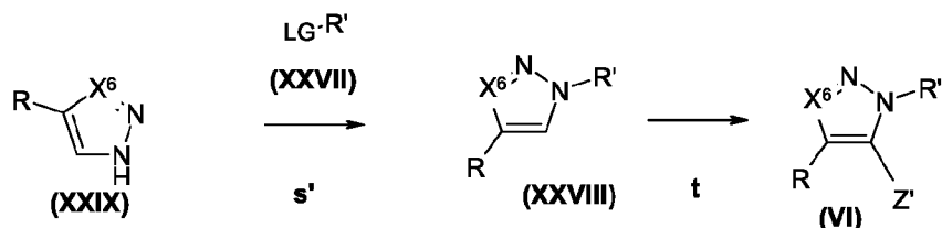
Scheme 8.1
