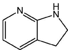
2,3-dihydro-1 H -pyrrolo [2,3- b ]pyridinyl
