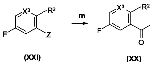
Scheme 5.1
