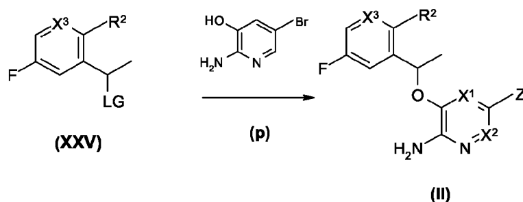
Scheme 2.4
