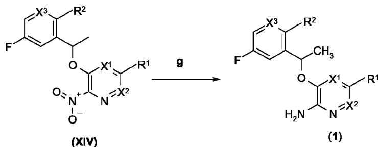
Scheme 1.7
