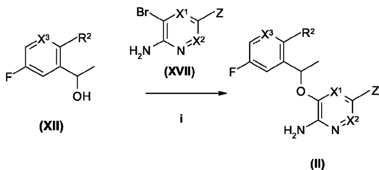
Scheme 2.5
