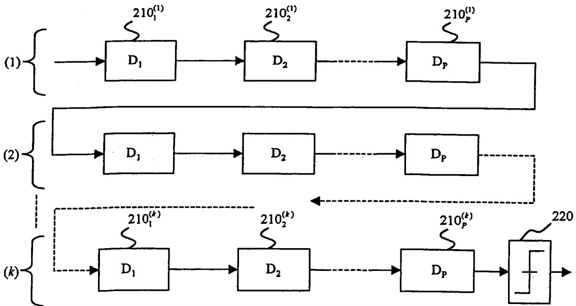
Fig. 2 BACKGROUND ART
