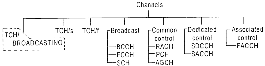
THE GSM CHANNEL ORGANIZATION
