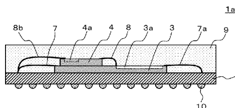
(EXEMPLARY EMBODIMENT 1) X-X'
