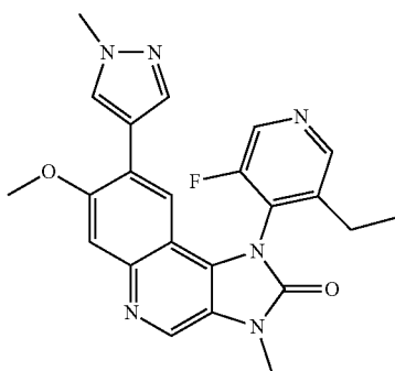
1-(3-Ethyl-5-fluoropyridin-4-yl)-7-methoxy-3-methyl-8-(1-methyl-1H-pyrazol-4-yl)-1,3-dihydroimidazo[4,5-c]quinolin-2-one
