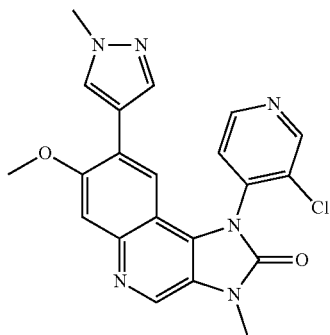
1-(3-Chloropyridin-4-yl)-7-methoxy-3-methyl-8-(1-methyl-1H-pyrazol-4-yl)-1,3-dihydroimidazo[4,5-c]quinolin-2-one
