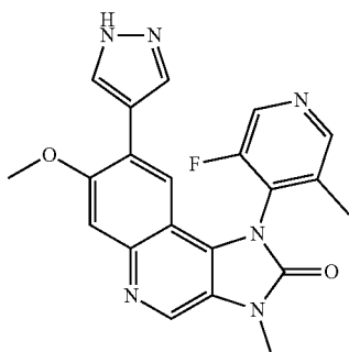
1-(3-Fluoro-5-methylpyridin-4-yl)-7-methoxy-3-methyl-8-(1H-pyrazol-4-yl)-1,3-dihydroimidazo[4,5-c]quinolin-2-one
