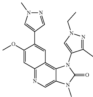
1-(1-Ethyl-3-methyl-1H-pyrazol-4-yl)-7-methoxy-3-methyl-8-(1-methyl-1H-pyrazol-4-yl)-1,3-dihydroimidazo[4,5-c]quinolin-2-one
