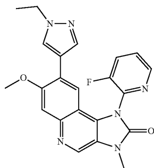
8-(1-Ethyl-1H-pyrazol-4-yl)-1-(3-fluoropyridin-2-yl)-7-methoxy-3-methyl-1,3-dihydroimidazo[4,5-c]quinolin-2-one
