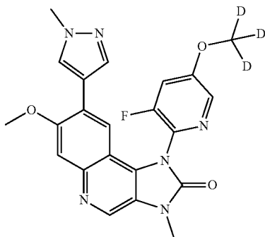
1-[3-Fluoro-5-(trideuteriomethoxy)-2-pyridyl]-7-methoxy-3-methyl-8-(1-methylpyrazol-4-yl)imidazo[4,5-c]quinolin-2-one
