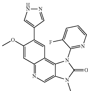
1-(3-Fluoropyridin-2-yl)-7-methoxy-3-methyl-8-(1H-pyrazol-4-yl)-1,3-dihydroimidazo[4,5-c]quinolin-2-one
