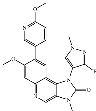
1-(3-Fluoro-1-methyl-1H-pyrazol-4-yl)-7-methoxy-8-(6-methoxypyridin-3-yl)-3-methyl-1,3-dihydroimidazo[4,5-c]quinolin-2-one
