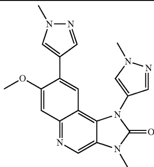
7-Methoxy-3-methyl-1,8-bis-(1-methyl-1H-pyrazol-4-yl)-1,3-dihydroimidazo[4,5-c]quinolin-2-one
