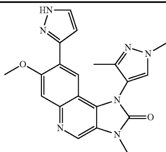
1-(1,3-Dimethyl-1H-pyrazol-4-yl)-7-methoxy-3-methyl-8-(1H-pyrazol-3-yl)-1,3-dihydro-imidazo[4,5-c]quinolin-2-one
