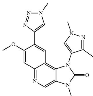
1-(1,3-Dimethyl-1H-pyrazol-4-yl)-7-methoxy-3-methyl-8-(1-methyl-1H-1,2,3-triazol-4-yl)-1,3-dihydroimidazo[4,5-c]quinolin-2-one
