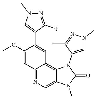
1-(1,3-Dimethyl-1H-pyrazol-4-yl)-7-methoxy-3-methyl-8-(3-fluoro-1-methyl-1H-pyrazol-4-yl)-1,3-dihydroimidazo[4,5-c]quinolin-2-one
