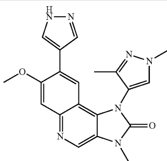
1-(1,3-Dimethyl-1H-pyrazol-4-yl)-7-methoxy-3-methyl-8-(1H-pyrazol-4-yl)-1,3-dihydroimidazo[4,5-c]quinolin-2-one
