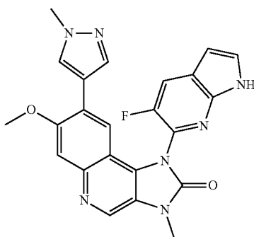
1-(5-Fluoro-1H-pyrrolo[2,3-b]pyridin-6-yl)-7-methoxy-3-methyl-8-(1-methyl-1H-pyrazol-4-yl)-1,3-dihydroimidazo[4,5-c]quinolin-2-one
