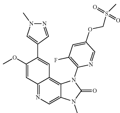
1-(3-Fluoro-5-methylsulfonylmethoxypyridin-2-yl)-7-methoxy-3-methyl-8-(1-methyl-1H-pyrazol-4-yl)-1,3-dihydroimidazo[4,5-c]quinolin-2-one
