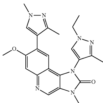
8-(1,3-Dimethyl-1H-pyrazol-4-yl)-1-(1-ethyl-3-methyl-1H-pyrazol-4-yl)-7-methoxy-3-methyl-1,3-dihydroimidazo[4,5-c]quinolin-2-one
