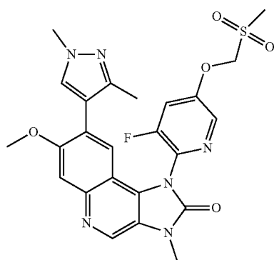
8-(1,3-Dimethyl-1H-pyrazol-4-yl)-1-(3-fluoro-5-methylsulfonylmethoxypyridin-2-yl)-7-methoxy-3-methyl-1,3-dihydroimidazo[4,5-c]quinolin-2-one
