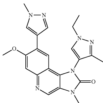
1-(1-Ethyl-3-methyl-1H-pyrazol-4-yl)-7-methoxy-3-methyl-8-(1-methyl-1H-pyrazol-4-yl)-1,3-dihydroimidazo[4,5-c]quinolin-2-one
