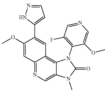
1-(3-Fluoro-5-methoxypyridin-4-yl)-7-methoxy-3-methyl-8-(2H-pyrazol-3-yl)-1,3-dihydroimidazo[4,5-c]quinolin-2-one
