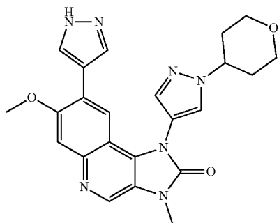
7-Methoxy-3-methyl-8-(1H-pyrazol-4-yl)-1-[1-(tetrahydropyran-4-yl)-1H-pyrazol-4-yl]-1,3-dihydroimidazo[4,5-c]quinolin-2-one
