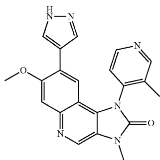
7-Methoxy-3-methyl-1-(3-methylpyridin-4-yl)-8-(1H-pyrazol-4-yl)-1,3-dihydroimidazo[4,5-c]quinolin-2-one
