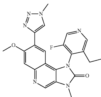
1-(3-Ethyl-5-fluoropyridin-4-yl)-7-methoxy-3-methyl-8-(1-methyl-1H-1,2,3-triazol-4-yl)-1,3-dihydroimidazo[4,5-c] quinolin-2-one
