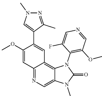
8-(1,3-Dimethyl-1H-pyrazol-4-yl)-1-(3-fluoro-5-methoxypyridin-4-yl)-7-methoxy-3-methyl-1,3-dihydroimidazo[4,5-c]quinolin-2-one
