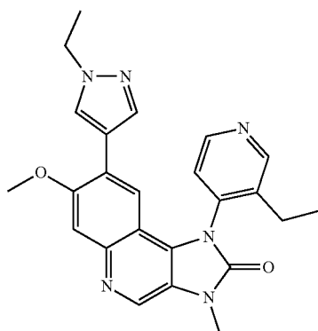
8-(1-Ethyl-1H-pyrazol-4-yl)-1-(3-ethylpyridin-4-yl)-7-methoxy-3-methyl-1,3-dihydroimidazo[4,5-c]quinolin-2-one
