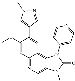
7-Methoxy-3-methyl-8-(1-methyl-1H-pyrazol-4-yl)-1-pyridin-4-yl-1,3-dihydroimidazo[4,5-c]quinolin-2-one
