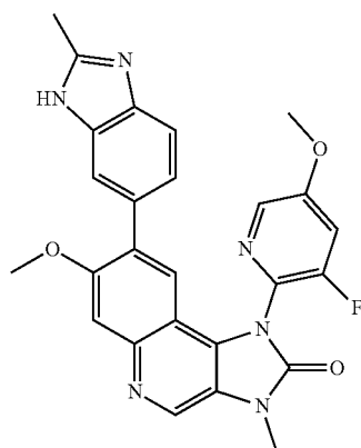
1-(3-Fluoro-5-methoxypyridin-2-yl)-7-methoxy-3-methyl-8-(2-methyl-3H-benzimidazol-5-yl)-1,3-dihydroimidazo[4,5-c]quinolin-2-one
