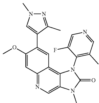
8-(1,3-Dimethyl-1H-pyrazol-4-yl)-1-(3-fluoro-5-methylpyridin-4-yl)-7-methoxy-3-methyl-1,3-dihydroimidazo[4,5-c]quinolin-2-one
