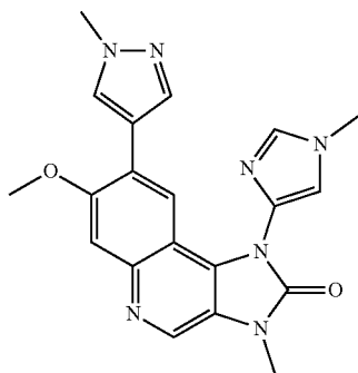
7-Methoxy-3-methyl-1-(1-methyl-1H-imidazol-4-yl)-8-(1-methyl-1H-pyrazol-4-yl)-1,3-dihydroimidazo[4,5-c]quinolin-2-one
