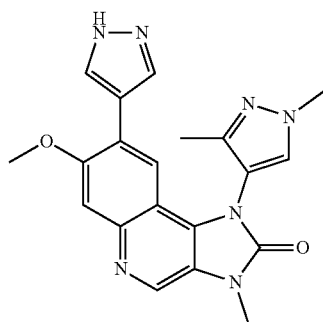
1-(1,3-Dimethyl-1H-pyrazol-4-yl)-7-methoxy-3-methyl-8-(1H-pyrazol-4-yl)-1,3-dihydroimidazo[4,5-c]quinolin-2-one
