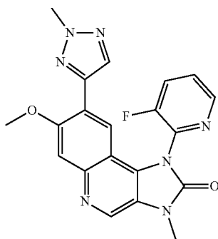
1-(3-Fluoropyridin-2-yl)-7-methoxy-3-methyl-8-(2-methyl-2H-1,2,3-triazol-4-yl)-1,3-dihydroimidazo[4,5-c]quinolin-2-one
