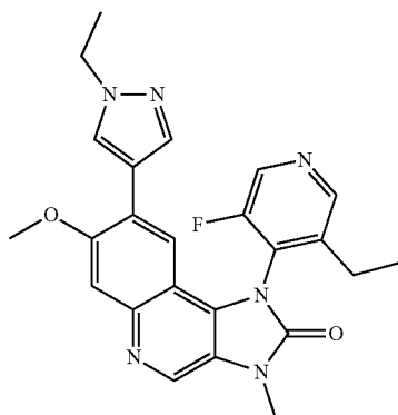
1-(3-Ethyl-5-fluoropyridin-4-yl)-8-(1-ethyl-1H-pyrazol-4-yl)-7-methoxy-3-methyl-1,3-dihydroimidazo[4,5-c]quinolin-2-one
