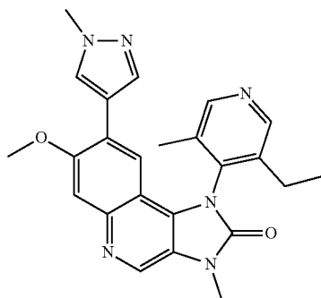
1-(3-Ethyl-5-methylpyridin-4-yl)-7-methoxy-3-methyl-8-(1-methyl-1H-pyrazol-4-yl)-1,3-dihydroimidazo[4,5-c]quinolin-2-one
