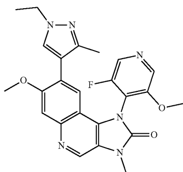
8-(1-Ethyl-3-methyl-1H-pyrazol-4-yl)-1-(3-fluoro-5-methoxypyridin-4-yl)-7-methoxy-3-methyl-1,3-dihydroimidazo[4,5-c]quinolin-2-one
