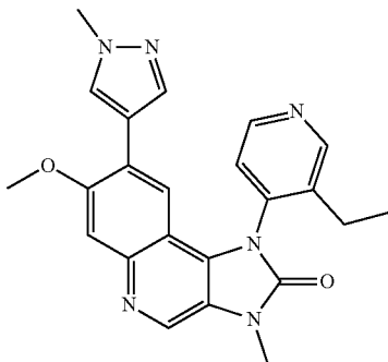
1-(3-Ethylpyridin-4-yl)-7-methoxy-3-methyl-8-(1-methyl-1H-pyrazol-4-yl)-1,3-dihydroimidazo[4,5-c]quinolin-2-one
