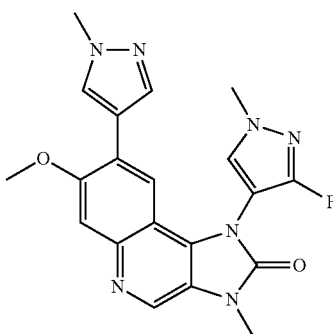
1-(3-Fluoro-1-methyl-1H-pyrazol-4-yl)-7-methoxy-3-methyl-8-(1-methyl-1H-pyrazol-4-yl)-1,3-dihydroimidazo[4,5-c]quinolin-2-one
