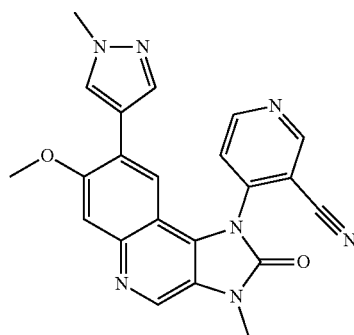
4-[7-Methoxy-3-methyl-8-(1-methyl-1H-pyrazol-4-yl)-2-oxo-2,3-dihydroimidazo[4,5-c]quinolin-1-yl]nicotinonitrile
