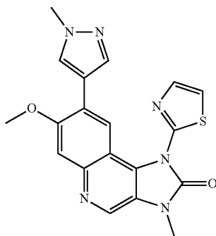
7-Methoxy-3-methyl-8-(1-methyl-1H-pyrazol-4-yl)-1-thiazol-2-yl-1,3-dihydroimidazo[4,5-c]quinolin-2-one
