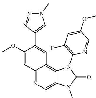
1-(3-Fluoro-5-methoxypyridin-2-yl)-7-methoxy-3-methyl-8-(1-methyl-1H-1,2,3-triazol-4-yl)-1,3-dihydroimidazo[4,5-c]quinolin-2-one
