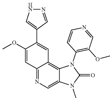
7-Methoxy-1-(3-methoxypyridin-4-yl)-3-methyl-8-(1H-pyrazol-4-yl)-1,3-dihydroimidazo[4,5-c]quinolin-2-one
