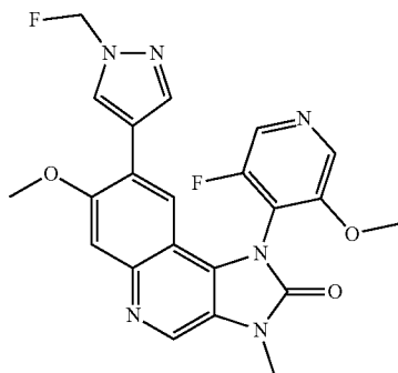
1-(3-Fluoro-5-methoxypyridin-4-yl)-8-(1-fluoromethyl-1H-pyrazol-4-yl)-7-methoxy-3-methyl-1,3-dihydroimidazo[4,5-c]quinolin-2-one
