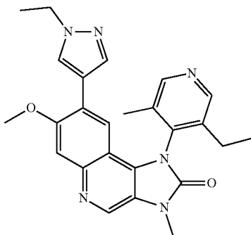
1-(3-Ethyl-5-methylpyridin-4-yl)-8-(1-ethyl-1H-pyrazol-4-yl)-7-methoxy-3-methyl-1,3-dihydroimidazo[4,5-c]quinolin-2-one
