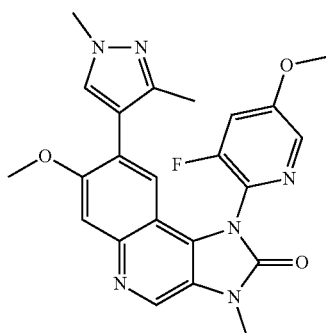
8-(1,3-Dimethyl-1H-pyrazol-4-yl)-1-(3-fluoro-5-methoxypyridin-2-yl)-7-methoxy-3-methyl-1,3-dihydroimidazo[4,5-c]quinolin-2-one
