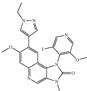
8-(1-Ethyl-1H-pyrazol-4-yl)-1-(3-fluoro-5-methoxypyridin-4-yl)-7-methoxy-3-methyl-1,3-dihydroimidazo[4,5-c]quinolin-2-one
