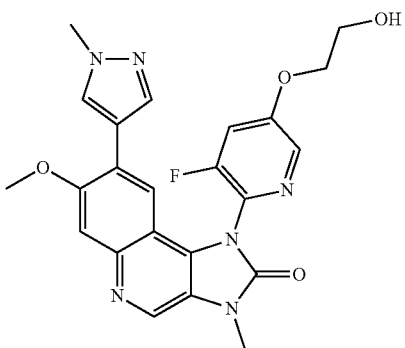
1-[3-Fluoro-5-(2-hydroxyethoxy)-2-pyridyl]-7-methoxy-3-methyl-8-(1-methylpyrazol-4-yl)imidazo[4,5-c]quinolin-2-one
