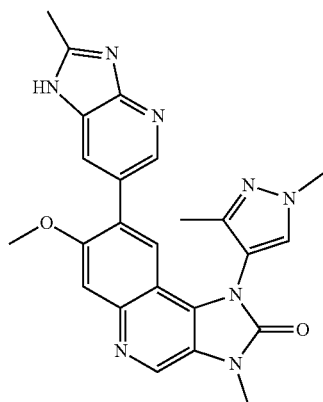
1-(1,3-Dimethyl-1H-pyrazol-4-yl)-7-methoxy-3-methyl-8-(2-methyl-1H-imidazo[4,5-b]pyridin-6-yl)-1,3-dihydroimidazo[4,5-c]quinolin-2-one
