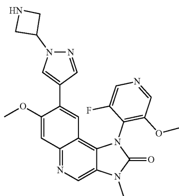
8-[1-(Azetidin-3-yl)-1H-pyrazol-4-yl]-1-(3-fluoro-5-methoxy-pyridin-4-yl)-7-methoxy-3-methyl-1H,2H,3H-imidazo[4,5-c]-quinolin-2-one
