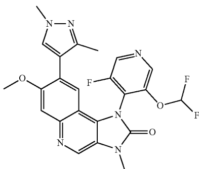
1-(3-Difluoromethoxy-5-fluoropyridin-4-yl)-8-(1,3-dimethyl-1H-pyrazol-4-yl)-7-methoxy-3-methyl-1,3-dihydroimidazo[4,5-c]quinolin-2-one
