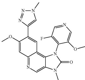
1-(3-Fluoro-5-methoxypyridin-4-yl)-7-methoxy-3-methyl-8-(1-methyl-1H-1,2,3-triazol-4-yl)-1,3-dihydroimidazo[4,5-c]quinolin-2-one
