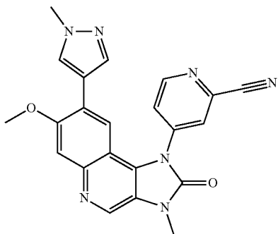
4-[7-Methoxy-3-methyl-8-(1-methyl-1H-pyrazol-4-yl)-2-oxo-2,3-dihydroimidazo[4,5-c]quinolin-1-yl]pyridine-2-carbonitrile
