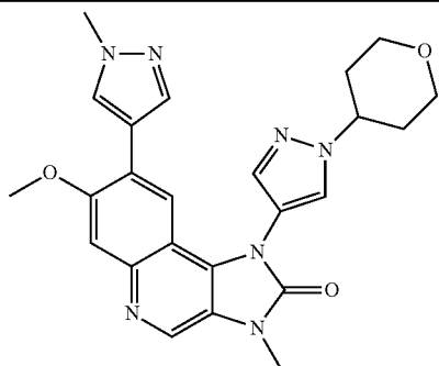
7-Methoxy-3-methyl-8-(1-methyl-1H-pyrazol-4-yl)-1-[1-(tetrahydropyran-4-yl)-1H-pyrazol-4-yl]-1,3-dihydroimidazo[4,5-c]quinolin-2-one
