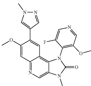
1-(3-Fluoro-5-methoxypyridin-4-yl)-7-methoxy-3-methyl-8-(1-methyl-1H-pyrazol-4-yl)-1,3-dihydroimidazo[4,5-c]quinolin-2-one
