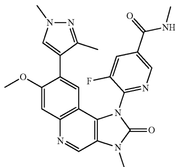
6-[8-(1,3-Dimethyl-1H-pyrazol-4-yl)-7-methoxy-3-methyl-2-oxo-2,3-dihydroimidazo[4,5-c]quinolin-1-yl]-5-fluoro-N-methylnicotinamide
