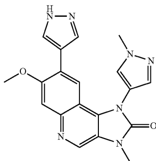
7-Methoxy-3-methyl-1-(1-methyl-1H-pyrazol-4-yl)-8-(1H-pyrazol-4-yl)-1,3-dihydroimidazo[4,5-c]quinolin-2-one
