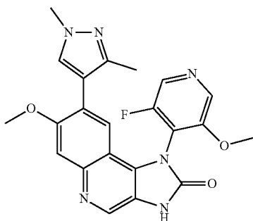
8-(1,3-Dimethyl-1H-pyrazol-4-yl)-1-(3-fluoro-5-methoxy-pyridin-4-yl)-7-methoxy-1,3-dihydroimidazo[4,5-c]quinolin-2-one
