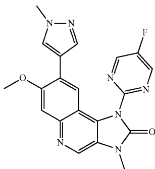
1-(5-Fluoropyrimidin-2-yl)-7-methoxy-3-methyl-8-(1-methyl-1H-pyrazol-4-yl)-1,3-dihydroimidazo[4,5-c]quinolin-2-one
