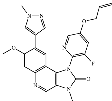
1-(5-Allyloxy-3-fluoropyridin-2-yl)-7-methoxy-3-methyl-8-(1-methyl-1H-pyrazol-4-yl)-1,3-dihydroimidazo[4,5-c]quinolin-2-one
