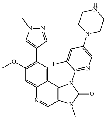
1-(3-Fluoro-5-piperazin-1-ylpyridin-2-yl)-7-methoxy-3-methyl-8-(1-methyl-1H-pyrazol-4-yl)-1,3-dihydroimidazo[4,5-c]quinolin-2-one
