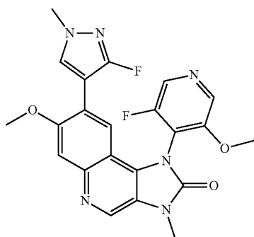
1-(3-Fluoro-5-methoxypyridin-4-yl)-7-methoxy-3-methyl-8-(3-fluoro-1-methyl-1H-pyrazol-4-yl)-1,3-dihydroimidazo[4,5-c]quinolin-2-one
