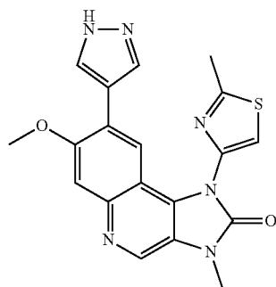
7-Methoxy-3-methyl-1-(2-methylthiazol-4-yl)-8-(1H-pyrazol-4-yl)-1,3-dihydroimidazo[4,5-c]quinolin-2-one
