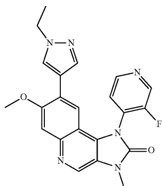
8-(1-Ethyl-1H-pyrazol-4-yl)-1-(3-fluoropyridin-4-yl)-7-methoxy-3-methyl-1,3-dihydroimidazo[4,5-c]quinolin-2-one
