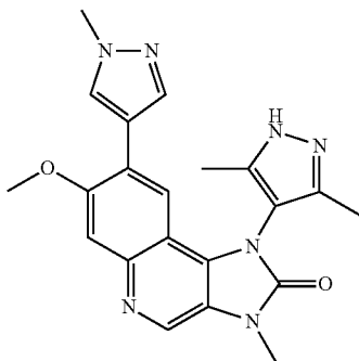
1-(3,5-Dimethyl-1H-pyrazol-4-yl)-7-methoxy-3-methyl-8-(1-methyl-1H-pyrazol-4-yl)-1,3-dihydroimidazo[4,5-c]quinolin-2-one
