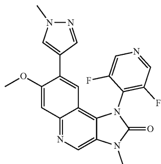
1-(3,5-Difluoropyridin-4-yl)-7-methoxy-3-methyl-8-(1-methyl-1H-pyrazol-4-yl)-1,3-dihydroimidazo[4,5-c]quinolin-2-one
