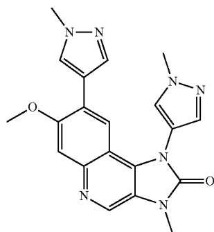
7-Methoxy-3-methyl-1,8-bis(1-methyl-1H-pyrazol-4-yl)-1,3-dihydroimidazo[4,5-c]quinolin-2-one
