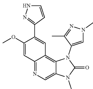
1-(1,3-Dimethyl-1H-pyrazol-4-yl)-7-methoxy-3-methyl-8-(1H-pyrazol-3-yl)-1,3-dihydroimidazo[4,5-c]quinolin-2-one
