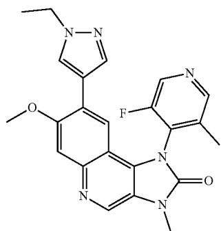
8-(1-Ethyl-1H-pyrazol-4-yl)-1-(3-fluoro-5-methylpyridin-4-yl)-7-methoxy-3-methyl-1,3-dihydroimidazo[4,5-c]quinolin-2-one
