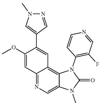
1-(3-Fluoropyridin-4-yl)-7-methoxy-3-methyl-8-(1-methyl-1H-pyrazol-4-yl)-1,3-dihydroimidazo[4,5-c]quinolin-2-one
