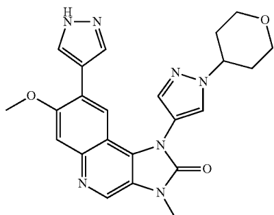
7-Methoxy-3-methyl-8-(1H-pyrazol-4-yl)-1-[1-(tetrahydropyran-4-yl)-1H-pyrazol-4-yl]-1,3-dihydroimidazo[4,5-c]quinolin-2-one
