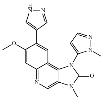
7-Methoxy-3-methyl-1-(2-methyl-2H-pyrazol-3-yl)-8-(1H-pyrazol-4-yl)-1,3-dihydroimidazo[4,5-c]quinolin-2-one
