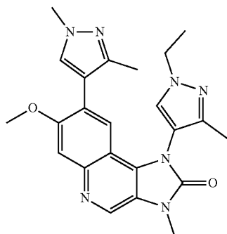
8-(1,3-Dimethyl-1H-pyrazol-4-yl)-1-(1-ethyl-3-methyl-1H-pyrazol-4-yl)-7-methoxy-3-methyl-1,3-dihydroimidazo[4,5-c]quinolin-2-one
