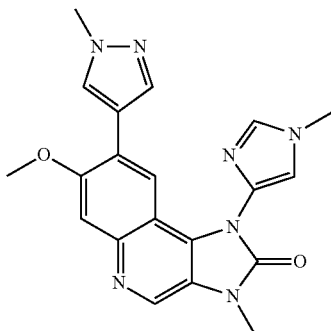
7-Methoxy-3-methyl-1-(1-methyl-1H-imidazol-4-yl)-8-(1-methyl-1H-pyrazol-4-yl)-1,3-dihydroimidazo[4,5-c]quinolin-2-one
