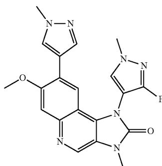
1-(3-Fluoro-1-methyl-1H-pyrazol-4-yl)-7-methoxy-3-methyl-8-(1-methyl-1H-pyrazol-4-yl)-1,3-dihydroimidazo[4,5-c]quinolin-2-one
