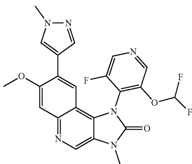
1-(3-Difluoromethoxy-5-fluoropyridin-4-yl)-7-methoxy-3-methyl-8-(1-methyl-1H-pyrazol-4-yl)-1,3-dihydroimidazo[4,5-c]quinolin-2-one
