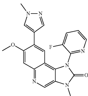
1-(3-Fluoropyridin-2-yl)-7-methoxy-3-methyl-8-(1-methyl-1H-pyrazol-4-yl)-1,3-dihydroimidazo[4,5-c]quinolin-2-one
