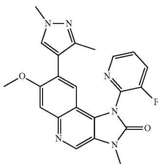
8-(1,3-Dimethyl-1H-pyrazol-4-yl)-1-(3-fluoropyridin-2-yl)-7-methoxy-3-methyl-1,3-dihydroimidazo[4,5-c]quinolin-2-one
