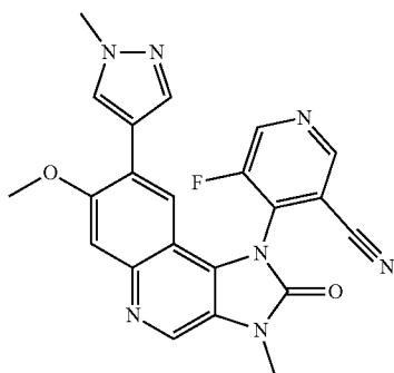
5-Fluoro-4-[7-methoxy-3-methyl-8-(1-methyl-1H-pyrazol-4-yl)-2-oxo-2,3-dihydroimidazo[4,5-c]quinolin-1-yl]nicotinonitrile
