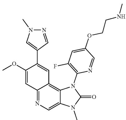
1-[3-Fluoro-5-(2-methylaminoethoxy)-pyridin-2-yl]-7-methoxy-3-methyl-8-(1-methyl-1H-pyrazol-4-yl)-1,3-dihydroimidazo[4,5-c]quinolin-2-one
