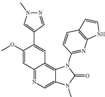
7-Methoxy-3-methyl-8-(1-methyl-1H-pyrazol-4-yl)-1-(1H-pyrrolo[2,3-b]pyridin-6-yl)-1,3-dihydroimidazo[4,5-c]quinolin-2-one
