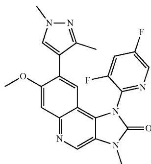
1-(3,5-Difluoropyridin-2-yl)-8-(1,3-dimethyl-1H-pyrazol-4-yl)-7-methoxy-3-methyl-1,3-dihydroimidazo[4,5-c]quinolin-2-one
