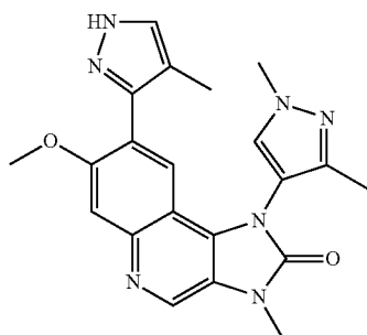
1-(1,3-Dimethyl-1H-pyrazol-4-yl)-7-methoxy-3-methyl-8-(4-methyl-1H-pyrazol-3-yl)-1,3-dihydroimidazo[4,5-c]quinolin-2-one
