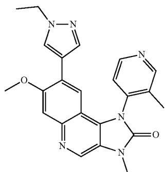
8-(1-Ethyl-1H-pyrazol-4-yl)-7-methoxy-3-methyl-1-(3-methylpyridin-4-yl)-1,3-dihydroimidazo[4,5-c]quinolin-2-one
