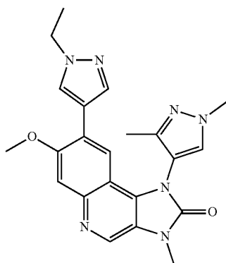
1-(1,3-Dimethyl-1H-pyrazol-4-yl)-8-(1-ethyl-1H-pyrazol-4-yl)-7-methoxy-3-methyl-1,3-dihydroimidazo[4,5-c]quinolin-2-one
