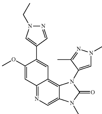
1-(1,3-Dimethyl-1H-pyrazol-4-yl)-8-(1-ethyl-1H-pyrazol-4-yl)-7-methoxy-3-methyl-1,3-dihydroimidazo[4,5-c]quinolin-2-one
