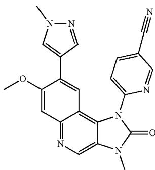
6-[7-Methoxy-3-methyl-8-(1-methyl-1H-pyrazol-4-yl)-2-oxo-2,3-dihydroimidazo[4,5-c]quinolin-1-yl]nicotinonitrile
