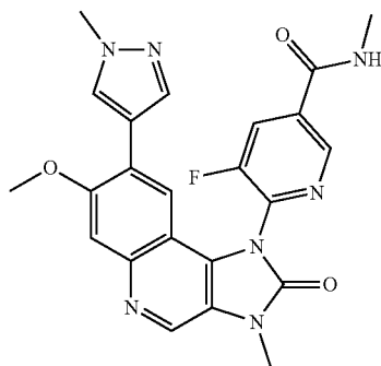
5-Fluoro-6-[7-methoxy-3-methyl-8-(1-methyl-1H-pyrazol-4-yl)-2-oxo-2,3-dihydroimidazo[4,5-c]quinolin-1-yl]-N-methylnicotinamide
