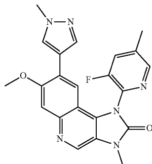
1-(3-Fluoro-5-methylpyridin-2-yl)-7-methoxy-3-methyl-8-(1-methyl-1H-pyrazol-4-yl)-1,3-dihydroimidazo[4,5-c]quinolin-2-one
