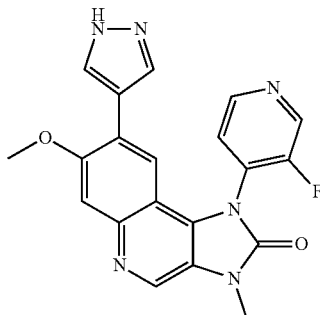
1-(3-Fluoropyridin-4-yl)-7-methoxy-3-methyl-8-(1H-pyrazol-4-yl)-1,3-dihydroimidazo[4,5-c]quinolin-2-one
