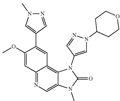
7-Methoxy-3-methyl-8-(1-methyl-1H-pyrazol-4-yl)-1-[1-(tetrahydropyran-4-yl)-1H-pyrazol-4-yl]-1,3-dihydroimidazo[4,5-c]quinolin-2-one
