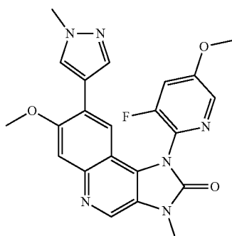
1-(3-Fluoro-5-methoxypyridin-2-yl)-7-methoxy-3-methyl-8-(1-methyl-1H-pyrazol-4-yl)-1,3-dihydroimidazo[4,5-c]quinolin-2-one
