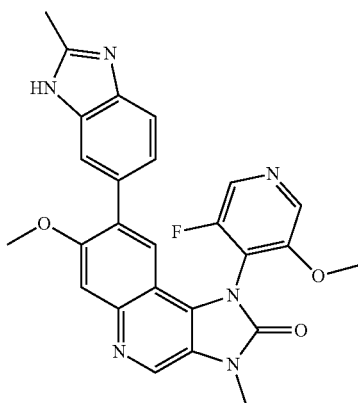
1-(3-Fluoro-5-methoxypyridin-4-yl)-7-methoxy-3-methyl-8-(2-methyl-3H-benzimidazol-5-yl)-1,3-dihydroimidazo[4,5-c]quinolin-2-one
