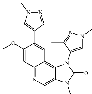
1-(1,3-Dimethyl-1H-pyrazol-4-yl)-7-methoxy-3-methyl-8-(1-methyl-1H-pyrazol-4-yl)-1,3-dihydroimidazo[4,5-c]quinolin-2-one
