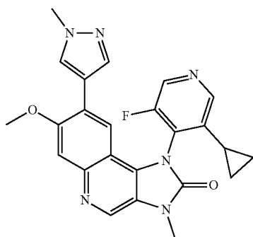
1-(3-Cyclopropyl-5-fluoropyridin-4-yl)-7-methoxy-3-methyl-8-(1-methyl-1H-pyrazol-4-yl)-1,3-dihydroimidazo[4,5-c]quinolin-2-one
