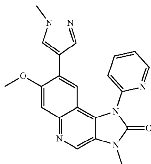
7-Methoxy-3-methyl-8-(1-methyl-1H-pyrazol-4-yl)-1-pyridin-2-yl-1,3-dihydroimidazo[4,5-c]quinolin-2-one
