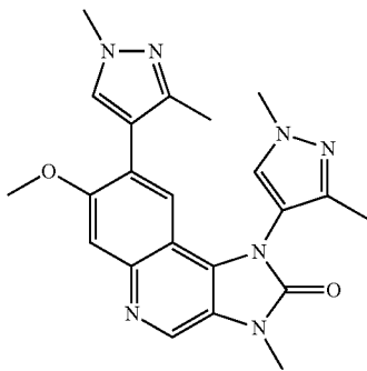
1,8-Bis-(1,3-dimethyl-1H-pyrazol-4-yl)-7-methoxy-3-methyl-1,3-dihydroimidazo[4,5-c]quinolin-2-one
