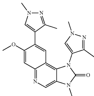
1,8-Bis(1,3-dimethyl-1H-pyrazol-4-yl)-7-methoxy-3-methyl-1,3-dihydroimidazo[4,5-c]quinolin-2-one
