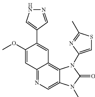
7-Methoxy-3-methyl-1-(2-methylthiazol-4-yl)-8-(1H-pyrazol-4-yl)-1,3-dihydroimidazo[4,5-c]quinolin-2-one
