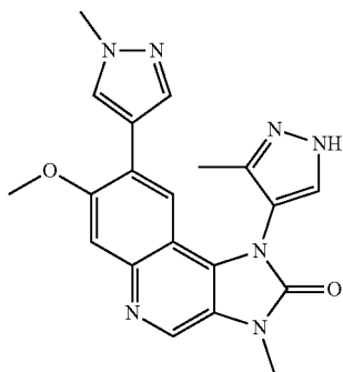
7-Methoxy-3-methyl-1-(3-methyl-1H-pyrazol-4-yl)-8-(1-methyl-1H-pyrazol-4-yl)-1,3-dihydroimidazo[4,5-c]quinolin-2-one
