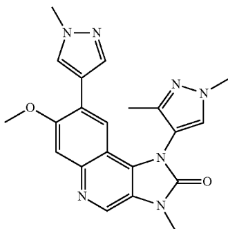
1-(1,3-Dimethyl-1H-pyrazol-4-yl)-7-methoxy-3-methyl-8-(1-methyl-1H-pyrazol-4-yl)-1,3-dihydroimidazo[4,5-c]quinolin-2-one
