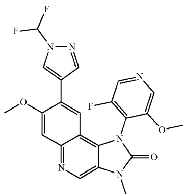
8-(1-Difluoromethyl-1H-pyrazol-4-yl)-1-(3-fluoro-5-methoxypyridin-4-yl)-7-methoxy-3-methyl-1,3-dihydroimidazo[4,5-c]quinolin-2-one
