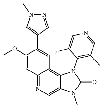
1-(3-Fluoro-5-methylpyridin-4-yl)-7-methoxy-3-methyl-8-(1-methyl-1H-pyrazol-4-yl)-1,3-dihydroimidazo[4,5-c]quinolin-2-one
