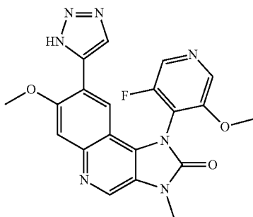
1-(3-Fluoro-5-methoxypyridin-4-yl)-7-methoxy-3-methyl-8-(3H-1,2,3-triazol-4-yl)-1,3-dihydroimidazo[4,5-c]quinolin-2-one
