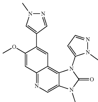
7-Methoxy-3-methyl-1-(2-methyl-2H-pyrazol-3-yl)-8-(1-methyl-1H-pyrazol-4-yl)-1,3-dihydroimidazo[4,5-c]quinolin-2-one
