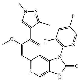
1-(3,5-Difluoropyridin-2-yl)-8-(1,3-dimethyl-1H-pyrazol-4-yl)-7-methoxy-1,3-dihydroimidazo[4,5-c]quinolin-2-one
