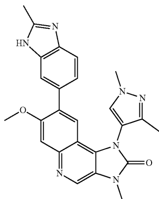
1-(1,3-Dimethyl-1H-pyrazol-4-yl)-7-methoxy-3-methyl-8-(2-methyl-3H-benzimidazol-5-yl)-1,3-dihydroimidazo[4,5-c]quinolin-2-one
