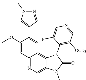
1-[3-Fluoro-5-(trideuteriomethoxy)-4-pyridyl]-7-methoxy-3-methyl-8-(1-methylpyrazol-4-yl)imidazo[4,5-c]quinolin-2-one
