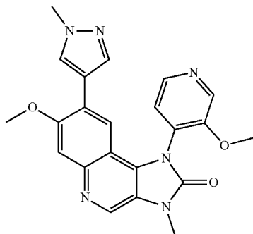
7-Methoxy-1-(3-methoxypyridin-4-yl)-3-methyl-8-(1-methyl-1H-pyrazol-4-yl)-1,3-dihydroimidazo[4,5-c]quinolin-2-one
