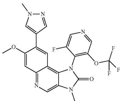
1-[3-Fluoro-5-(trifluoromethoxy)-4-pyridyl]-7-methoxy-3-methyl-8-(1-methyl-1H-pyrazol-4-yl)-1,3-dihydroimidazo[4,5-c]quinolin-2-one
