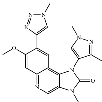
1-(1,3-Dimethyl-1H-pyrazol-4-yl)-7-methoxy-3-methyl-8-(1-methyl-1H-1,2,3-triazol-4-yl)-1,3-dihydroimidazo[4,5-c]quinolin-2-one
