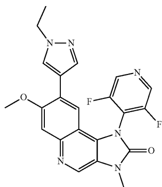
1-(3,5-Difluoropyridin-4-yl)-8-(1-ethyl-1H-pyrazol-4-yl)-7-methoxy-3-methyl-1,3-dihydroimidazo[4,5-c]quinolin-2-one
