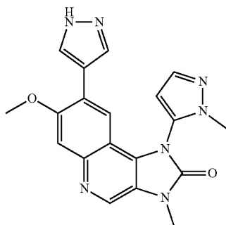
7-Methoxy-3-methyl-1-(2-methyl-2H-pyrazol-3-yl)-8-(1H-pyrazol-4-yl)-1,3-dihydroimidazo[4,5-c]quinolin-2-one
