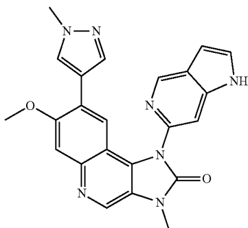
7-Methoxy-3-methyl-8-(1-methyl-1H-pyrazol-4-yl)-1-(1H-pyrrolo[3,2-c]pyridin-6-yl)-1,3-dihydroimidazo[4,5-c]quinolin-2-one
