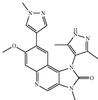
1-(3,5-Dimethyl-1H-pyrazol-4-yl)-7-methoxy-3-methyl-8-(1-methyl-1H-pyrazol-4-yl)-1,3-dihydroimidazo[4,5-c]quinolin-2-one
