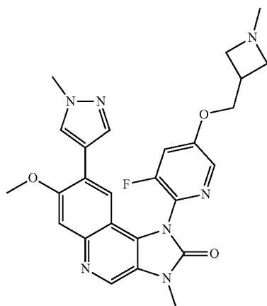
1-[3-Fluoro-5-(1-methylazetidin-3-ylmethoxy)pyridin-2-yl]-7-methoxy-3-methyl-8-(1-methyl-1H-pyrazol-4-yl)-1,3-dihydroimidazo[4,5-c]quinolin-2-one
