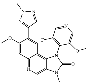
1-(3-Fluoro-5-methoxypyridin-4-yl)-7-methoxy-3-methyl-8-(2-methyl-2H-1,2,3-triazol-4-yl)-1,3-dihydroimidazo[4,5-c] quinolin-2-one
