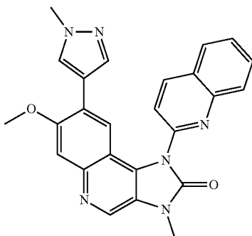
7-Methoxy-3-methyl-8-(1-methyl-1H-pyrazol-4-yl)-1-quinolin-2-yl-1,3-dihydroimidazo[4,5-c]quinolin-2-one
