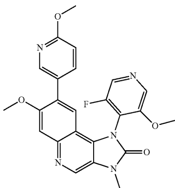
1-(3-Fluoro-5-methoxypyridin-4-yl)-7-methoxy-8-(6-methoxypyridin-3-yl)-3-methyl-1,3-dihydroimidazo[4,5-c]quinolin-2-one
