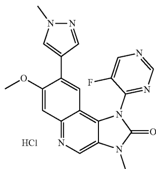
1-(5-Fluoropyrimidin-4-yl)-7-methoxy-3-methyl-8-(1-methyl-1H-pyrazol-4-yl)-1H,2H,3H-imidazo[4,5-c]quinolin-2-one hydrochloride
