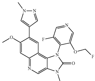
1-(3-Fluoro-5-fluoromethoxypyridin-4-yl)-7-methoxy-3-methyl-8-(1-methyl-1H-pyrazol-4-yl)-1,3-dihydroimidazo[4,5-c]quinolin-2-one
