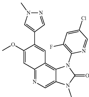
1-(5-Chloro-3-fluoropyridin-2-yl)-7-methoxy-3-methyl-8-(1-methyl-1H-pyrazol-4-yl)-1,3-dihydroimidazo[4,5-c]quinolin-2-one
