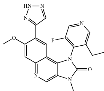
1-(3-Ethyl-5-fluoropyridin-4-yl)-7-methoxy-3-methyl-8-(2H-1,2,3-triazol-4-yl)-1,3-dihydroimidazo[4,5-c] quinolin-2-one
