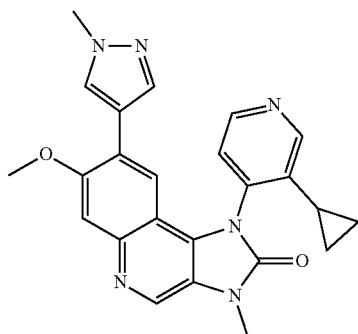
1-(3-Cyclopropylpyridin-4-yl)-7-methoxy-3-methyl-8-(1-methyl-1H-pyrazol-4-yl)-1,3-dihydroimidazo[4,5-c]quinolin-2-one
