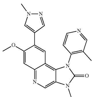
7-Methoxy-3-methyl-8-(1-methyl-1H-pyrazol-4-yl)-1-(3-methylpyridin-4-yl)-1,3-dihydroimidazo[4,5-c]quinolin-2-one
