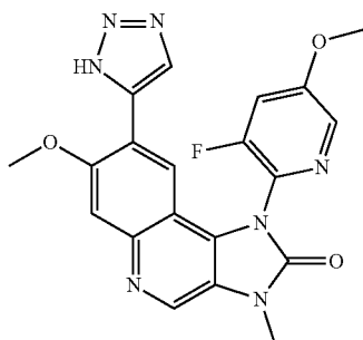
1-(3-Fluoro-5-methoxypyridin-2-yl)-7-methoxy-3-methyl-8-(3H-1,2,3-triazol-4-yl)-1,3-dihydroimidazo[4,5-c] quinolin-2-one
