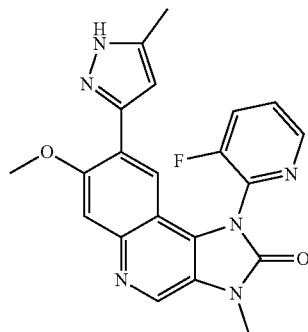
1-(3-Fluoropyridin-2-yl)-7-methoxy-3-methyl-8-(5-methyl-1H-pyrazol-3-yl)-1,3-dihydroimidazo[4,5-c]quinolin-2-one
