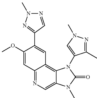
1-(1,3-Dimethyl-1H-pyrazol-4-yl)-7-methoxy-3-methyl-8-(2-methyl-2H-1,2,3-triazol-4-yl)-1,3-dihydroimidazo[4,5-c]quinolin-2-one
