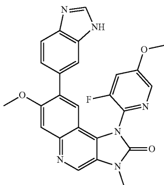
8-(3H-Benzimidazol-5-yl)-1-(3-fluoro-5-methoxypyridin-2-yl)-7-methoxy-3-methyl-1,3-dihydroimidazo[4,5-c]quinolin-2-one
