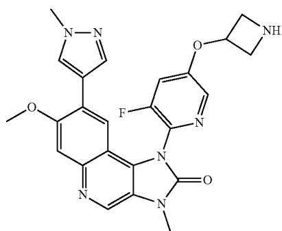
1-[5-(Azetidin-3-yloxy)-3-fluoropyridin-2-yl]-7-methoxy-3-methyl-8-(1-methyl-1H-pyrazol-4-yl)-1,3-dihydroimidazo[4,5-c]quinolin-2-one
