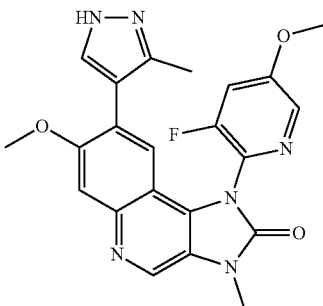
1-(3-Fluoro-5-methoxypyridin-2-yl)-7-methoxy-3-methyl-8-(3-methyl-1H-pyrazol-4-yl)-1,3-dihydroimidazo[4,5-c]quinolin-2-one
