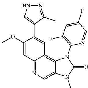
1-(3,5-Difluoropyridin-2-yl)-7-methoxy-3-methyl-8-(3-methyl-1H-pyrazol-4-yl)-1,3-dihydroimidazo[4,5-c]quinolin-2-one
