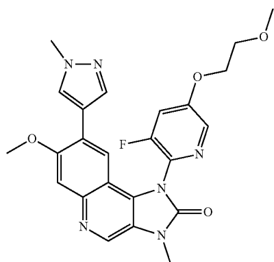
1-[3-Fluoro-5-(2-methoxyethoxy)-2-pyridyl]-7-methoxy-3-methyl-8-(1-methylpyrazol-4-yl)imidazo[4,5-c]quinolin-2-one
