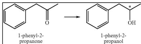
Reaction A: Bioconversion of 1-phenyl-2-propanone into 1-phenyl-2-propanol.
