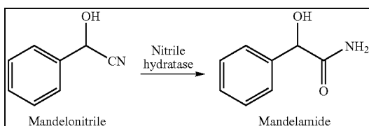
Reaction C: Bioconversion of mandelonitrile into mandelamide
