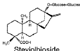
Steviolbioside
