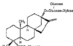
Rebaudioside F
