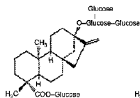
Rebaudioside A
