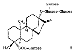
Rebaudioside A
