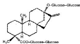
Rebaudioside E
