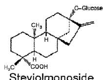
Steviolmonoside
