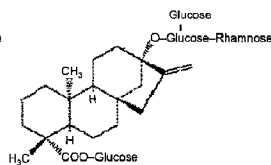
Rebaudioside C
