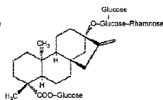
Rebaudioside C
