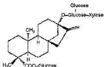
Rebaudioside F
