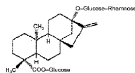
Dulcoside A
