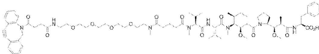
Figure 11B: DBCO-DM4
