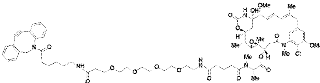
Figure 11B: DBCO-DM4
