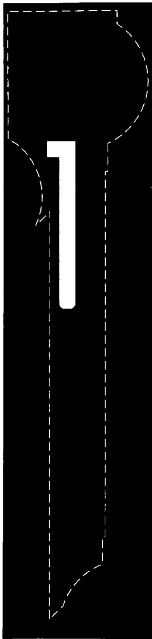
N-Well mask
