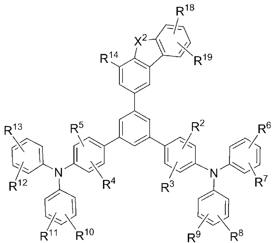
[Chemical Formula 6]
