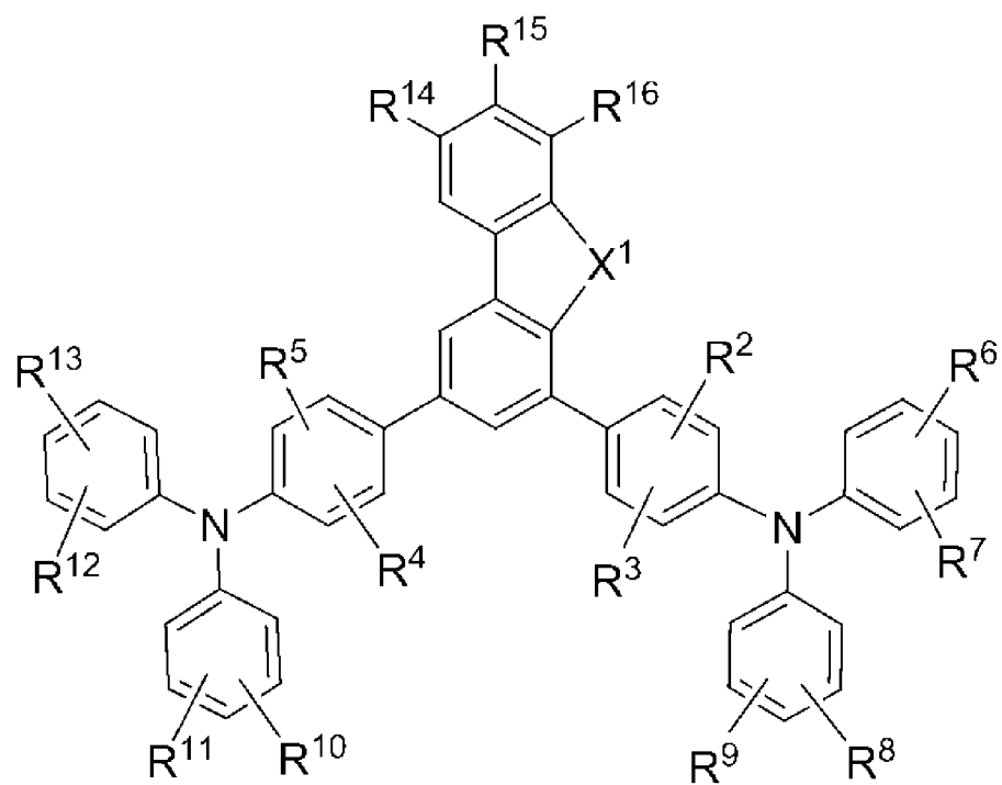
[Chemical Formula 5]
