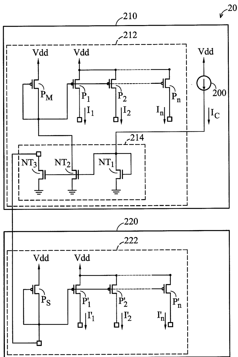
Fig. 2 ( Prior Art )
