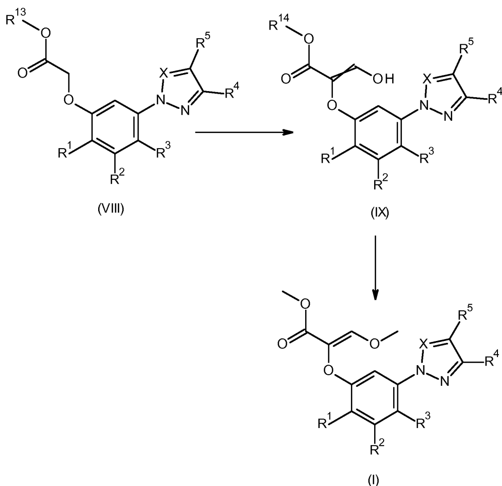
Scheme 6
