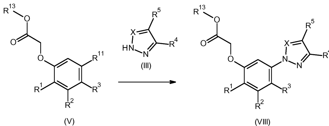
Scheme 7
