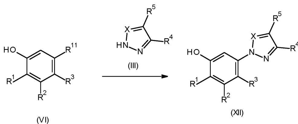
Scheme 12
