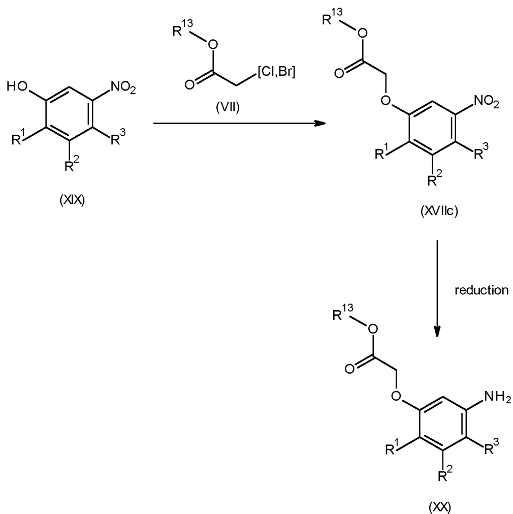
Scheme 16
