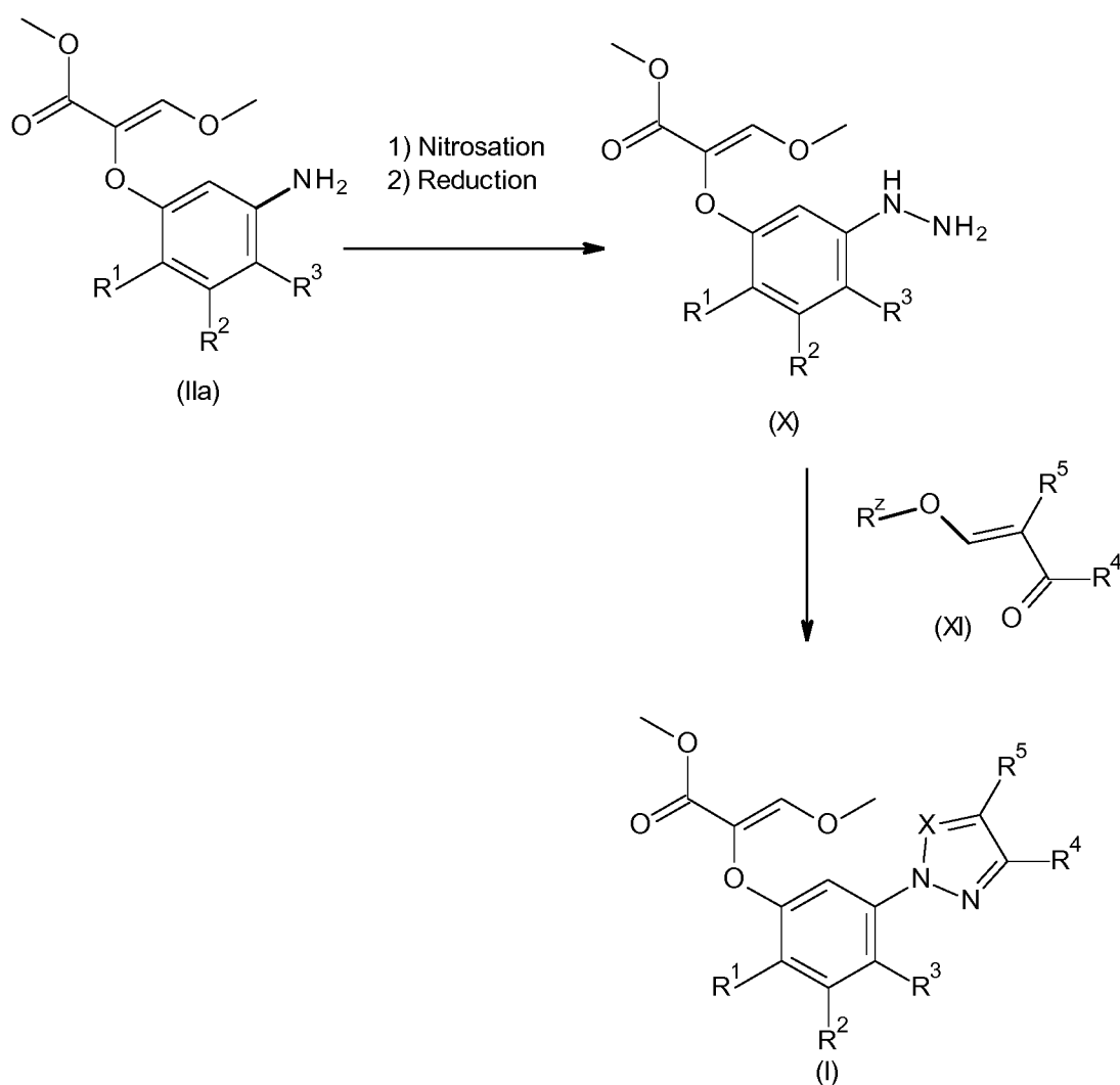
Scheme 9
