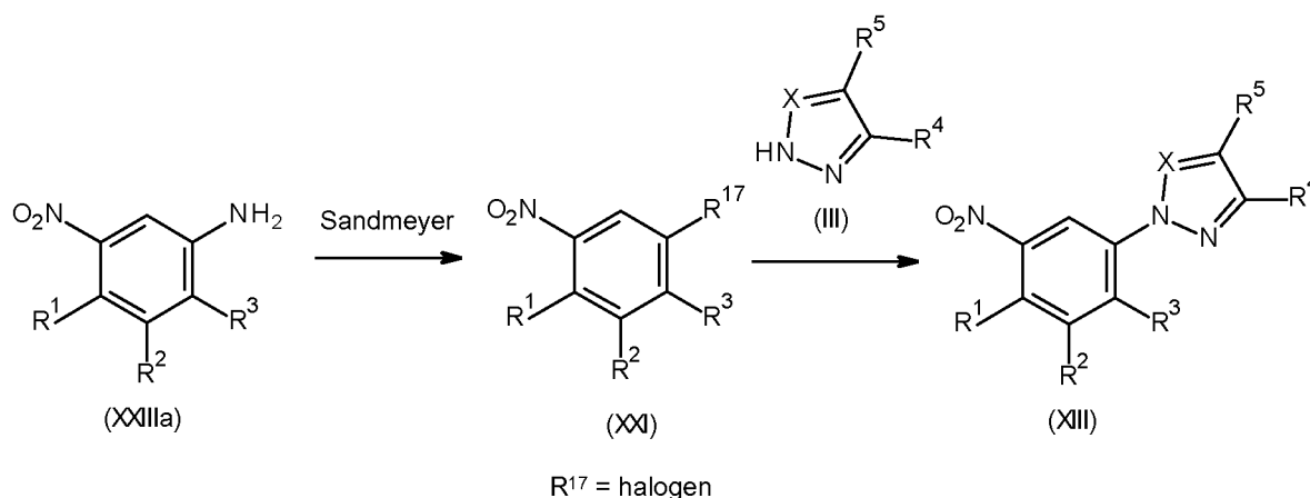
Scheme 20
