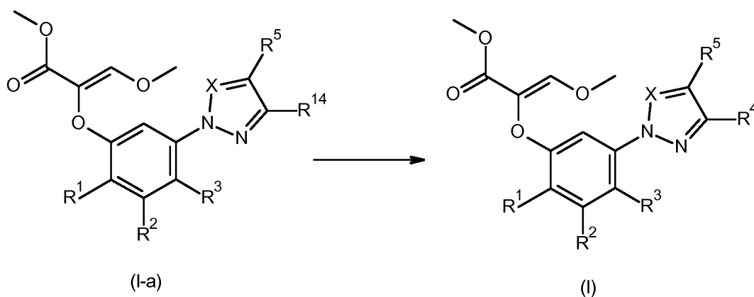
Scheme 8
