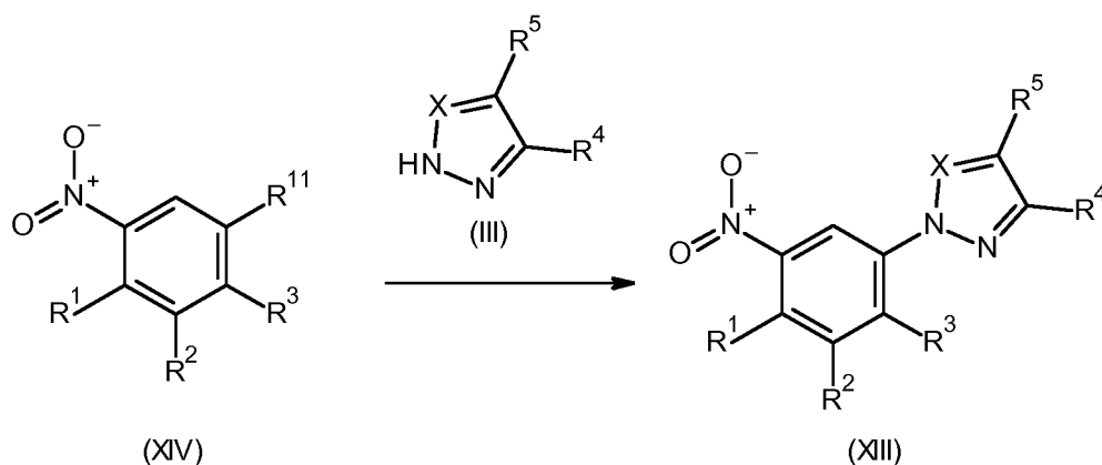
Scheme 11
