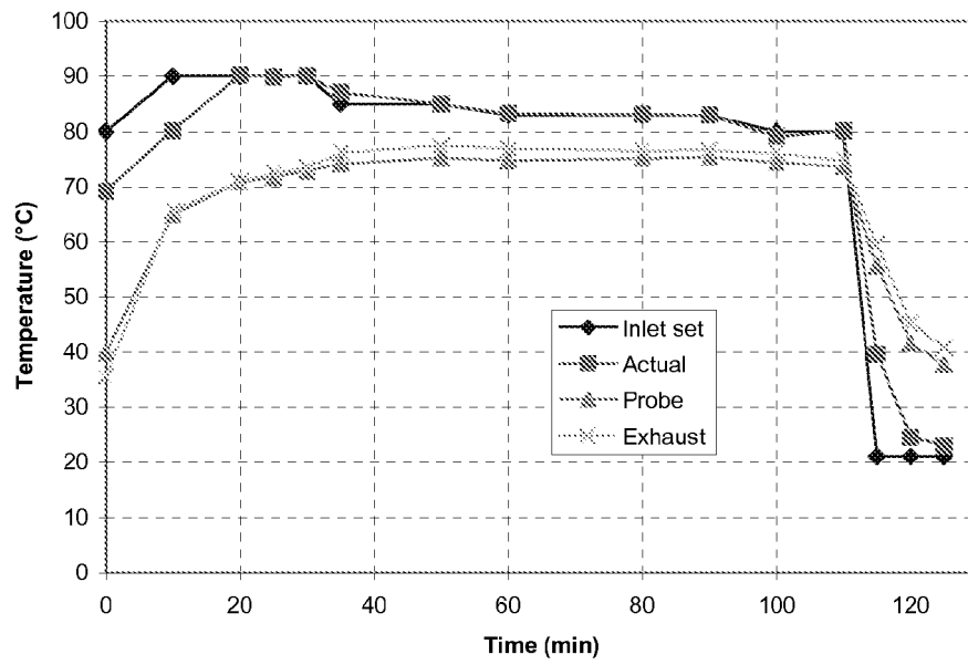
Curing of Example 13.5 Temperature Profile
