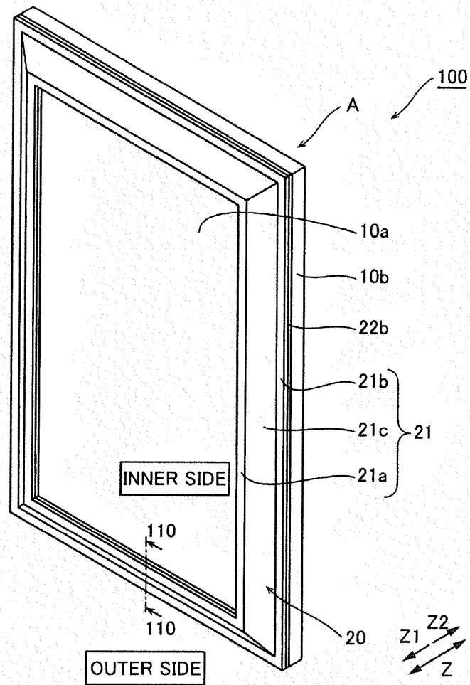
FIG. 1 FIRST EMBODIMENT
