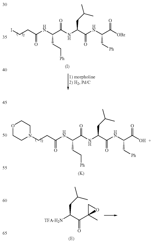
Scheme 5: Synthesis of Example 6
