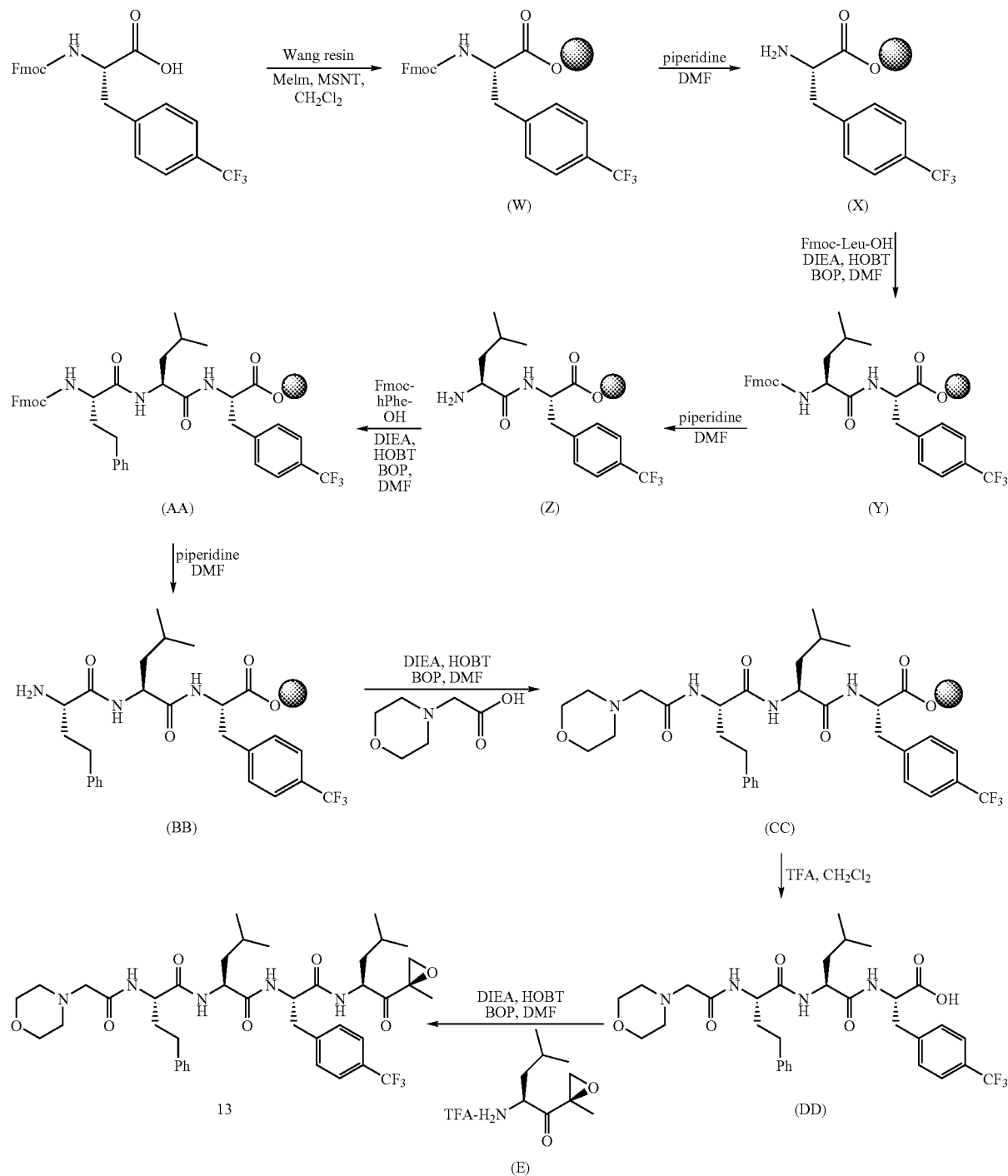
Scheme 10: Synthesis of Example 13
