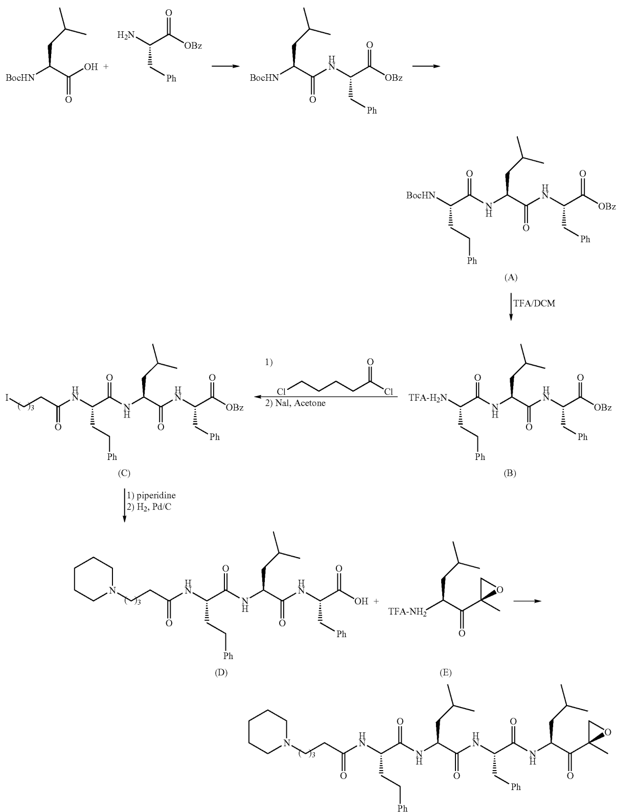
Scheme 1: Synthesis of Example 1
