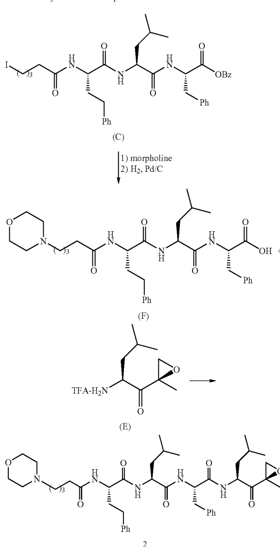
Scheme 2: Synthesis of Example 2
