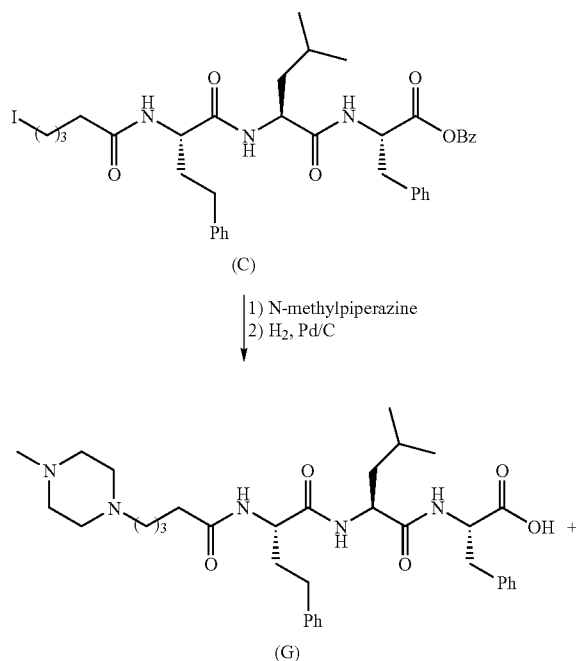
Scheme 3: Synthesis of Example 3
