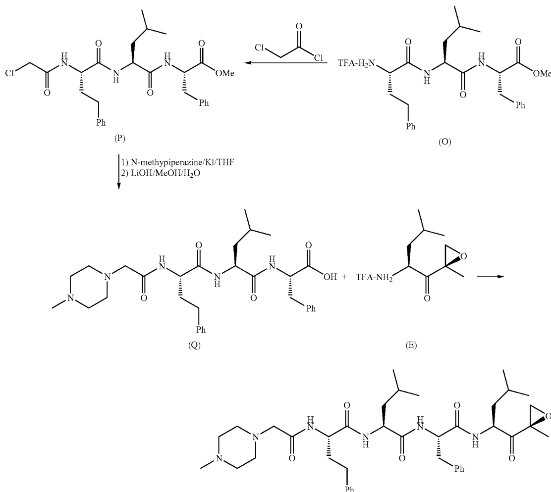
Scheme 8: Synthesis of Example 9
