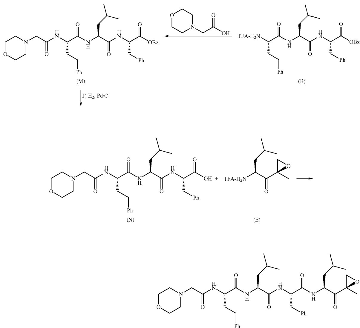
Scheme 7: Synthesis of Example 8
