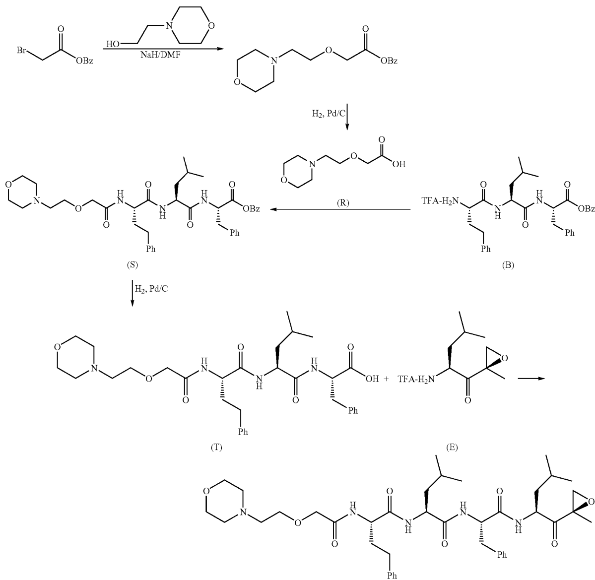
Scheme 9: Synthesis of Example 10
