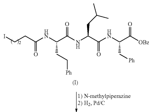
Scheme 6: Synthesis of Example 7
