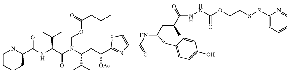
EC0312 C_{50}H_{72}N_8O_{11}S_3 Mol. Wt.: 1057.35
