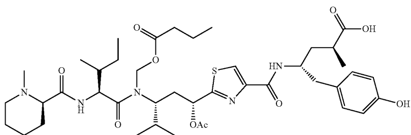
Tubulysin B C_{42}H_{63}N_5O_{10}S Mol. Wt.: 830.04
