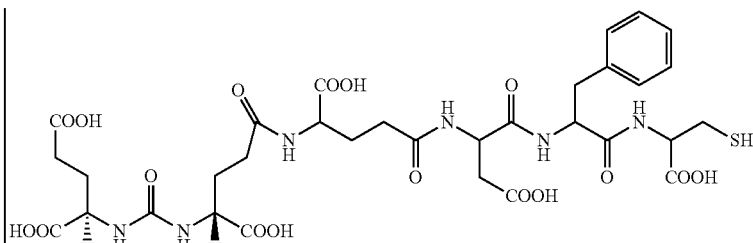
PC01SK68 C_{32}H_{42}N_6O_{17}S Mol. Wt.: 814.77
