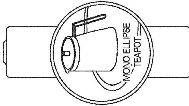
OBJECT RECOGNITION
