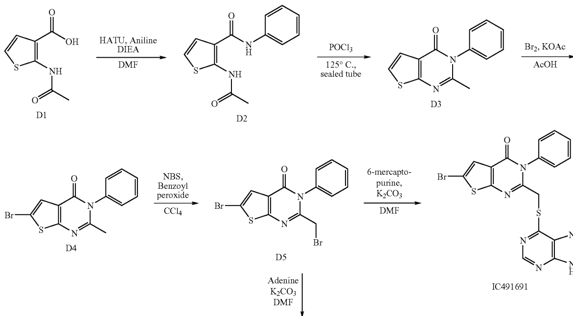
Scheme II. Preparation of Additional Compounds of the Invention.
