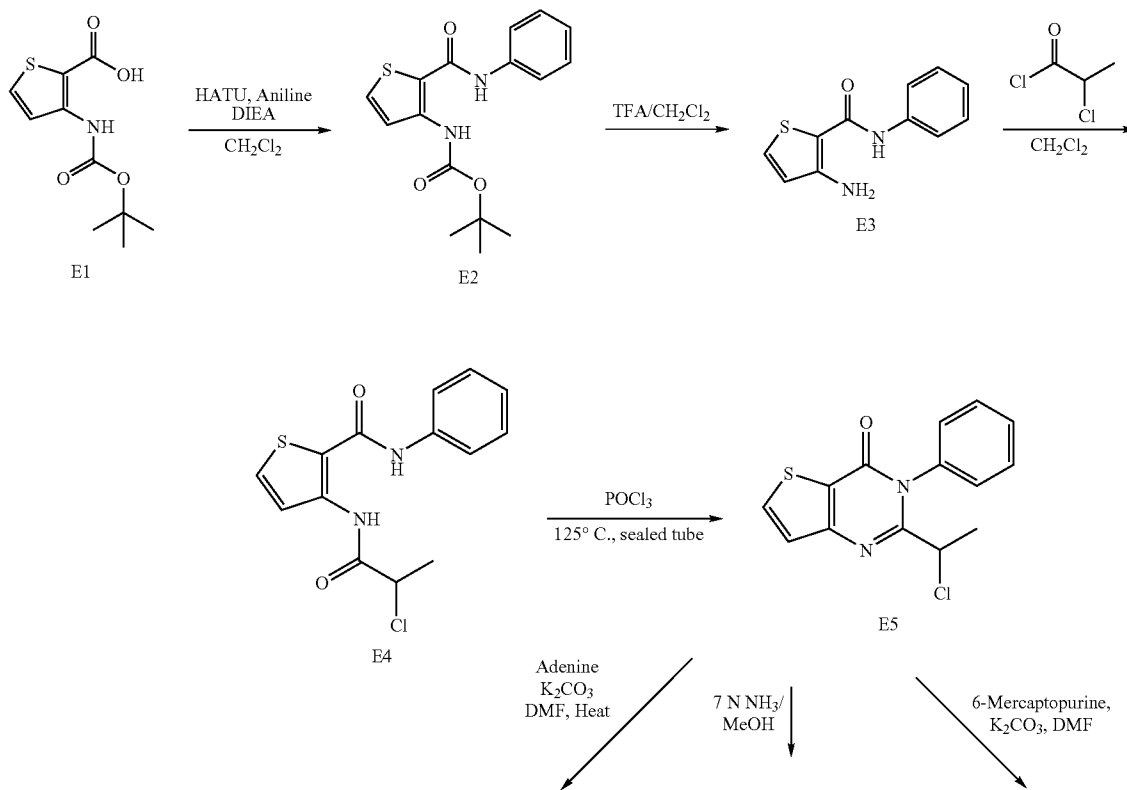
Scheme III. Preparation of Additional Compounds of the Invention.
