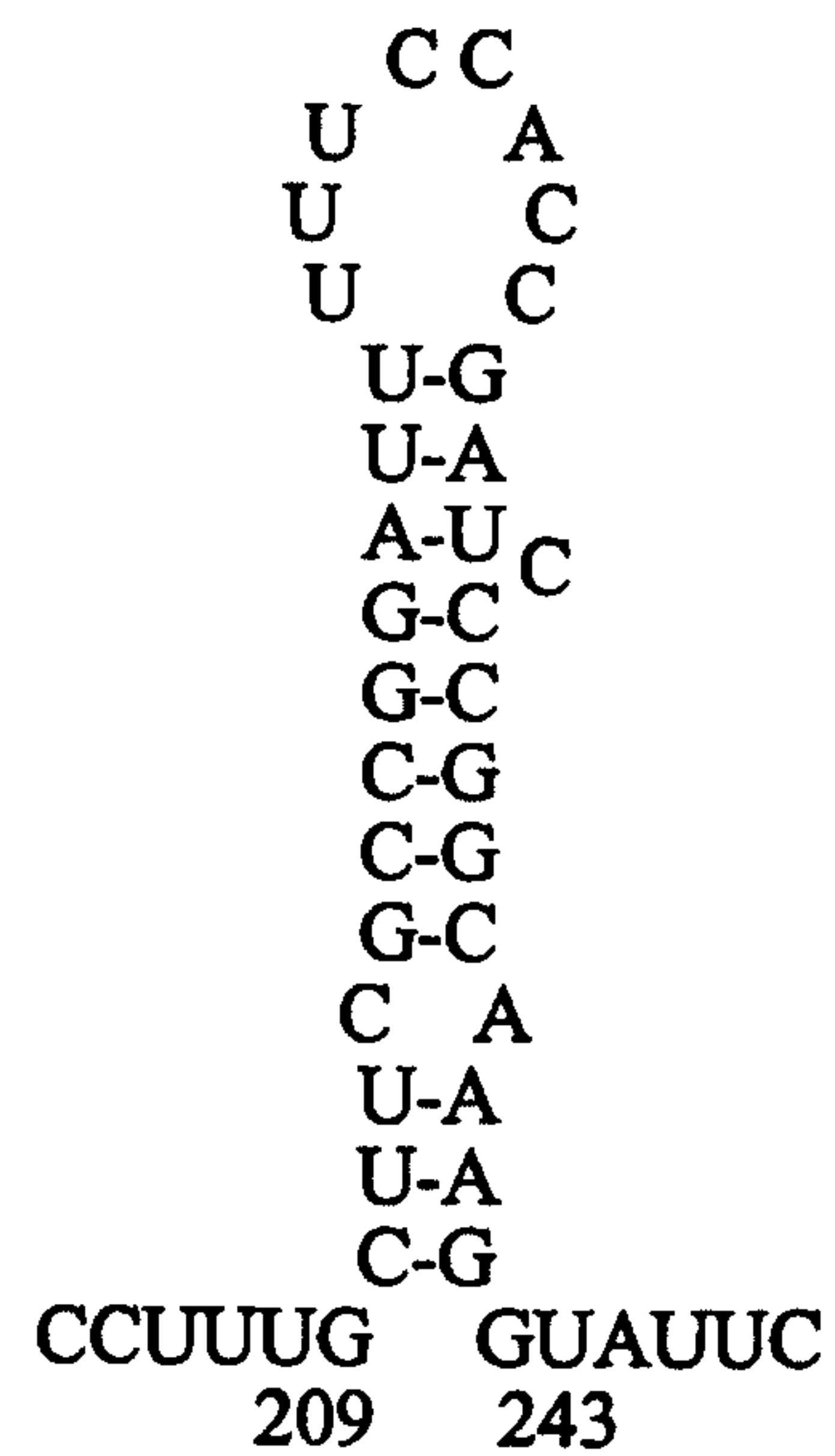
NOV RNA 2 Encapsidation Signal
