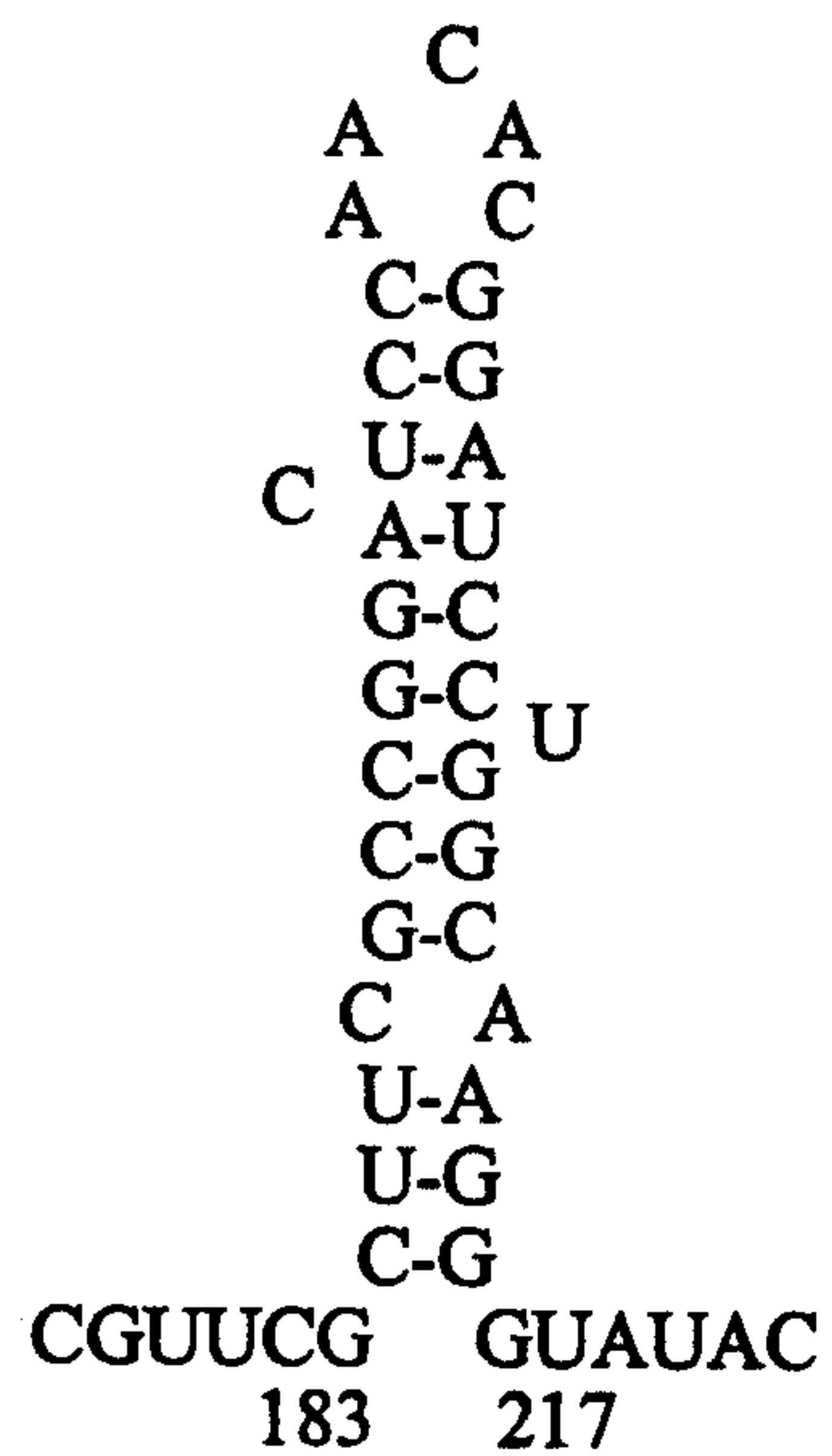
BOV RNA 2 Encapsidation Signal
