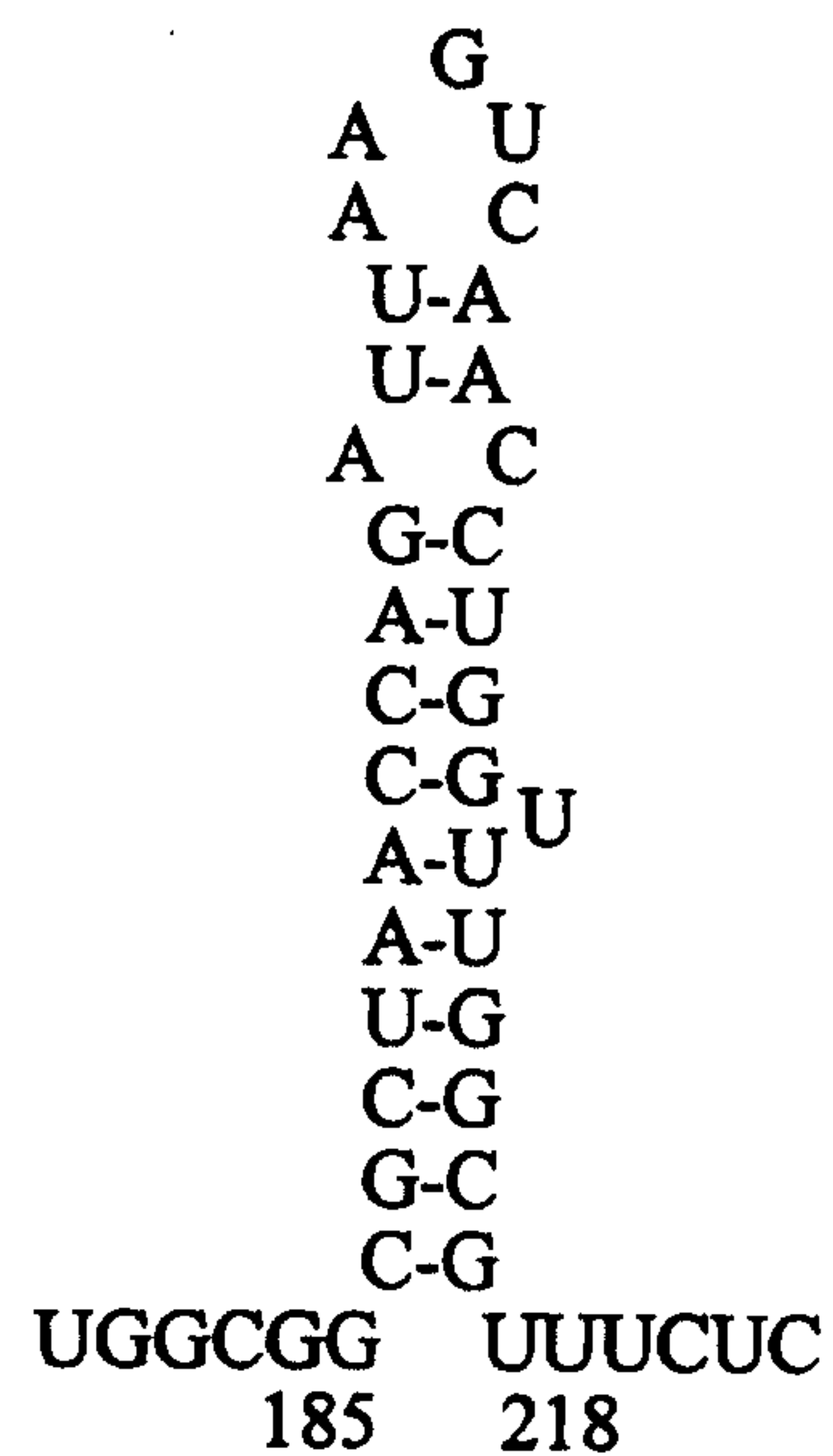
FHV RNA 2 Encapsidation Signal
