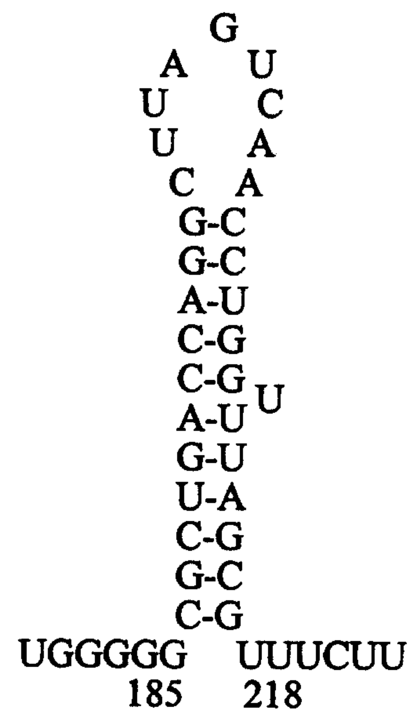
BBV RNA 2 Encapsidation Signal
