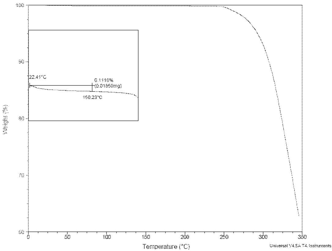
Fig. 7 TGA trace of Form 2
