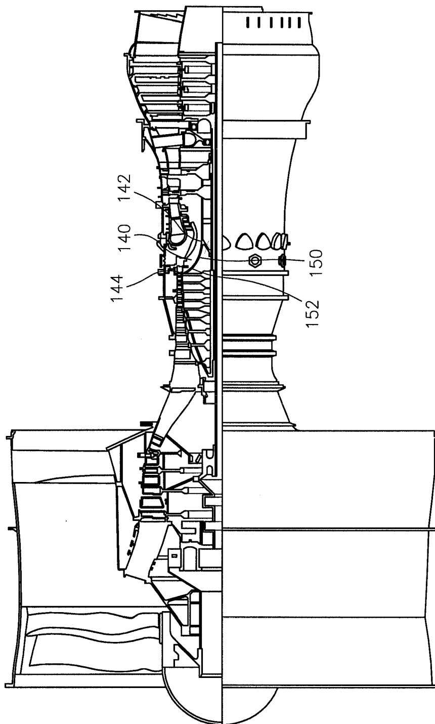
FIG. 4 (PRIOR ART)
