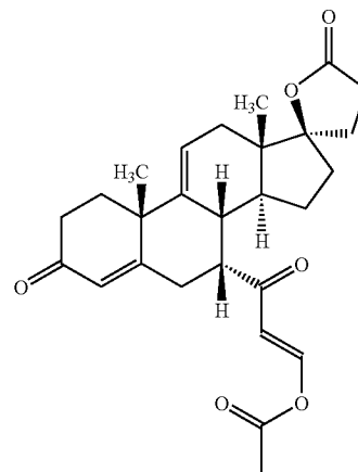
Trans-Enolacetate
