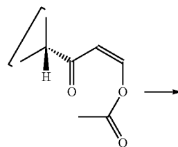
Cis-Enolacetate
