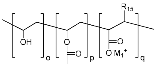
[Chemical Formula 9]
