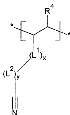
[Chemical Formula 4]
