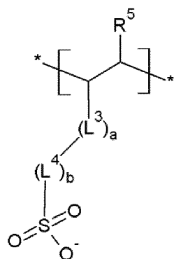
[Chemical Formula 5]
