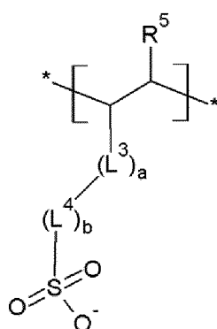
[Chemical Formula 5]
