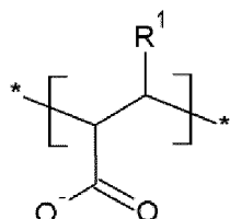
[Chemical Formula 1]
