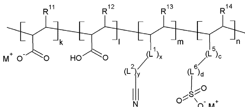
[Chemical Formula 8]
