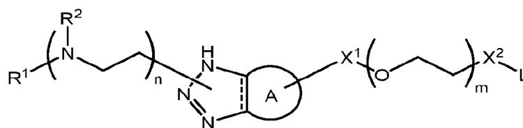
Formula I
