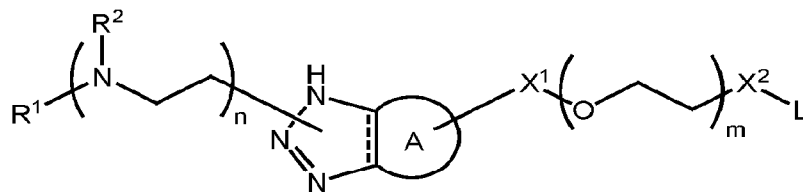
Formula I,
