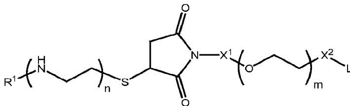
Formula IM,
