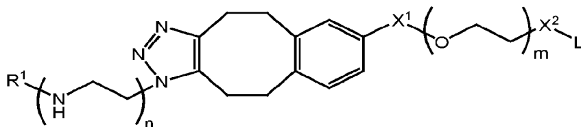
Formula IH-2,
