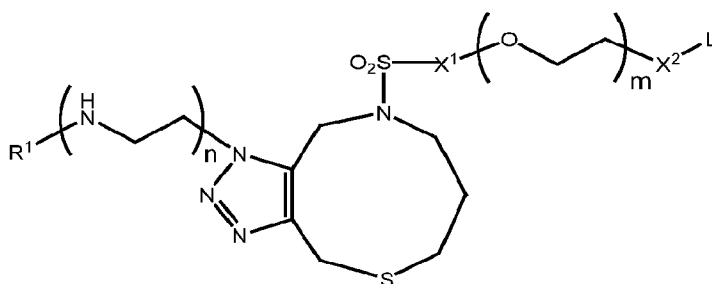
Formula IK-3,
