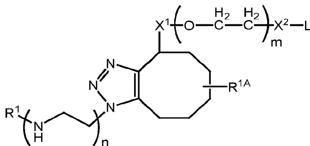
Formula IE-14,
