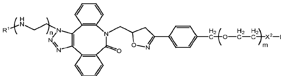
Formula IA-9a,
