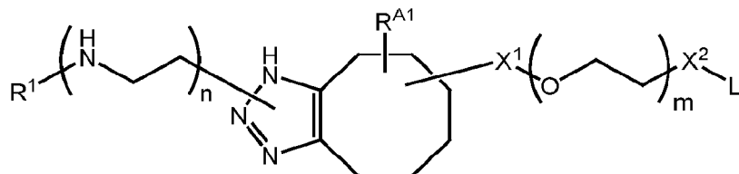
Formula IE,
