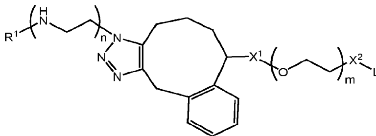
Formula II-1,
