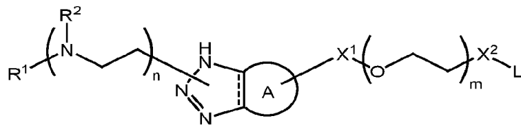
Formula I
