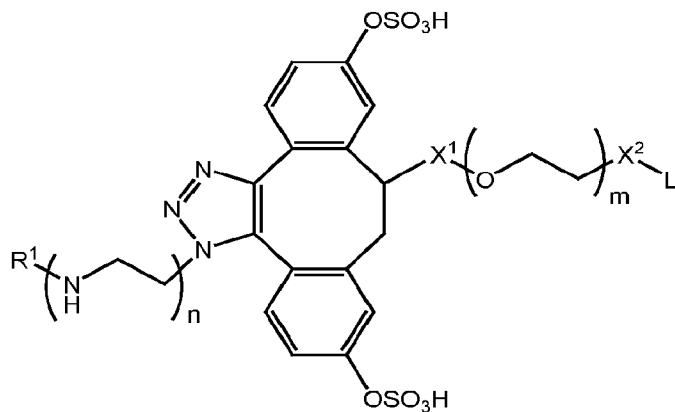
Formula IE-10,
