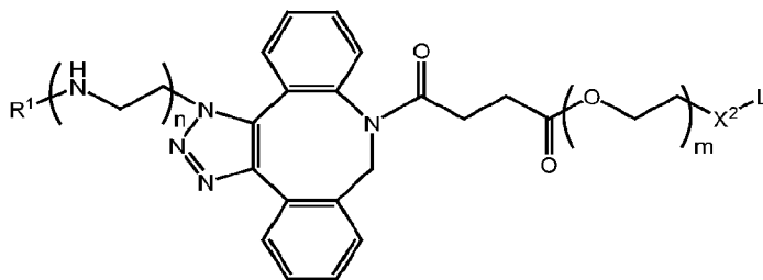
Formula IA-3a,
