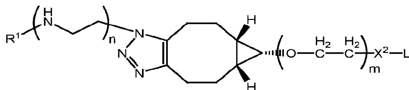
Formula IB-1a,
