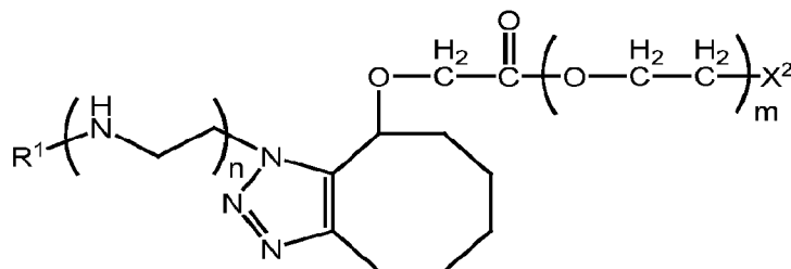
Formula IE-13a,
