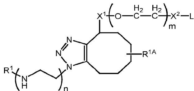
Formula IE-14,
