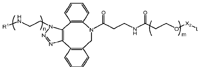
Formula IA-3c,
