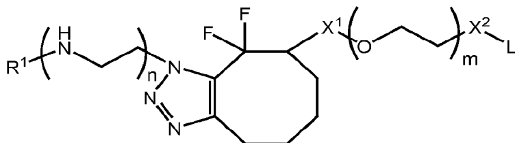
Formula IE-11,
