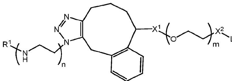
Formula IJ-2,
