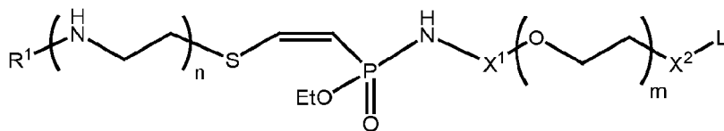
Formula IS,
