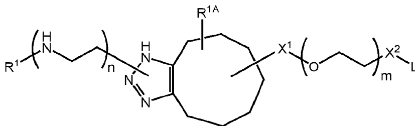
Formula II,
