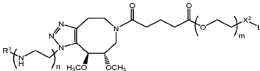
Formula IA-8a,
