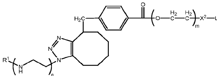
Formula IE-14c,
