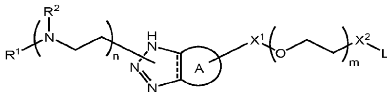
Formula I
