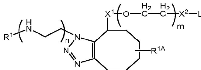
Formula IE-13,
