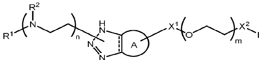
Formula I
