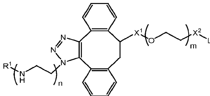
Formula IE-8,
