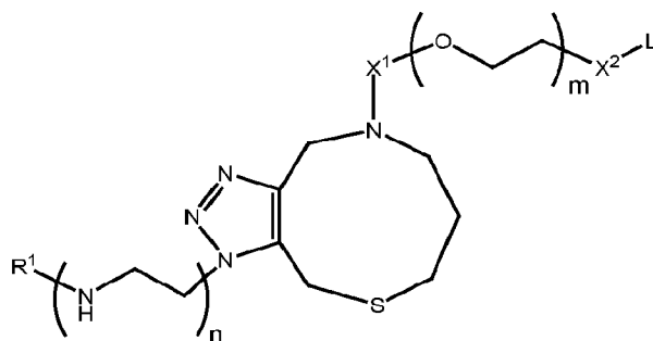
Formula IK-2,
