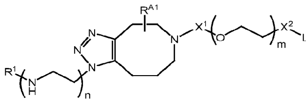
Formula IA-2,
