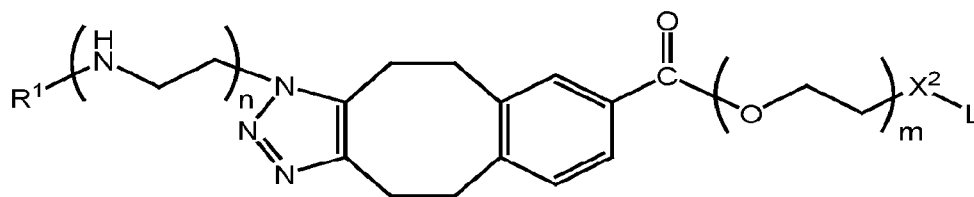
Formula IH-1a,
