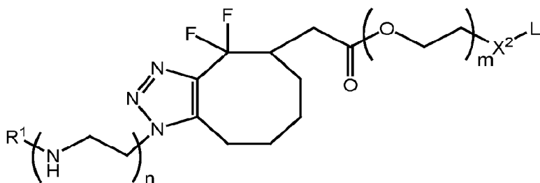
Formula IE-12a,
