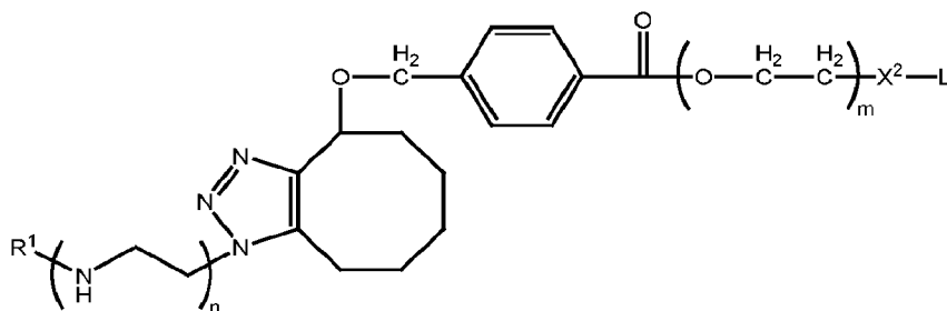
Formula IE-14b,
