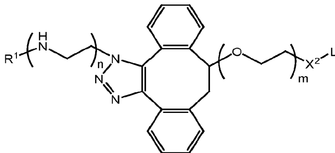
Formula IE-7a,
