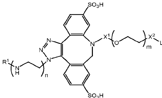
Formula IA-6,
