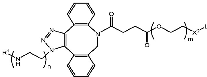
Formula IA-4a,
