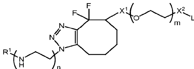
Formula IE-12,
