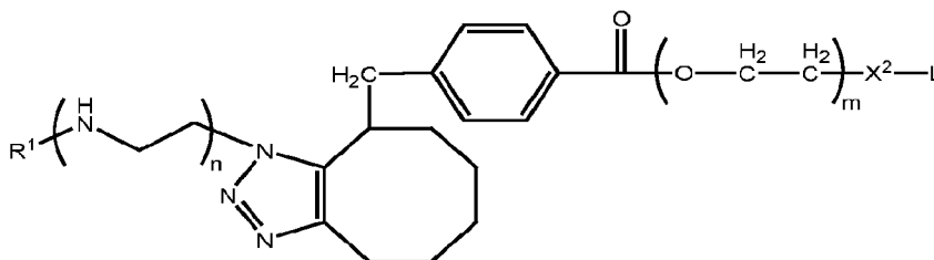
Formula IE-13c,
