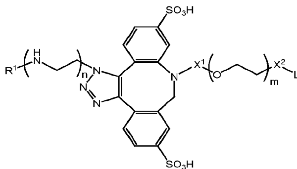
Formula IA-5,
