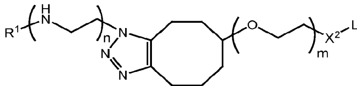
Formula IE-3a,
