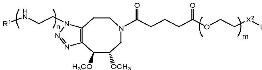
Formula IA-7a,
