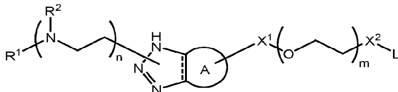
Formula I,
