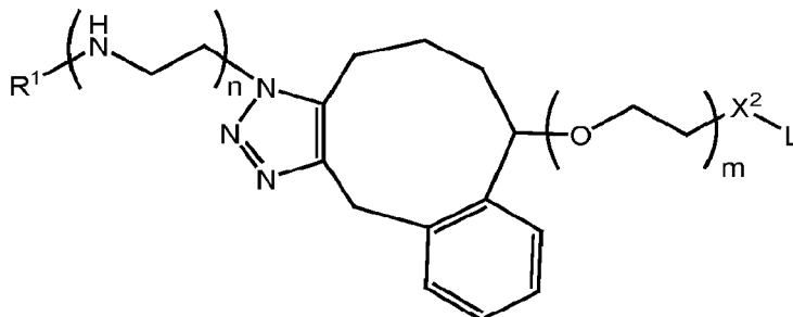
Formula IJ-1a,
