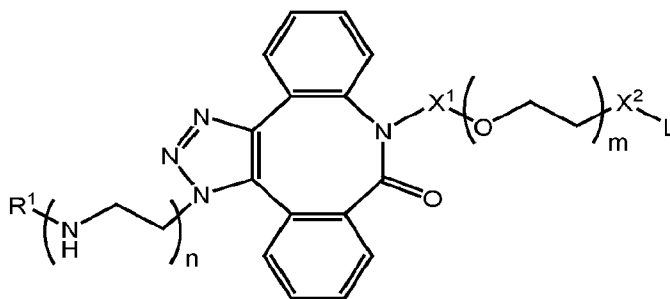
Formula IA-10,
