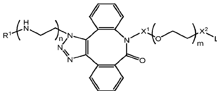
Formula IA-9,
