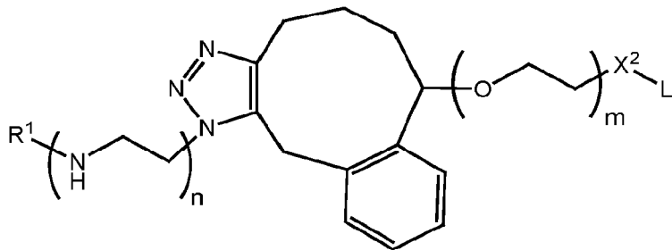
Formula IJ-2a,
