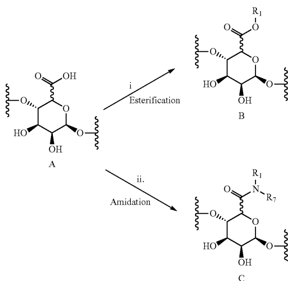
Scheme 1. Representative Reaction Conditions: i. HO—R 1 , 2-Chloro-4,6-dimethoxy-1,3,5-triazine (CDMT), N-methyl morpholine (NMM); ii. HNR 1 R 7 , CDMT, NMM.
