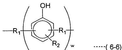
[Chemical formula 26]
