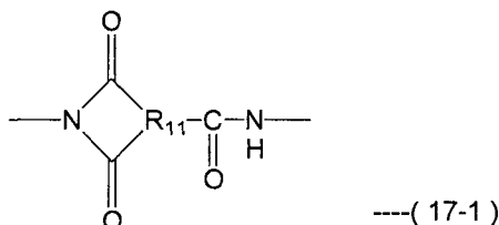
[Chemical formula 31]
