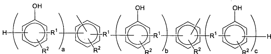
[Chemical formula 42]
