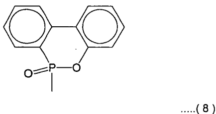
[Chemical formula 12]
