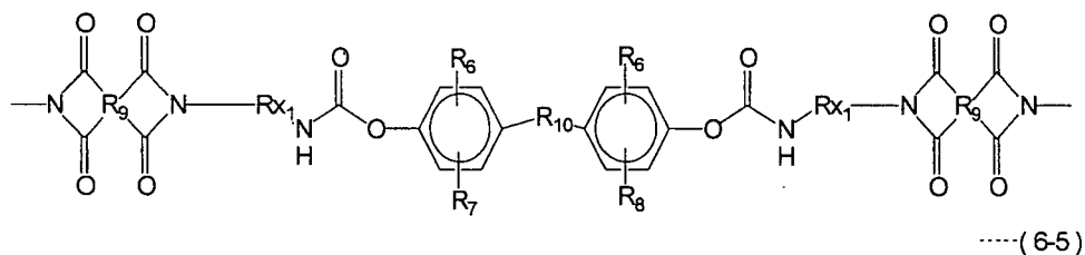
[Chemical formula 25]
