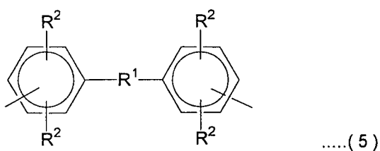
[Chemical formula 38]
