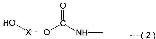
[Chemical formula 6]
