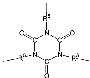
[Chemical formula 44]
