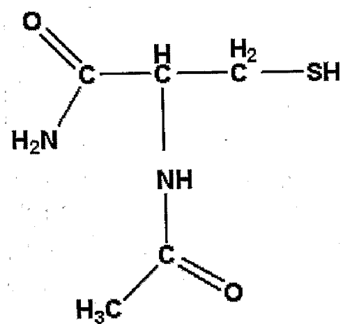
N-Acetylcysteine amide (AD4)
