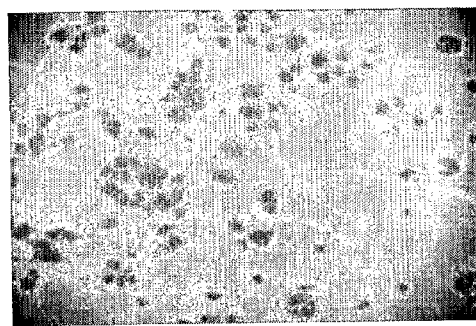
NACA only (750 \mu M)
