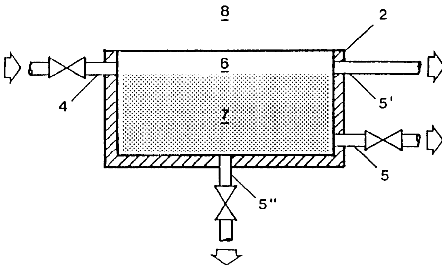
FIGURE 2 PRIOR ART
