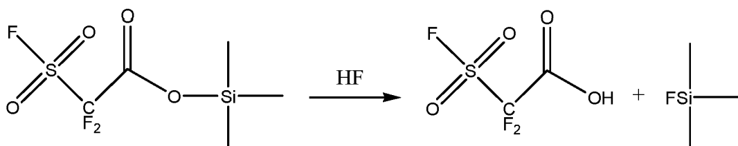
<Reaction formula (3)>
