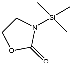
<Chemical formula 2 (1)>
