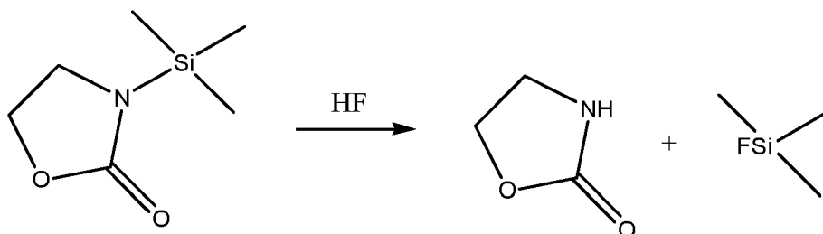
<Reaction formula (2)>
